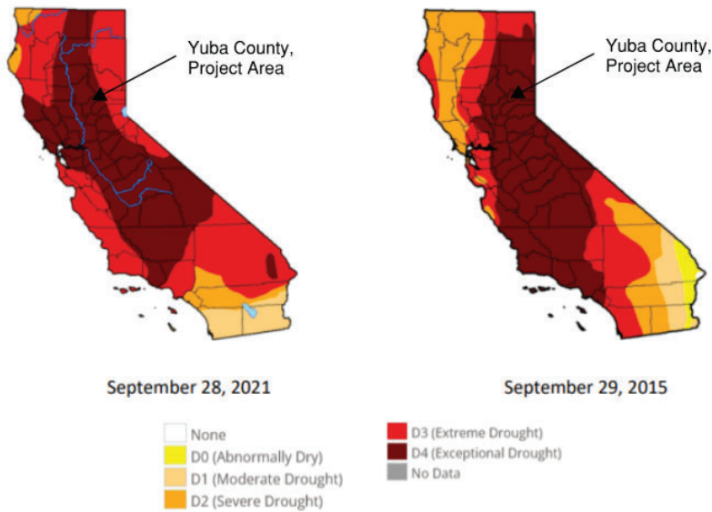
Figure 6: Drought Intensity in California Comparison of conditions at the end of the Water Year, 2021 vs. 2015
