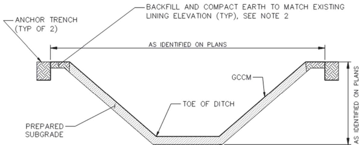
Figure 5. Cross Section of GCCM-lined Ditch
