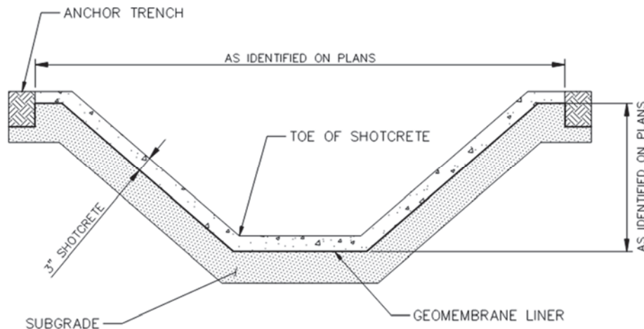
Figure 3. Geomembrane Liner with Shotcrete Schematic
