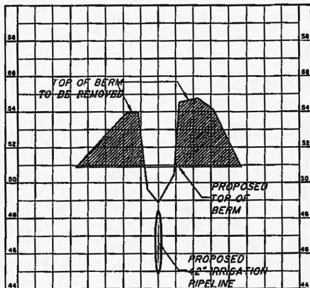
SECTION B-B SCALE=1"=50'
