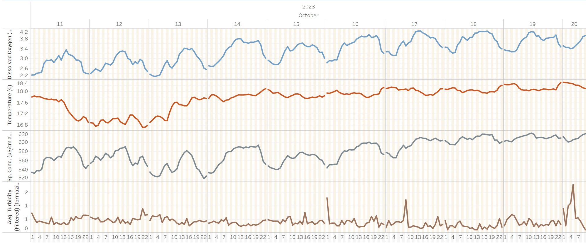
Hourly Average Dissolved Oxygen, Temperature, Specific Conductance, and Turbidity Values
