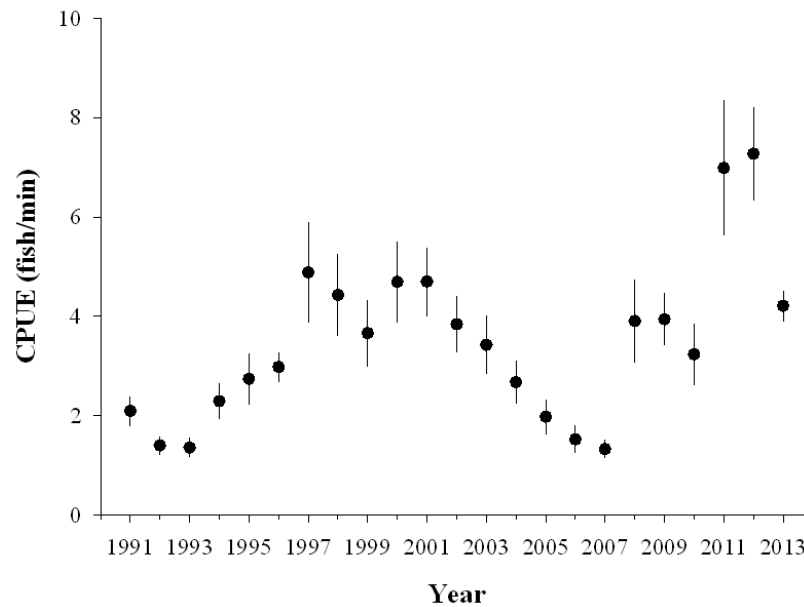
Figure F2.1-1. Overall mean CPUE for rainbow trout among years from all samples combined (by year) from the Lees Ferry reach of the Colorado River, error bars represent 95% confidence intervals.
