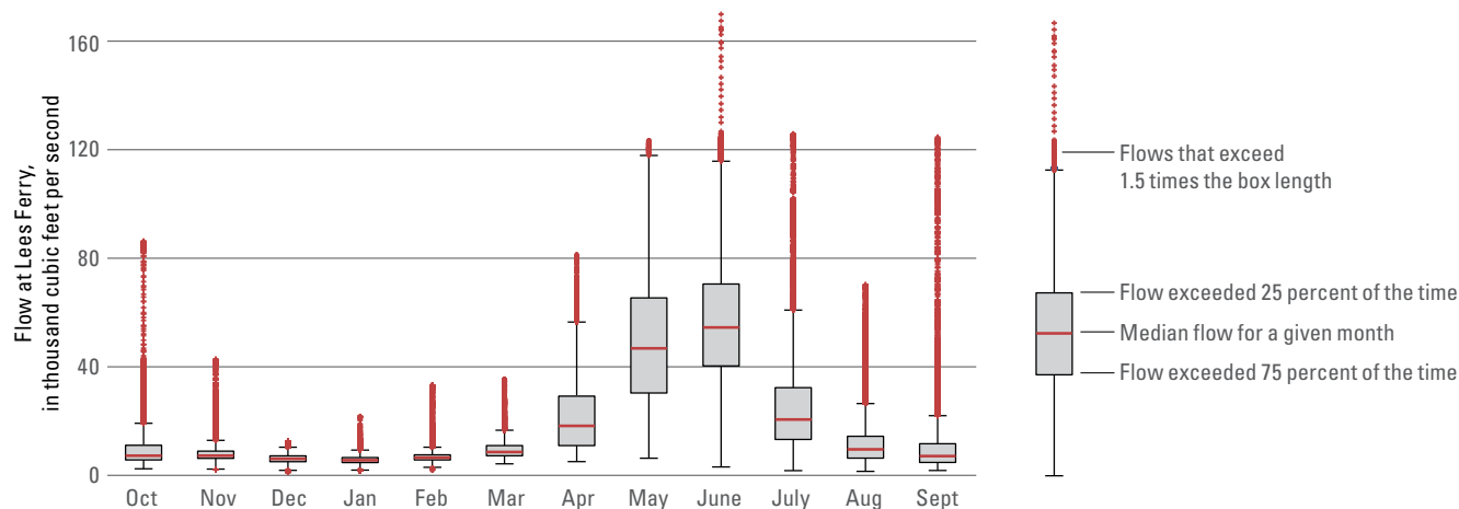
Figure 6. The pre-dam flow regime on the Colorado River at Lees Ferry (data from Topping and others, 2003). The plot shows box-and-whisker diagrams for each month of all instantaneous flow measurements from the beginning of the record (1921) to the beginning of flow regulation by Glen Canyon Dam (1963). The plot illustrates the strong snowmelt signal from April to July as well as the higher flows in the late summer and early fall.
