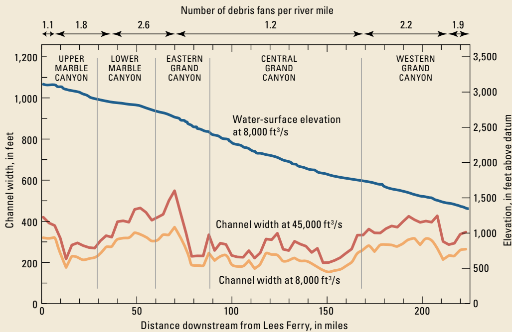
Downstream variations in channel width and water-surface elevation, and the occurrence of debris fans and eddy deposition zones between Lees Ferry and Diamond Creek. From data described by Magirl and others (2008).
