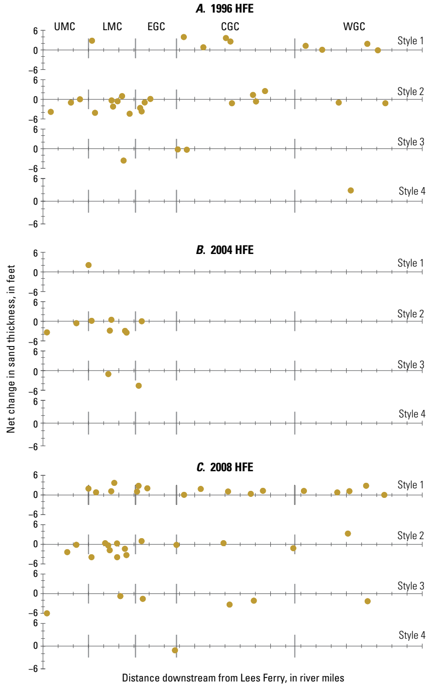
Figure 13. Downstream variations in response style at study sites for the 1996, 2004, and 2008 high-flow experiments (HFEs). Upper Marble Canyon (UMC), lower Marble Canyon (LMC), eastern Grand Canyon (EGC), central Grand Canyon (CGC), and western Grand Canyon (WGC) segments are shown. A , The distribution of total-eddy net change in thickness of sand for each response style with distance downstream for the 1996 HFE. B , The distribution of total-eddy net change in thickness of sand for each response style with distance downstream for the 2004 HFE. Data were not collected in central Grand Canyon or western Grand Canyon. C , The distribution of total-eddy net change in thickness of sand for each response style with distance downstream for the 2008 HFE. Modified from Hazel and others (2010).
