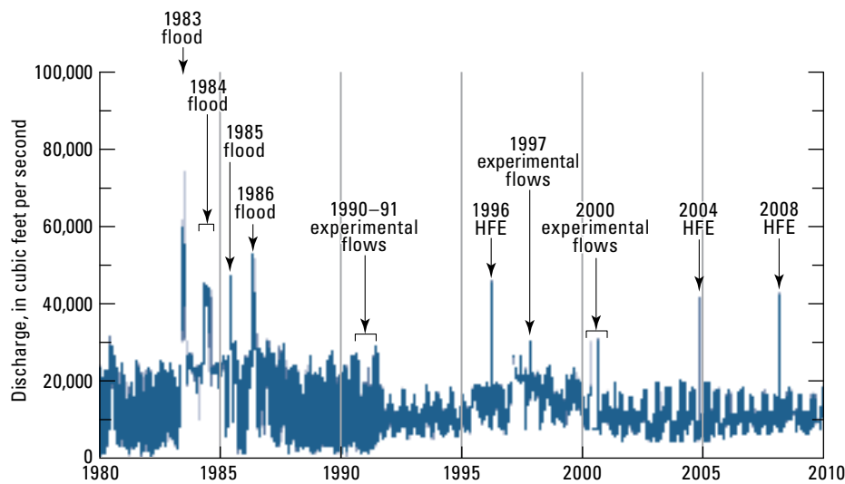
Figure 5. Continuous discharge record for the Colorado River at Lees Ferry for 1980 through 2009. The observations used to construct this record are at 15-minute intervals. Post-dam floods, experimental flows, and high-flow experiments (HFEs) are indicated. Modified from Topping and others (2003).
