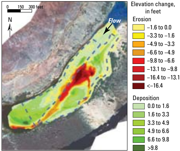
Figure 9. Style 2 deposition and erosion during 2008 high-flow experiment at river mile 44. The dashed lines show the study site boundary and the approximate location of the boundary between the main channel and the eddy. Streamflow is from top to bottom. Modified from Hazel and others (2010).
