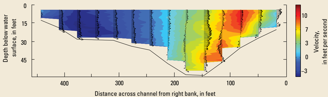
Cross-section view illustrating the three-dimensional characteristics of streamflow during the 2008 HFE. The view is looking downstream and shows the core of high-velocity flow far on the right side of the river. Filled contours are the downstream velocity component; downstream is red and upstream is blue. Arrows show vectors of cross-section and vertical-velocity components. Transect is located at the downstream end of the eddy depicted on the previous page (Wright and Kaplinski, in press).
