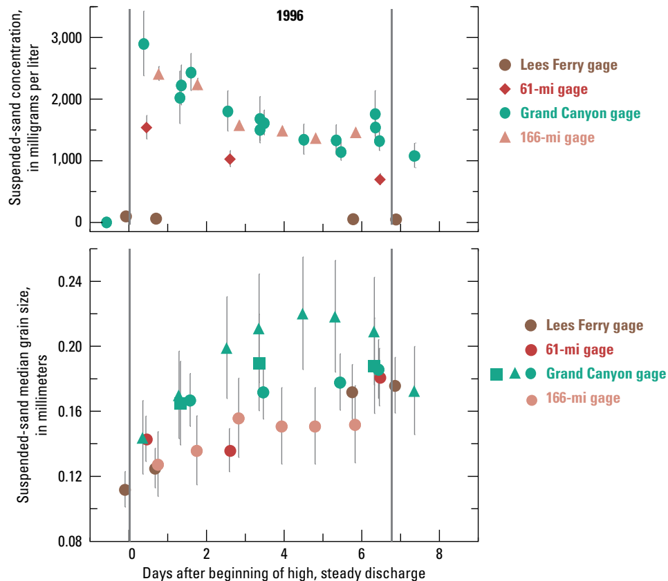
Figure 4A. Suspended-sand data collected during the 1996 high-flow experiment (HFE) at all study sites. The upper graph shows suspended-sand concentration; the lower graph shows suspended-sand median grain size. Data were shifted in time such that zero time (indicated by the leftmost vertical gray line) is the beginning of high, steady discharge during the HFE. The right vertical gray line indicates the end of the high, steady discharge part of the HFE. The symbols represent discrete samples. Error bars indicate the 95-percent confidence interval associated with these measurements. Modified from Topping and others (2010). Gage locations are shown in figure 1.
