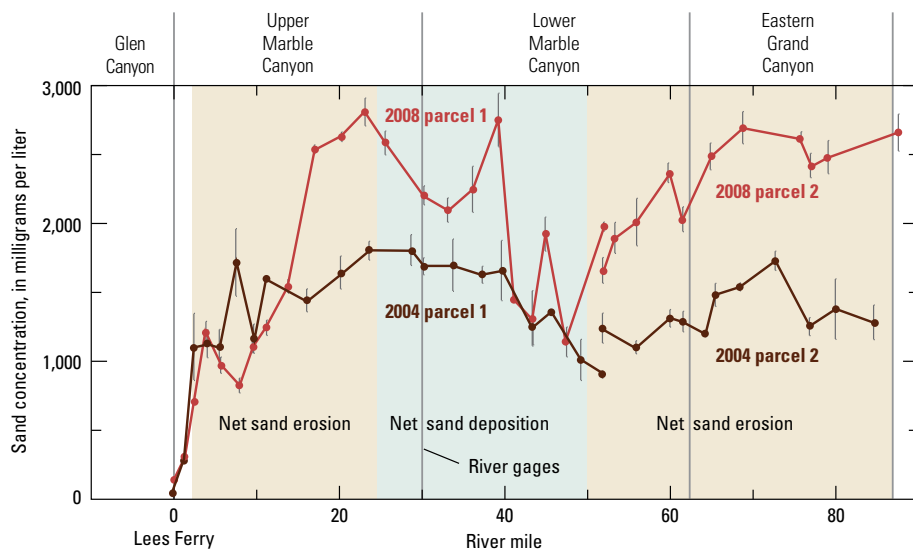
Figure 5. Downstream changes in suspended-sand concentration measured during high-flow experiments in 2004 and 2008. Tan shading indicates reaches of net sand erosion, and blue shading indicates reaches of net sand deposition. “Parcel 1” indicates sampling on the first day of the steady high flow, and “parcel 2” indicates sampling on the second day of the steady high flow. Vertical lines indicate locations of the Lees Ferry, 30-mile, 61-mile, and Grand Canyon gages. Modified from Topping and others (2010). Gage locations are shown in figure 1.
