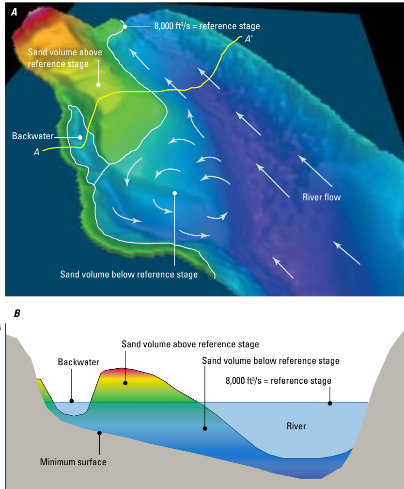
Figure 3. A, Perspective view based on 3-foot resolution digital elevation model of a typical eddy sandbar and the adjacent channel showing pattern of recirculating flow, the reference stage of 8,000 ft 3 /s in white, and a typical backwater as defined by aquatic ecologists. The portions of the sandbar above the reference stage and below the reference stage are distinguished. Main-stem flow is from bottom right to top left. B, Cross-section view of an eddy sandbar and channel illustrating the region for sand above the reference stage and total sand (sand above the reference stage plus sand below the reference stage). Modified from Grams, Hazel, and others (2010).
