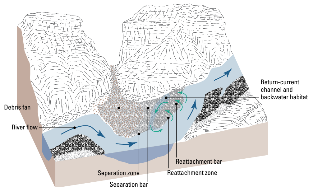
Figure 10. Diagrammatic illustration of a typical fan-eddy complex, including reattachment sandbar, return-current channel, and backwater habitat. Main channel flow is from left to right. The separation zone is the area where downstream flow separates from the bank, and the reattachment zone is the area where downstream flow reattaches to the bank. The small arrows indicate the primary cell of recirculating flow within the eddy at flows during which the sandbar would be submerged. Modified from Schmidt and Graf (1990).
