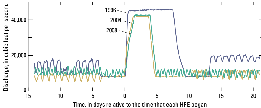
Figure 6. Continuous discharge record for the Colorado River at Lees Ferry for three high-flow experiments (HFEs). The 1996 HFE began at 12:00 a.m. on March 26, 1996; the 2004 HFE began at 12:00 a.m. on November 21, 2004; and the 2008 HFE began at 6:00 p.m. on March 4, 2008.
