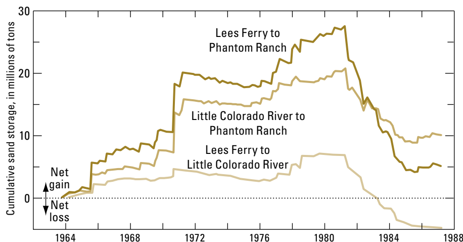
Figure 8. Cumulative sand storage between the Lees Ferry and Grand Canyon gaging stations (river miles 0–88), based on the assumption that the same discharge always transports the same amount of sand. From U.S. Department of the Interior, 1995, fig. III-15.
