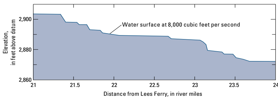
Figure 9. Longitudinal profile of the Colorado River water surface from river mile 21 to 24 in Marble Canyon showing the relatively flat pool segments separated by short and relatively steep rapids. The water-surface profile is based on data collected by light detection and ranging (lidar) in March 2000, when the release from Glen Canyon Dam was steady at 8,000 cubic feet per second (Magirl and others, 2005).
