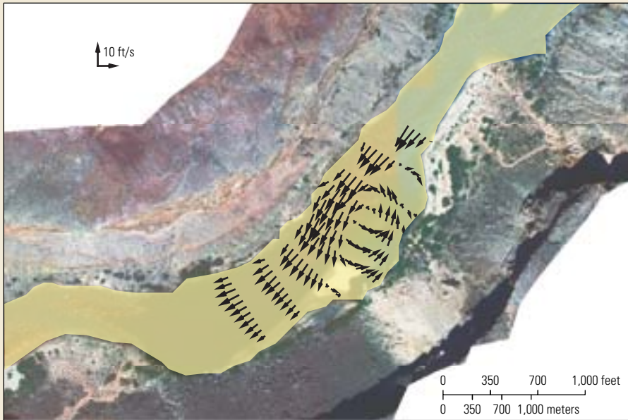
Depth-average horizontal velocities measured at peak flow during the 2008 HFE at the fan-eddy complex shown on the previous page. Scale bars indicate the speed of the flow. Modified from Wright and Kaplinski (in press).
