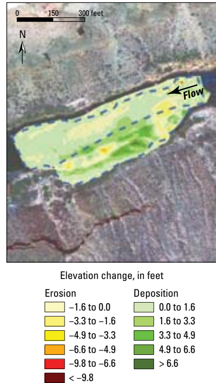
Figure 8. Style 1 net depositional response to the 2008 high-flow experiment at river mile 172. The dashed lines show the study site boundary and the approximate location of the boundary between the main channel and the eddy. Streamflow is from right to left. Modified from Hazel and others (2010).
