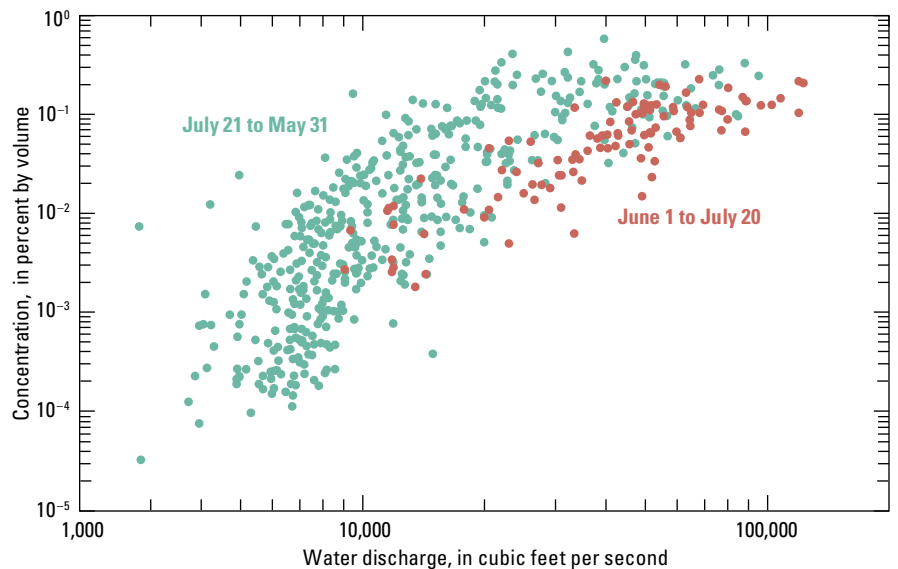
Figure 7. Suspended-sand concentration and discharge of the Colorado River near the Grand Canyon gage at river mile 88 during the pre-dam period (1944–62). Concentrations shown are the average for the measurement section based on depth-integrated samples. The red symbols represent data collected from June 1 to July 20, and the green symbols represent data collected from July 21 to May 31. As described in the text, the systematic nature of the time when measured concentrations were relatively high or low indicates that the scatter is not random and is related to the amount and size of sand available for transport and its distribution on the bed and along the channel margins. Modified from Topping, Rubin, and Vierra (2000, fig. 4b).
