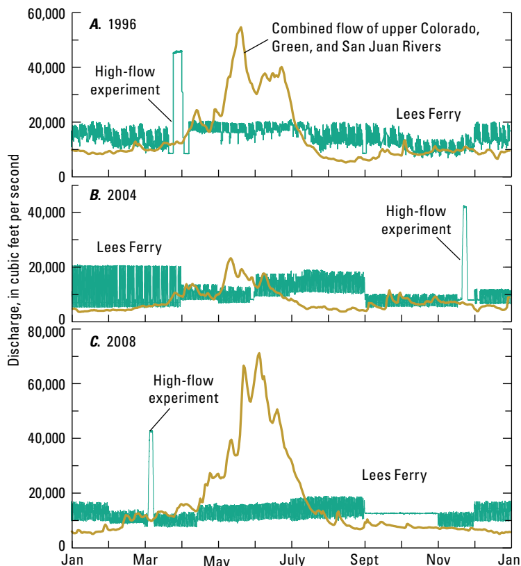
Figure 4. Discharge of the Colorado River at Lees Ferry and the estimated inflow to Lake Powell for the years when the three high-flow experiments occurred. A , 1996. B , 2004. C , 2008. Inflow to Lake Powell was estimated as the sum of measured discharge each day at the Green River at Green River, Utah (U.S. Geological Survey station 09315000), the Colorado River near Cisco, Utah (U.S. Geological Survey station 9180500), and the San Juan River near Bluff, Utah (U.S. Geological Survey station 9379500).
