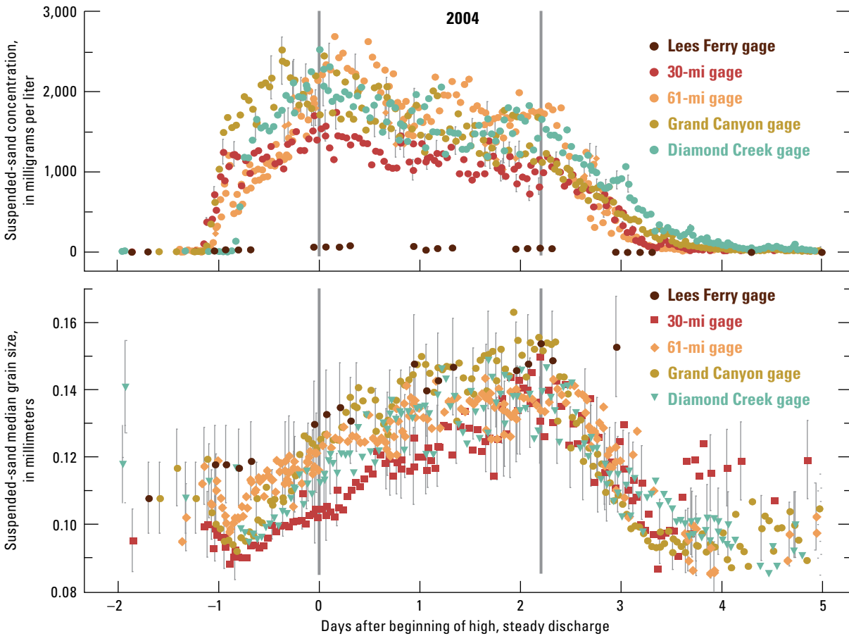
Figure 4B. Suspended-sand data collected during the 2004 high-flow experiment (HFE) at all study sites. The upper graph shows suspended-sand concentration; the lower graph shows suspended-sand median grain size. Data were shifted in time such that zero time (indicated by the leftmost vertical gray line) is the beginning of high, steady discharge during the HFE. The right vertical gray line indicates the end of the high, steady discharge part of the HFE. The symbols represent discrete samples. Error bars indicate the 95-percent confidence interval associated with these measurements. Modified from Topping and others (2010). Gage locations are shown in figure 1.
