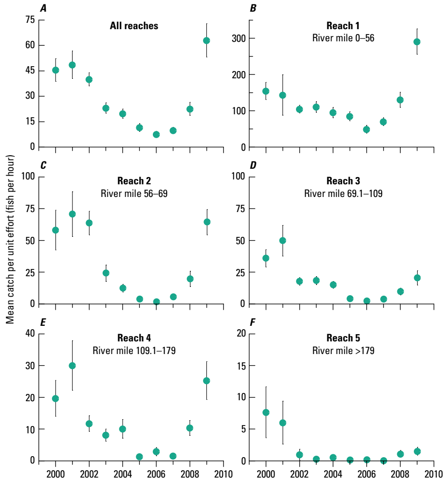
Figure 6. Mean catch per unit effort (fish per hour) of rainbow trout captured during electrofishing surveys on the Colorado River between Lees Ferry and Lake Mead, 2000–2009. A , All reaches. B , Reach 1. C , Reach 2. D , Reach 3. E , Reach 4. F , Reach 5. Points represent the average among sites and seasons, and bars represent \pm 2 standard errors of the average, an approximation for a 95-percent confidence interval. From Makinster and others (2010).
