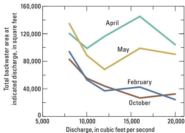
Figure 23. The relation between total backwater habitat area and discharge for the sandbar and backwater monitoring sites in 2008. Modified from Grams, Schmidt, and Andersen (2010).
