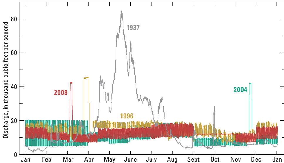
Figure 5. Discharge of the Colorado River at Lees Ferry (U.S. Geological Survey gaging station 9380000) for the calendar years during which the three high-flow experiments occurred—1996, 2004, and 2008—and 1937. The 1937 discharge record is shown because it represents a typical pre-dam year. The 1937 instantaneous peak discharge of 84,800 cubic feet per second was equal in magnitude to an average pre-dam flood likely to occur approximately every 2 years.
