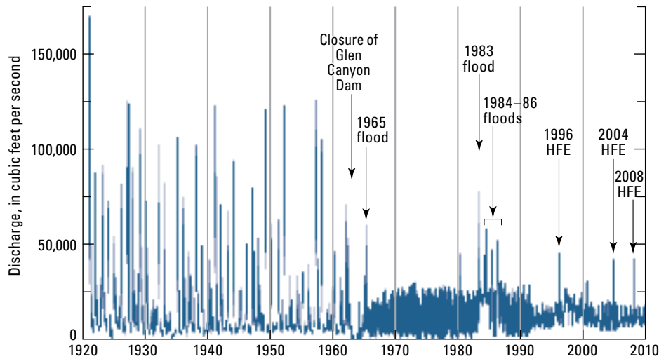
Figure 3. Continuous-discharge record for the Colorado River at Lees Ferry (river mile 0) for 1921 through 2009. With the exception of the first 2 years, the observations used to construct this record are at intervals of 30 minutes or less. Closure of Glen Canyon Dam and post-dam floods and high-flow experiments (HFEs) are indicated. Modified from Topping and others (2003).
