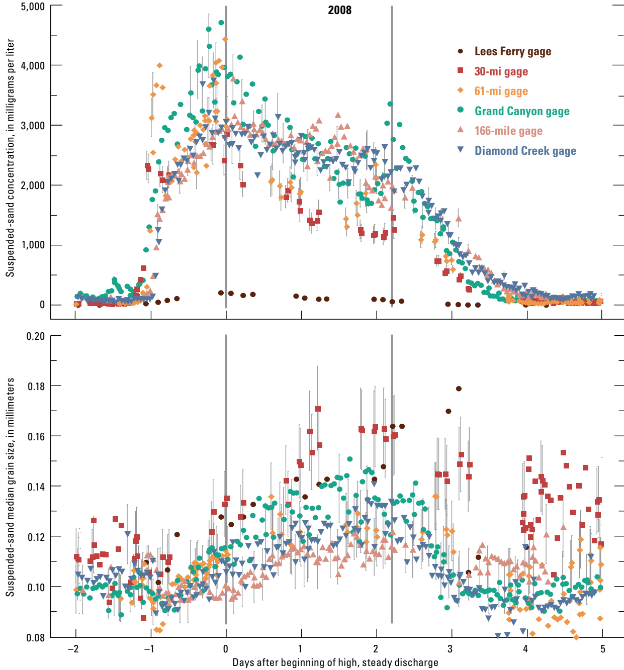
Figure 4C. Suspended-sand data collected during the 2008 high-flow experiment (HFE) at all study sites. The upper graph shows suspended-sand concentration; the lower graph shows suspended-sand median grain size. Data were shifted in time such that zero time (indicated by the leftmost vertical gray line) is the beginning of high, steady discharge during the HFE. The right vertical gray line indicates the end of the high, steady discharge part of the HFE. The symbols represent discrete samples. Error bars indicate the 95-percent confidence interval associated with these measurements. Modified from Topping and others (2010). Gage locations are shown in figure 1.
