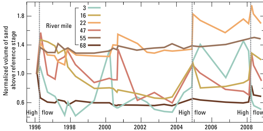
Figure 19. Normalized sandbar volume above the reference stage at selected sites for February 1996 to October 2009. Normalized means that the values shown are relative values; they are shown as the ratio of sandbar volume measured on the indicated date to sandbar volume measured in February 1996, before the 1996 high-flow experiment. Each high flow is shown by a vertical dotted gray line.
