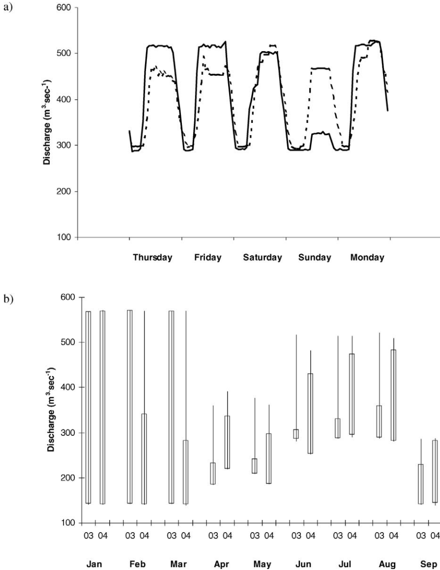
FIGURE 1.—(a) Hydrograph of releases from Glen Canyon Dam during a typical 5-d period in 2003 (July 10–14; solid line) and 2004 (July 8–12; dashed line) and (b) the average daily minimum and maximum flows during the week (lines) and on Sundays (bars) from January through September. The monthly averages of the daily minimum and maximum flows are based on 15-min automated flow measurements taken at Glen Canyon Dam.
