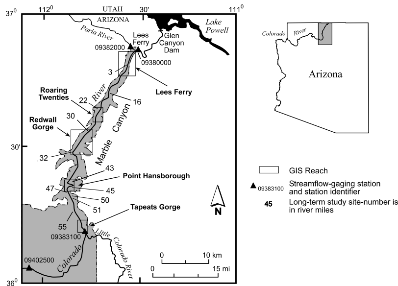
Figure 2. Colorado River in Marble Canyon, Arizona. The shaded area is Grand Canyon National Park. Shown are the locations of the U.S. Geological Survey streamflow-gauging stations, the 5 GIS-based reaches, and the 11 long-term study sites. The long-term study sites are referred to by distance in river miles downstream relative to Lees Ferry (river mile 0).
