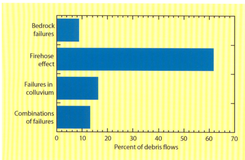
Figure 3. Initiation mechanisms for selected debris flows between 1939 through 2002 in Grand Canyon (n = 68; modified from Griffiths and others, 1997).
