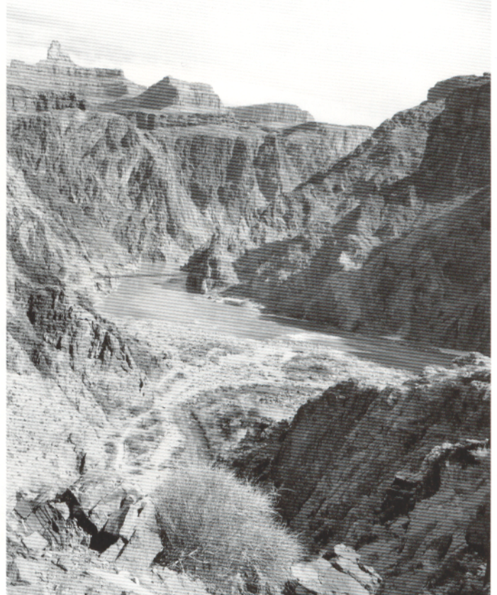
Figure 2. Replicate photographs of the debris fan at Bright Angel Creek (river mile 87.8-R). (A) (February 5, 1890) Bright Angel Creek, a perennial stream, has its headwaters on the North Rim. In 1890, the channel is distinct, relatively narrow, and hooks right to join the Colorado River beyond the cliff at lower right (photograph by Robert Brewster Stanton). (B) (February 13, 1991) Beginning in December 1966, several debris flows have significantly changed the debris fan, moving the edge of the debris fan closer to the Colorado River (photograph by Ted Melis).
