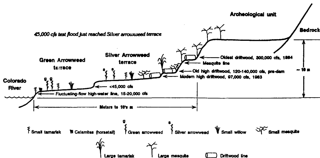
Figure 2. Strandlines and terraces in eastern Grand Canyon. Shown schematically are terrace treads and risers, strandlines marked by driftwood lines, and the vegetation types characteristic of each terrace level.
