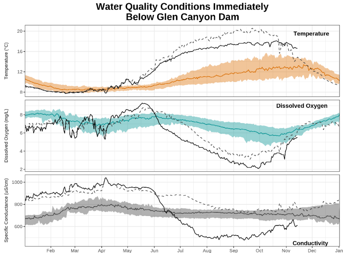
Figure 1. Water quality record from Glen Canyon Dam near Page, AZ (gaging station #09379901*) for temperature (A) dissolved oxygen (B) and specific conductance (C). Dashed and solid lines show daily median values for calendar years 2022 and 2023 respectively (medians are from the continuous data record, logging at 15-minute increments). Colored lines show the long-term median value for each parameter and the orange, blue, and brown color bands represent the daily 10 th and 90 th quantiles of temperature, dissolved oxygen and specific conductance, respectively. The water quality record represented in this figure contains 12 years of data for temperature and dissolved oxygen, and nine years of data for specific conductance. *Data from this site are currently posted and available through June 2023 at https://www.gcmrc.gov/discharge_gw_sediment/station/GCDAMP/09379901 ; more recent data are filtered raw values that are awaiting further quality assurance before being posted online. Figure adapted from U.S. Geological Survey (2024).
