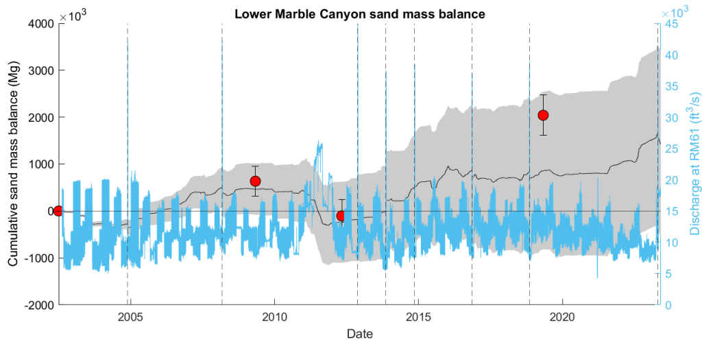
Figure 2. Mass balance sand budget for Lower Marble Canyon from August 2002 to December 2022. The black line shows the mass balance computed from continuous measurements of sediment flux measured by Project A with uncertainty shown by the gray shaded region. The red circles show the mass balance for the same river segment computed from repeat measurements of riverbed elevations measured by Project B.2. These data illustrate the necessity of the Project B.2 measurements of riverbed elevation to compute sediment storage changes over time periods greater than approximately five years. Data from Topping and others (2021), Grams and others (2013), Grams and others (2019), and unpublished data.
