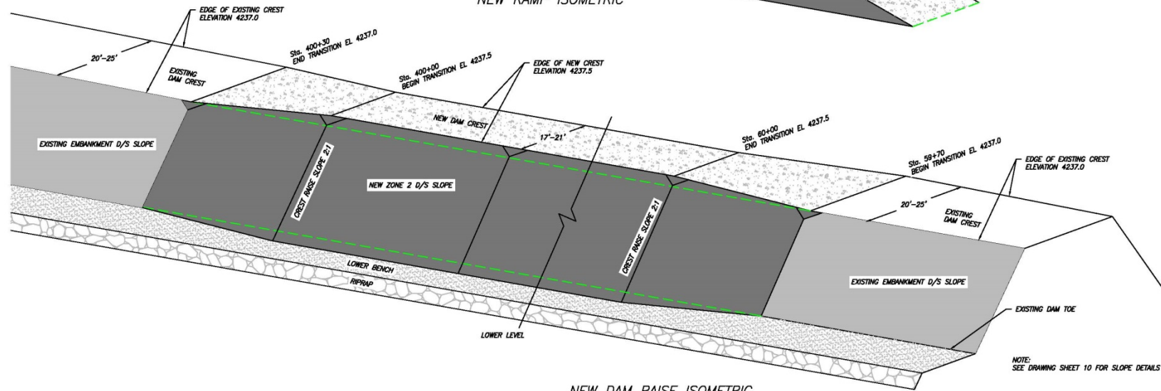
NEW DAM RAISE ISOMETRIC
