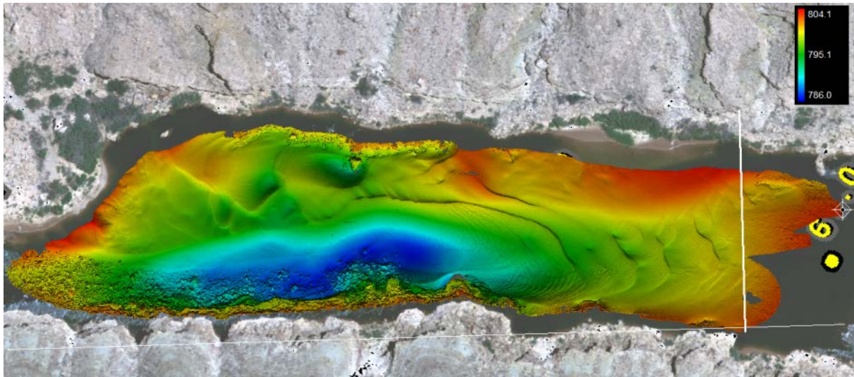
Figure 15. Bathymetry (measured in May 2014) of the sediment gaging pool at RM61. Repeat surveys of this area (in May 2009, May 2012, and August 2013) have revealed an active and consistently well-developed dune field.
