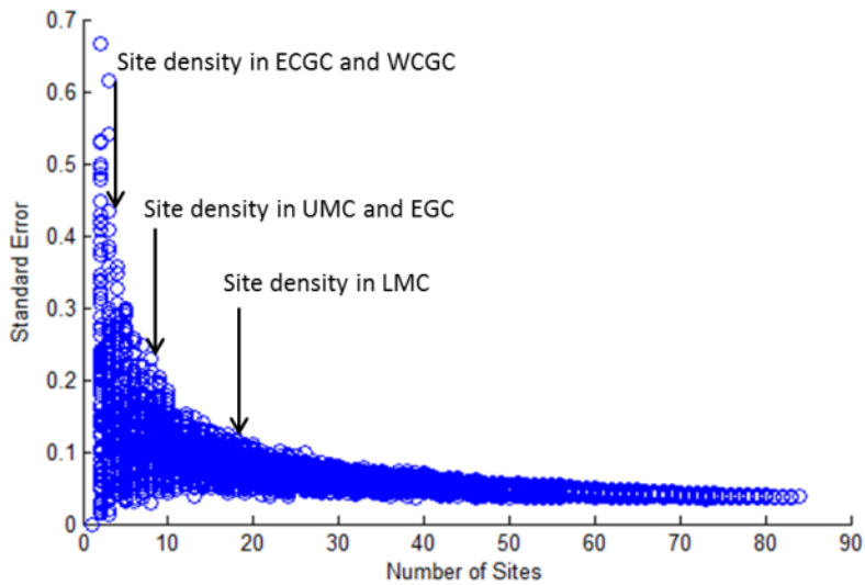
Figure 6. Bootstrap simulation of expected standard error (m) for estimates of sandbar thickness change as a function of sample size. Measurements of thickness change for 84 sandbars in lower Marble Canyon (data from Project 3.2) were sampled randomly using increasing sample size (1 to 84). For each sample size, 100 random selections of sites (numbering between 1 and 84) were made from among the 84 sites, and the standard error calculated and plotted. The standard error decreases quickly with increasing sample size up until n \sim 20 . Standard error decreases more gradually thereafter. The sample site density in lower Marble Canyon (LMC) achieves a reasonable uncertainty for the number of sites. More sites would be required in east central Grand Canyon (ECGC), west central Grand Canyon (WCGC), upper Marble Canyon (UMC), and eastern Grand Canyon (EGC).
