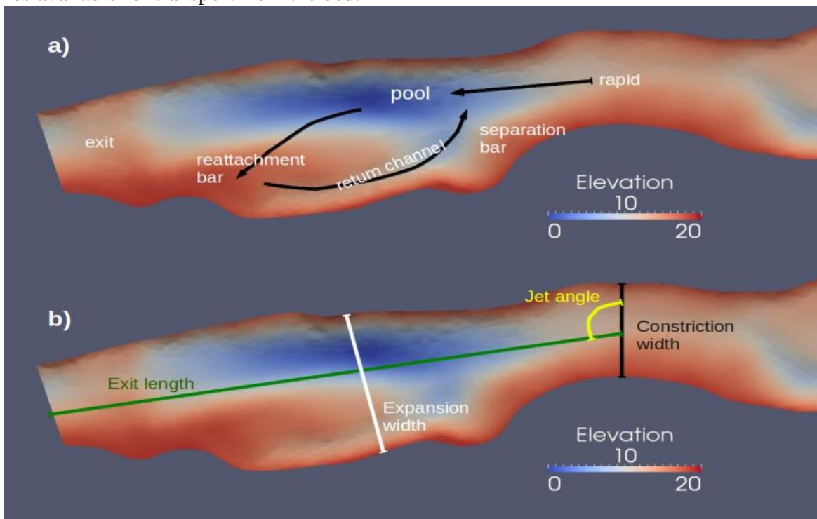
Figure 12. a) General topography of an eddy and b) geometric parameters influencing flow hydraulics.
