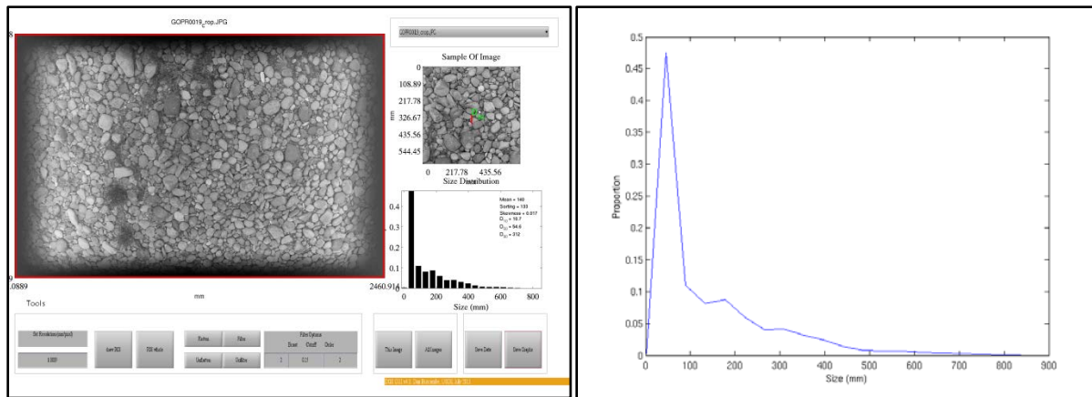
Figure 10. Example of coarse-grained size distribution derived from digital still image taken from the surface of a point bar located along the river right shoreline about 9 miles upstream of Lees Ferry in Glen Canyon (preliminary data, Buscombe and Melis, US Geological Survey, 2013), using the algorithm of Buscombe (2013).
