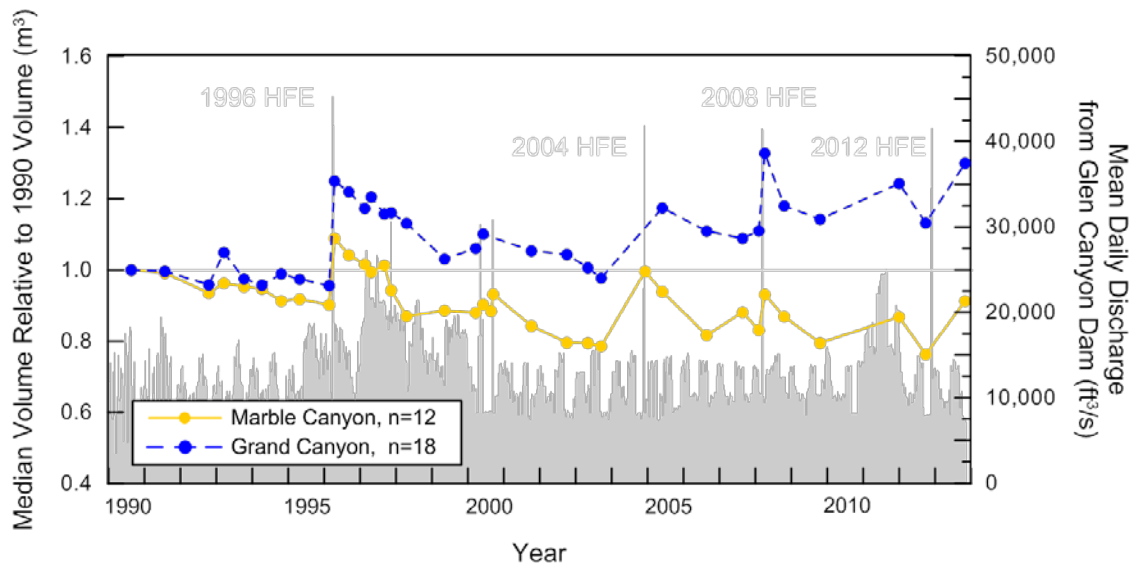
Figure 5. Sandbar size from 1990 to October 2013 (preliminary data provided by Joseph E. Hazel, Jr.).
