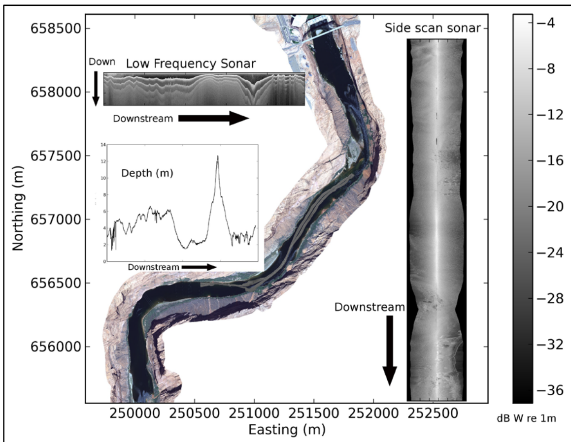
Figure 8. Example of “Humminbird®” sidescan imagery of the riverbed near -9 mile bar in Glen Canyon showing a patchy riverbed with fine to coarse gravels and clumps of submerged vegetation (shadow areas). Ongoing work is trying to relate each observed texture to a substrate type using underwater video for reference (preliminary data, Buscombe and Melis, US Geological Survey, 2013).
