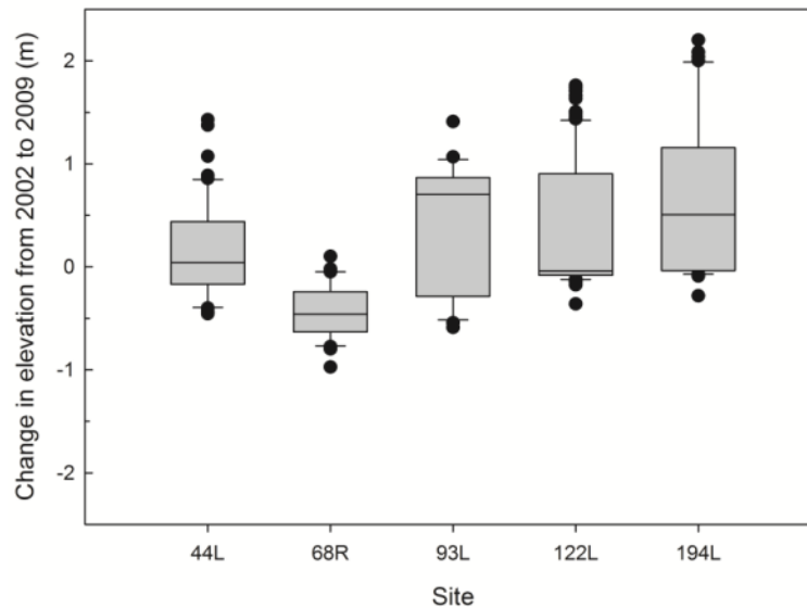
Figure 8. Box plots showing distribution of changes in elevation determined from total station surveys in 2002 and 2009 at five sandbar monitoring sites.
