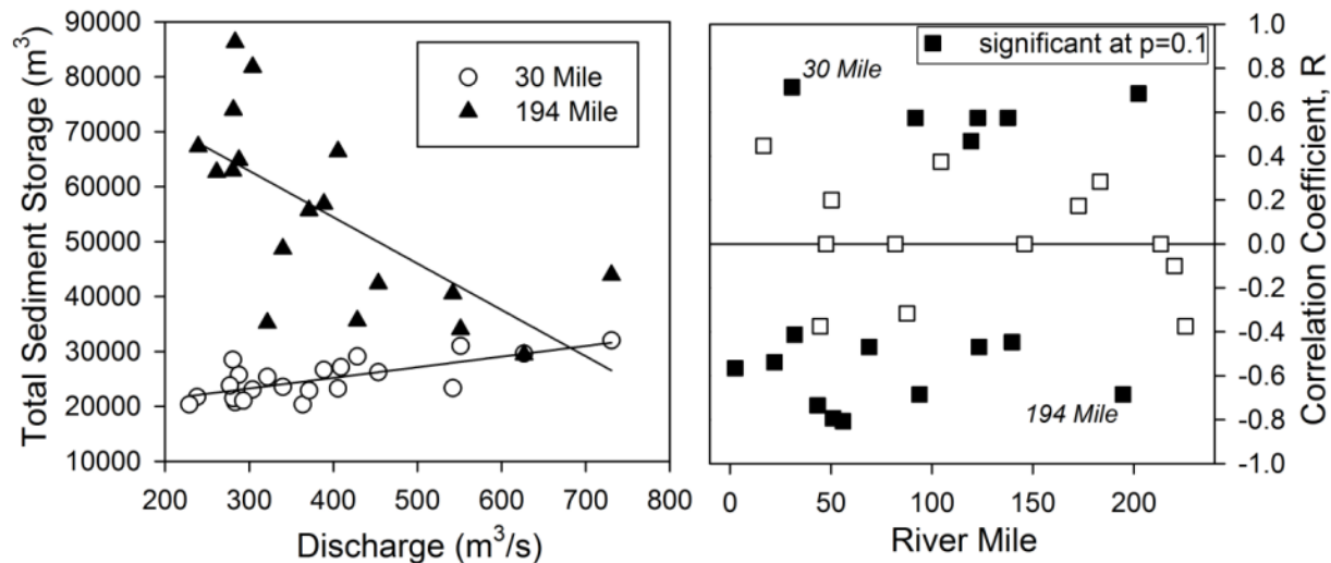
Figure 11. Left) Changes in observed total sand storage as a function of recent discharge for two of the long-term monitoring sites. Right) Downstream trends in the correlation coefficient, R , of the discharge-sediment storage relations. Positive (negative) values indicate increases (decreases) in sediment storage with discharge; closed (open) squares are locations where the regression is (is not) significant.
