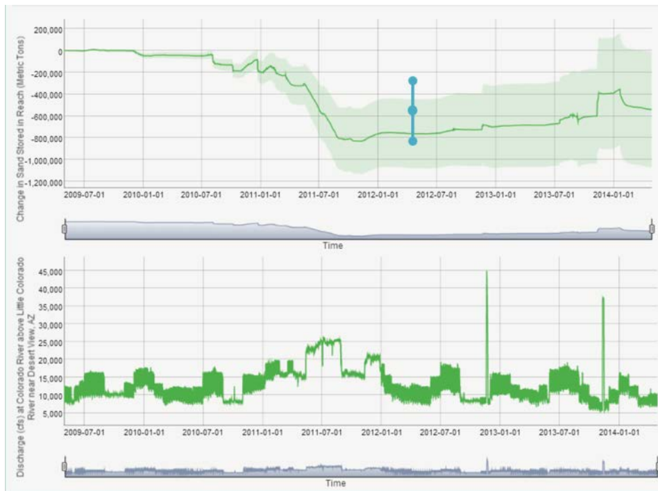
Figure 3. Sand budget for May 1, 2009 to April 30, 2014 for lower Marble Canyon (upper plot) and discharge of the Colorado River at the downstream end of the segment for the same period (lower plot). The sand budget computed by the difference in sand transport at the upstream and downstream ends of the reach is shown by the solid line with the shaded region indicating the uncertainty. Each point on the line is the sand budget for the time period between the start date and the date indicated on the horizontal axis. The uncertainty associated with each measurement contributes to the total uncertainty and increases quasi-linearly with time. The morphologic sand budget for the same reach computed by the measurements of deposits in the channel in 2009 and 2012 is shown by the filled circle with error bars, shown at the time at which the repeat measurements were made (May 2012).
