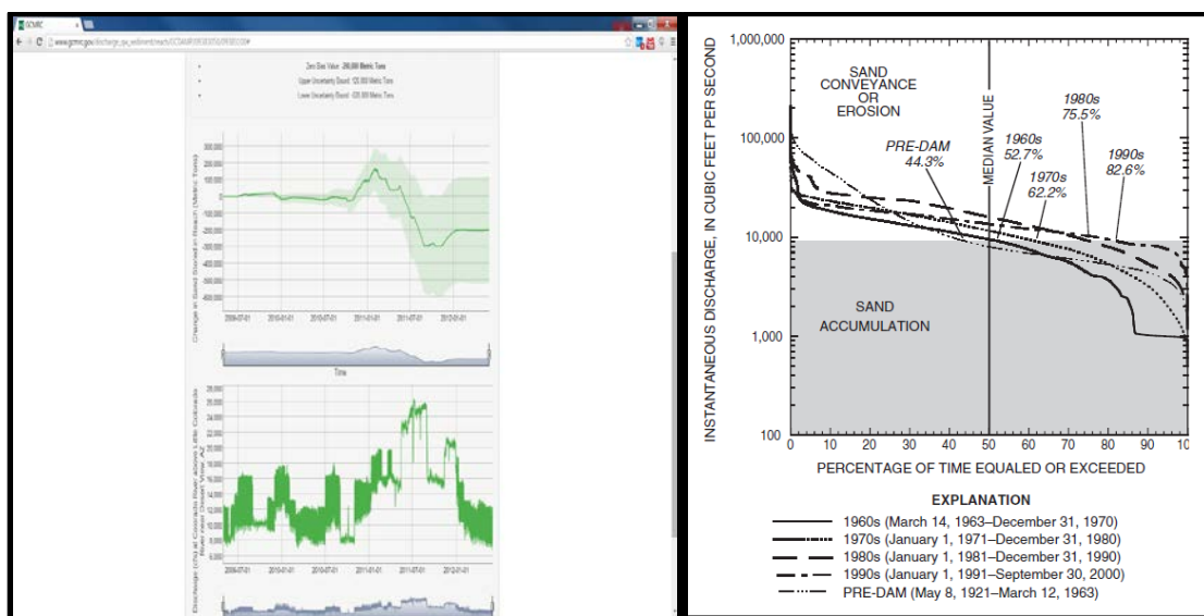
Figure 5. Left - cumulative sand budget for Lower Marble Canyon (river miles 30-61) from May 2009 to June 2012, and discharge at the Colorado River above the Little Colorado River near Desert View, AZ. Although the budget over this 3-year period is still technically indeterminate within the uncertainty bounds, it more clearly suggests sand mass export from Lower Marble Canyon (GCMRC preliminary sand budget, 2014; www.gcmrc.gov ), and the downward trend in sand storage supports topographic channel-bed monitoring of the segment from May 2009 to May 2012, that indicates about 0.47(+/-0.15) Tg of sand were eroded from the main channel of Lower Marble Canyon in the period between the mapping surveys (Grams and others, preliminary data, USGS 2014). Right - Flow-duration curves for the Colorado River at Lees Ferry from each of the four post-dam decades and the entire pre-dam period. The gray shaded region shows the pre-dam discharge range under which sand accumulated in the reach between the Lees Ferry and Grand Canyon gaging stations, in Marble and upper Grand Canyons. The percentages of time when these discharges were exceeded during each period are indicated in italics (from Topping and others, 2003). This trend suggests that MLFF has probably been effective at keeping the channel bed in lower Marble Canyon highly winnowed with respect to sand and finer sediments, and implementation of the 2012-20 HFE protocol, allowing annual clear water floods annually in the fall might also be providing areas of gravel exposure and lower water turbidity during the December through June periods; seasons when rainbow trout are typically known to spawn below Glen Canyon Dam.
