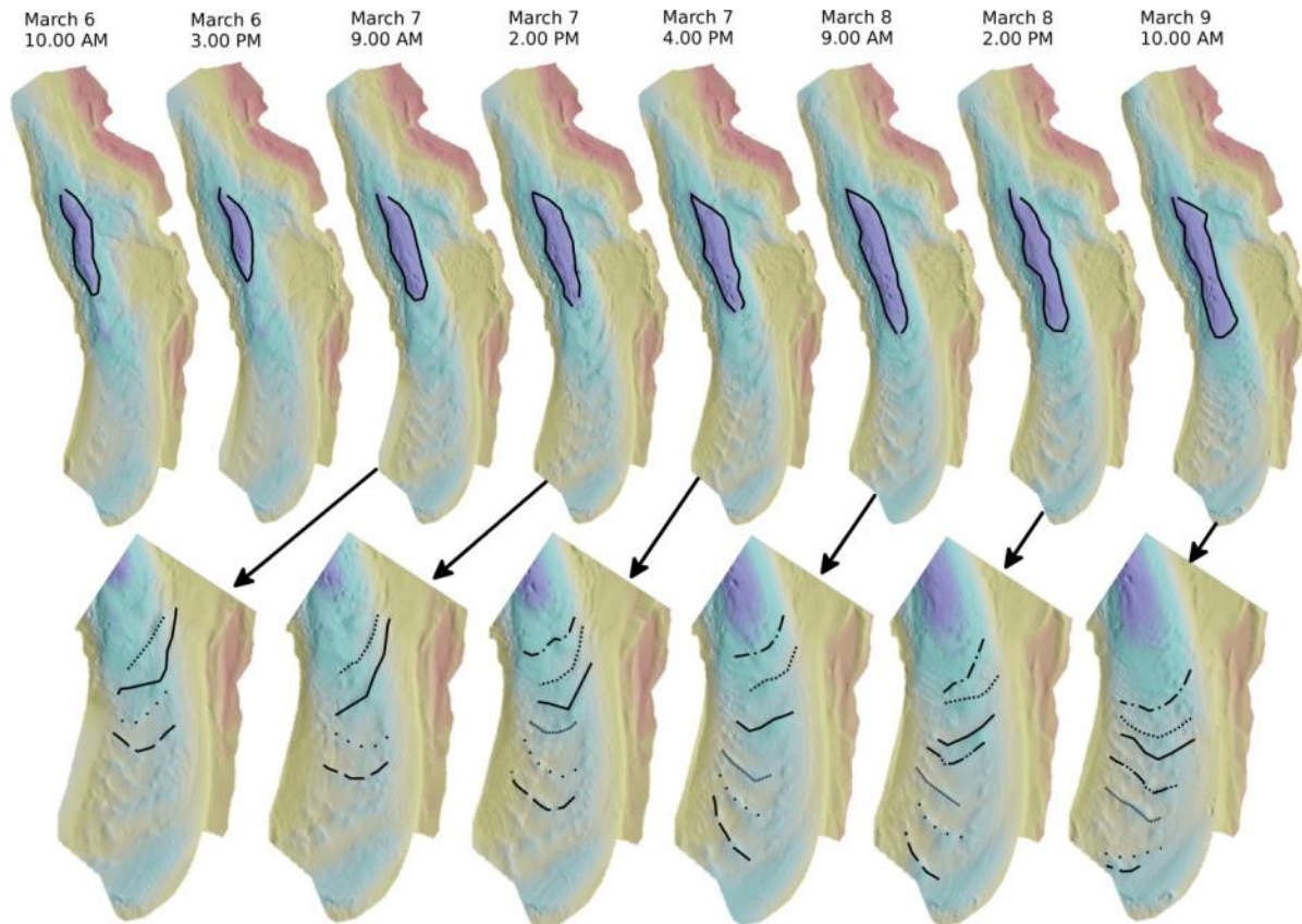
Figure 14. Evolution of the bed at Eminence during the 2008 HFE (data from Wright and Kaplinski, 2011) showing significant bed deformation and migration of bedforms over the timescale of hours to days.
