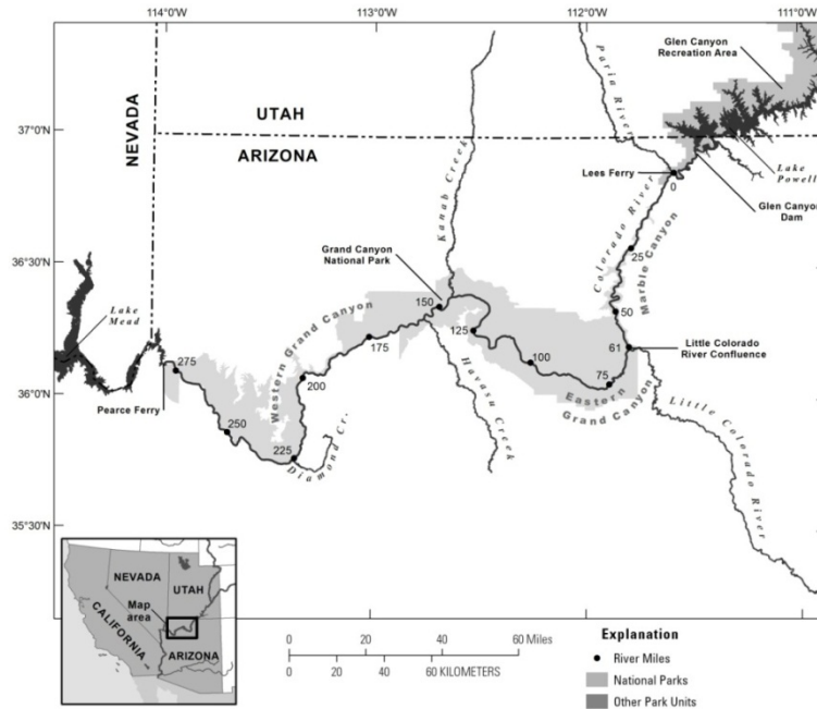
Figure 2. Four landscape-scale segment used for stratification (Glen Canyon, Marble Canyon, Eastern Grand Canyon, and Western Grand Canyon). The confluences of the Paria, and the Little Colorado Rivers, and Kanab Creek with the Colorado River separate the four segments.
