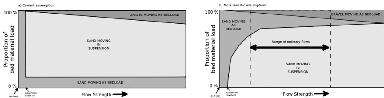
Figure 13. Schematic of how the relative proportions of bed material load (total load minus wash load) change with increasing flow strength. Two scenarios are presented: (a) represents the current assumption that bedload is a constant proportion of bed material load; and (b) depicts the new hypothesis to be tested in this study that the proportion of bed material load moving as bedload is a function of flow strength.
