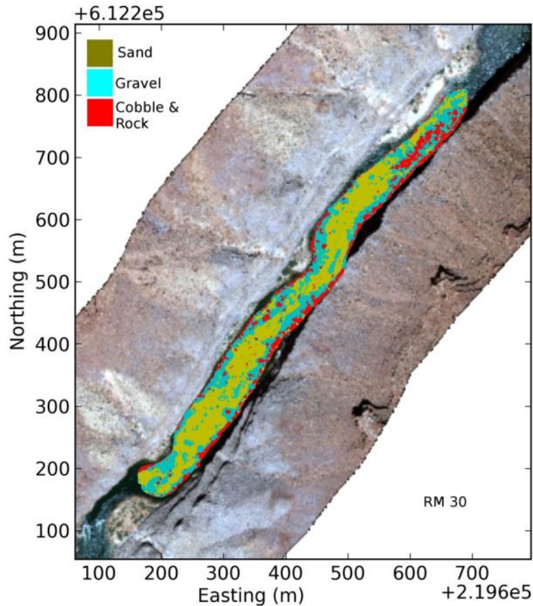
Figure 10. Acoustic sediment classification at RM30, August 2013, using the methods of Buscombe and others (in review). The resolution of classification is 25 cm 2 .
