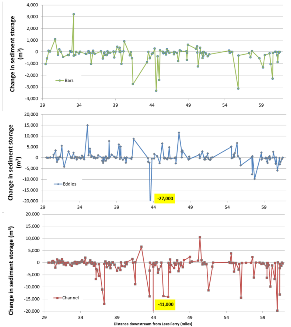
Figure 4. Change in sediment storage between May 2009 and May 2012 for lower Marble Canyon computed by comparing the maps (DEMs) of the channel made in those two years. Each marker represents a surveyed pool. Note the different vertical scales. In this period with a net decrease in sediment storage (Fig. 4), the eddies exhibited a small net increase in storage while the bars and the channel both lost sediment. The largest changes occurred in the channel and were concentrated in relatively few pools.
