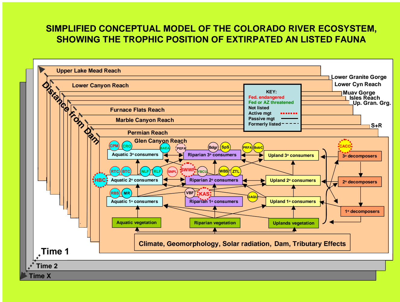
Fig. 2: The Colorado River ecosystem, depicting four trophic levels affected by the dam and physical factors, through the geomorphic reaches of the river and over time. The relationships of some extirpated and at-risk species are depicted within their trophic levels as circles. Abbreviations for species are found in Table 1. Most management attention is focused on CACO, HBC, KAS, and SWWL (large circles), but other endangered (red text), threatened (blue text), and non-federally listed (black text) species also occurred in the CRE or appear to be at-risk of extirpation there.
