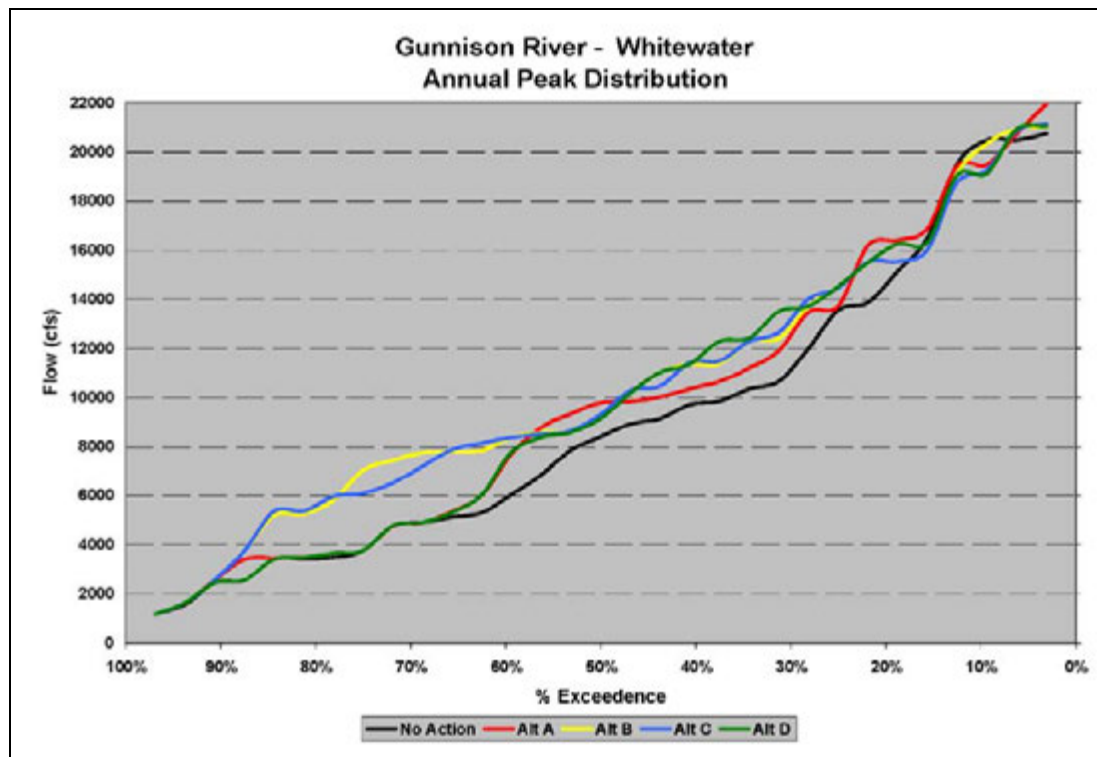
Figure 3.3- 14—Annual Peak Distribution at Whitewater
