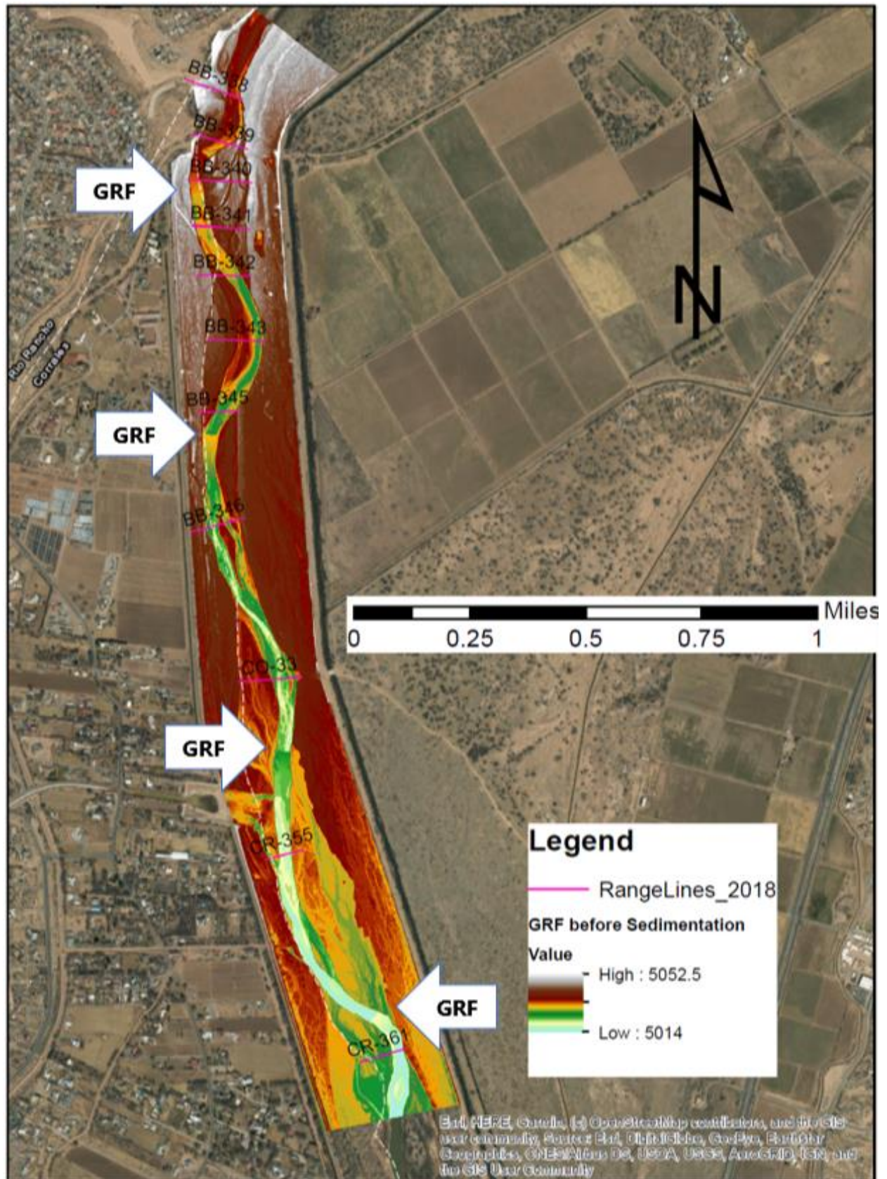
Figure 39: Digital Elevation Model of GRF before sedimentation alternative
