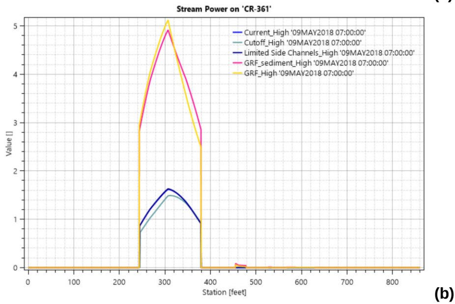
Figure 84: a) Cross section of terrain for all four models on CR-361 and, b) Stream Power at CR-361
