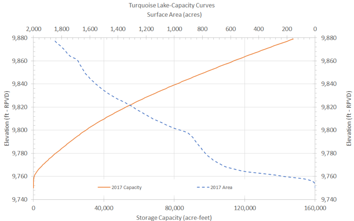
Figure 1. Turquoise Lake surface area and storage capacity curves based on the 2017 survey. Use the elevation axes to find the storage capacity (orange curve, bottom axis) or surface area (blue dotted curve, top axis) for a given reservoir elevation.
