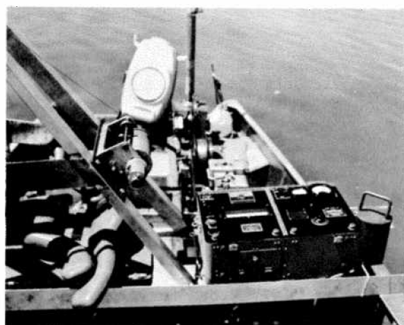
Figure 9. View of sonic depth recorder cabinet (in right foreground). Photo P258-D-57706
