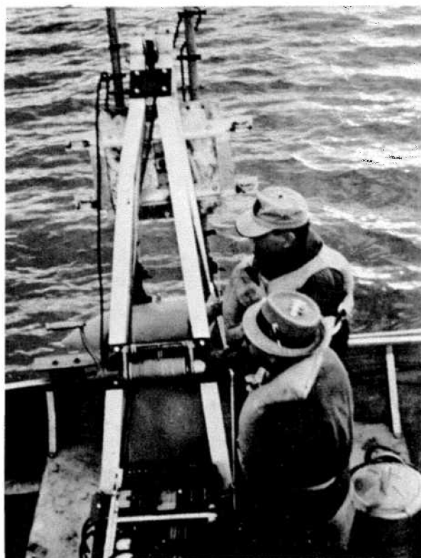
Figure 4. Sonic depth recording equipment. Transducer is out of water. Photo P258-D-57761
