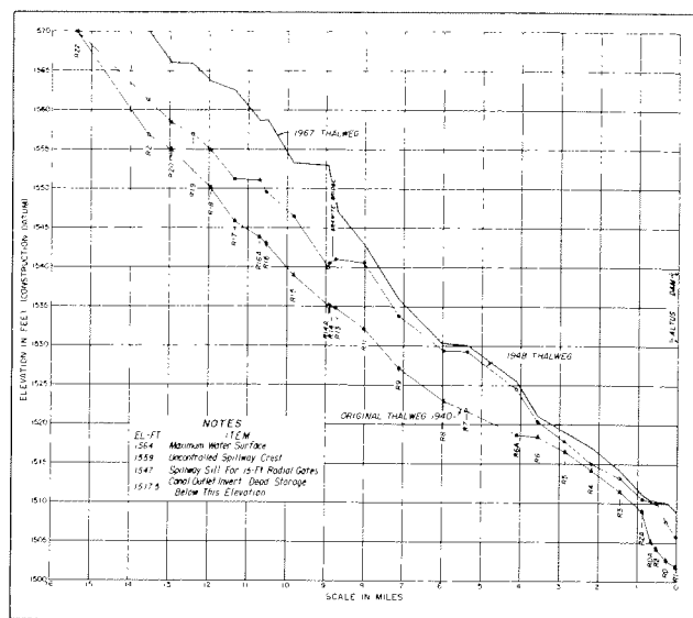
Figure 17. Longitudinal profiles.
