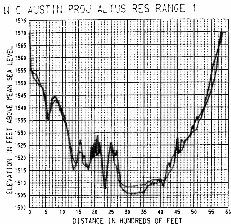
Figure 28. 1948 and 1967 sedimentation range profiles—Range 1.
