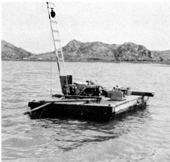
Figure 10. Gravity core sampler shown suspended from a cable and lying on the platform of the raft. Photo P258-D-57699
