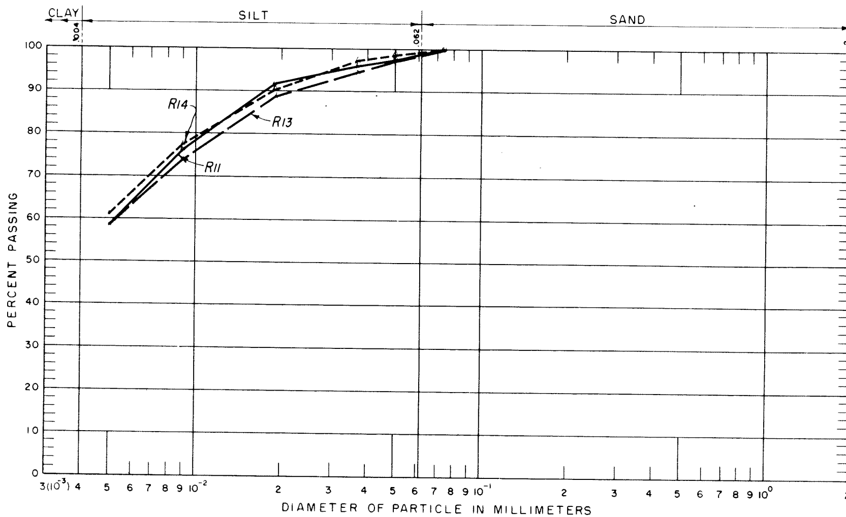
Figure 19. Particle size analysis curves. Ranges 11, 13, and 14—1948 survey.
