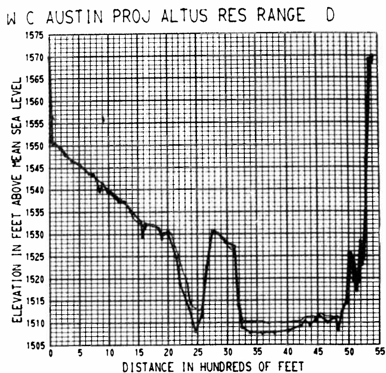
Figure 29. 1948 and 1967 sedimentation range profiles—Range D.
