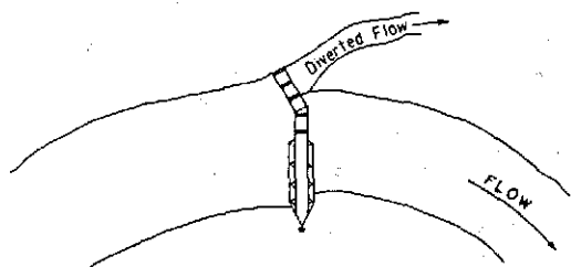
B. Good diversion site to exclude sediment, but not for floating ice or debris
