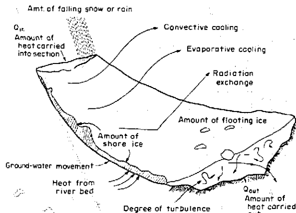
Figure A-1. Ice formation—Factors that affect the rate of cooling of a section of river water. 101-D-630
