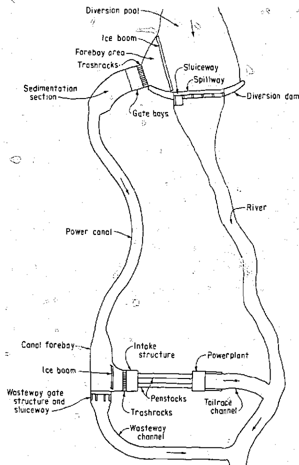
Figure 1. Typical diversion to power canal. 101-D-625
