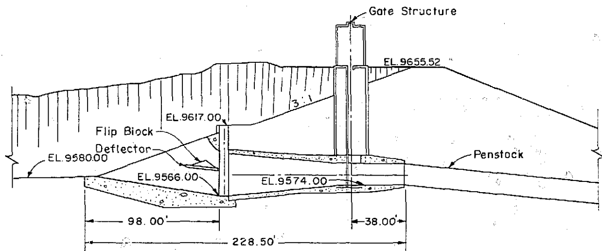
Figure 7. Final inlet-outlet structure.
