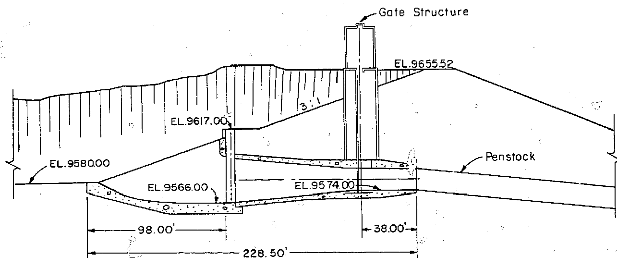
Figure 5. Preliminary inlet-outlet structure.
