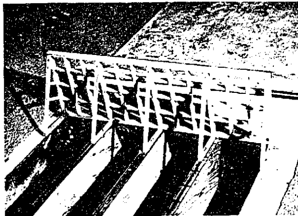
Figure 13. Lattice wall vortex suppressor. Photo PX-D-70837
