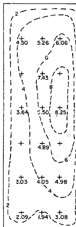
STOP LOG SECTION VELOCITY DISTRIBUTION LOOKING IN DIRECTION OF PUMPED FLOW
