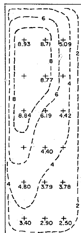
STOP LOG SECTION VELOCITY DISTRIBUTION LOOKING IN DIRECTION OF PUMPED FLOW
