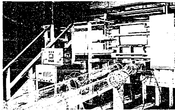
Figure 3. 1:23.23 scale model penstocks. Photo PX-D-70819
