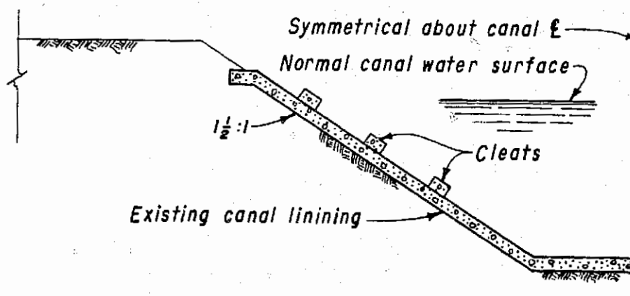
Figure 8. Other proposed canal escape solutions.
