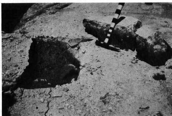
(a) Sample No. 1. Typical of best soil-cement. Photo P800-D-68968
