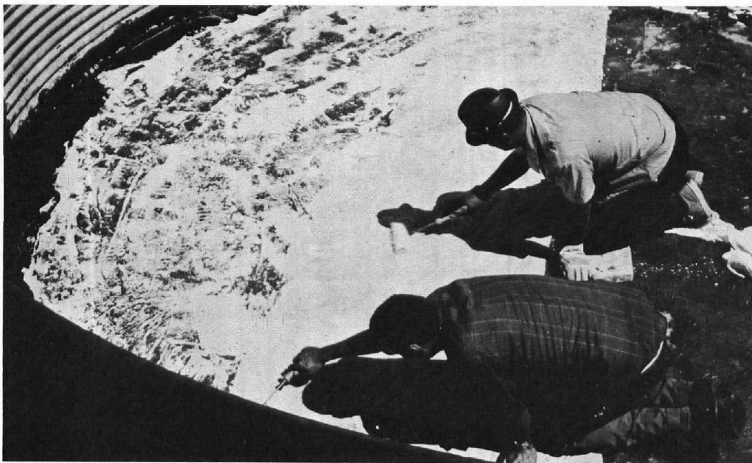
(a) Application of B-5800 to form a residual vinyl plastic film. The material was applied as a concentrated mixture, 3 parts B-5800 to 1 part water, in two equal applications at a total rate of 0.4 gsy ( 1.8 \text{ l/m}^2 ). Photo P800-D-68963
