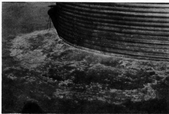
Photograph 13. Saturation condition around test tank containing natural, untreated soil. Such a condition will reduce seepage. Photo P800-D-68979
