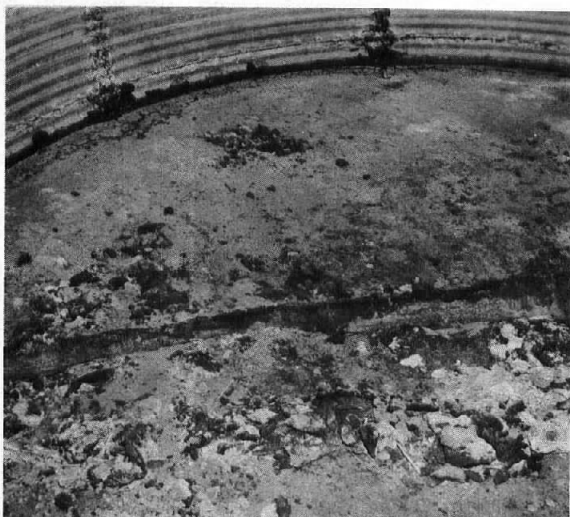
(a) Overall view. Photo P800-D-68971
