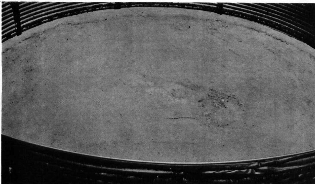
(a) View of completed soil lining containing sealant B-6166 in dry condition. Photo P800-D-68966
