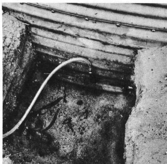
Photograph 8. Plastic tube installed in tank to detect any water pressure that might develop in sand drainage layer. Photo P800-D-68970
