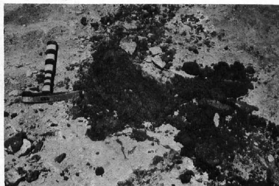
(b) Sample No. 2. Typical of poorest soil-cement. Photo P800-D-68969
