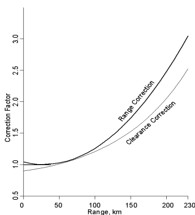
Figure 5.—Range and clearance correction factors as a function of range for the 0.5^\circ -degree beam for old range correction and new clearance correction (both with \alpha = 150 and \beta = 2.0 ).
