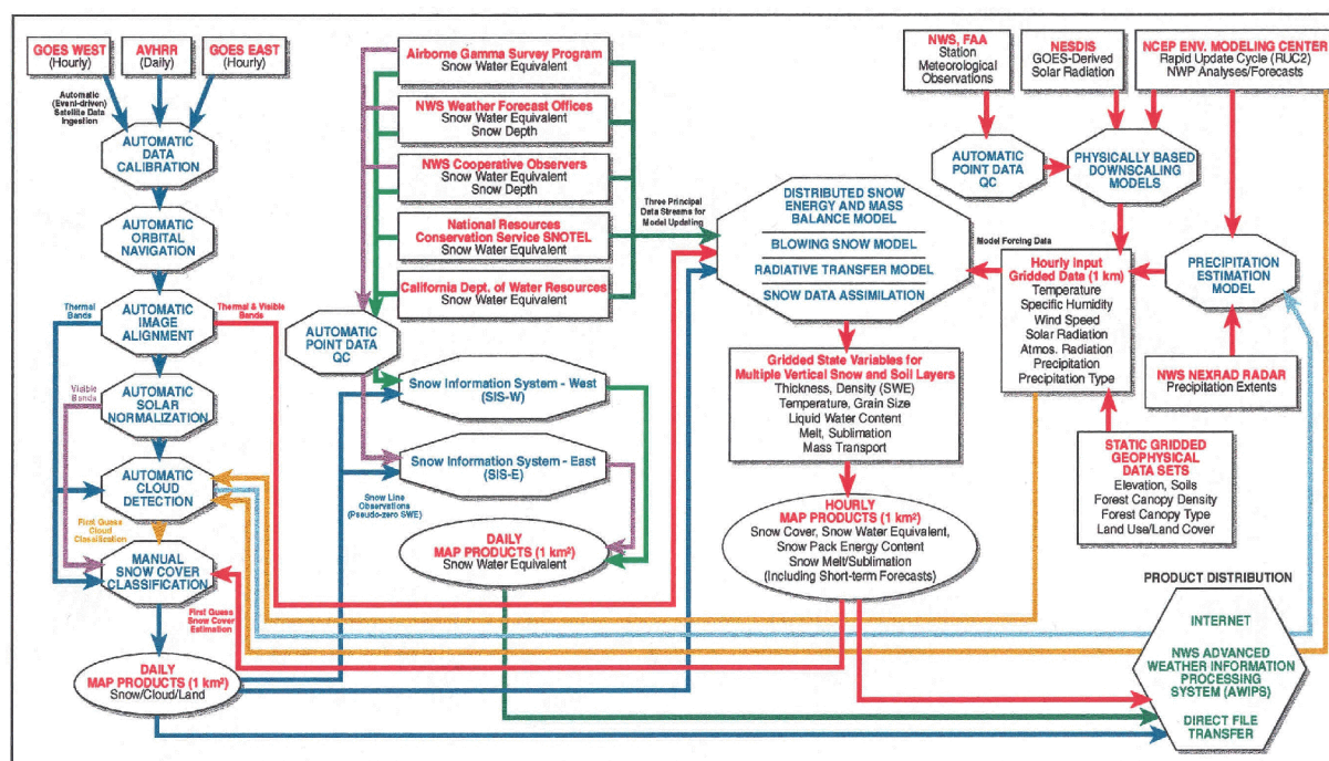
Figure 36.—Flowchart for SNODAS, including model components, data sources, flow, and output.
