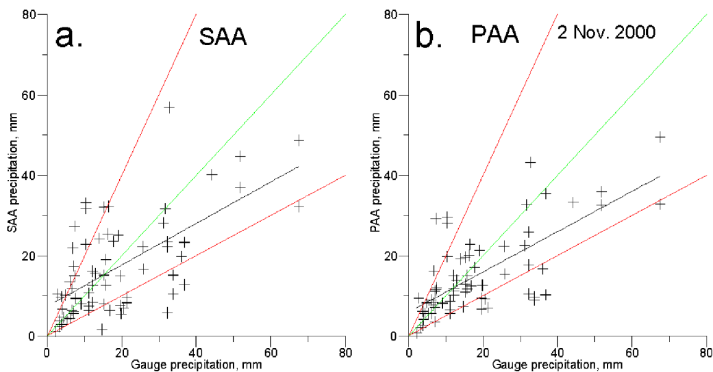
Figure 35.—Relationships of SAA (panel a.) and PAA (panel b.) radar estimates to gauge precipitation G for 24 hours ending 1200 UTC 2 November 2000, for seven radars (KGGW, KMBX, KVMX, KUDX, KBIS, KDLH, KMPX). Green and red lines denote the 1:1 ratio and a factor of two spread from that ratio, respectively. Black line is least squares fit to points.
