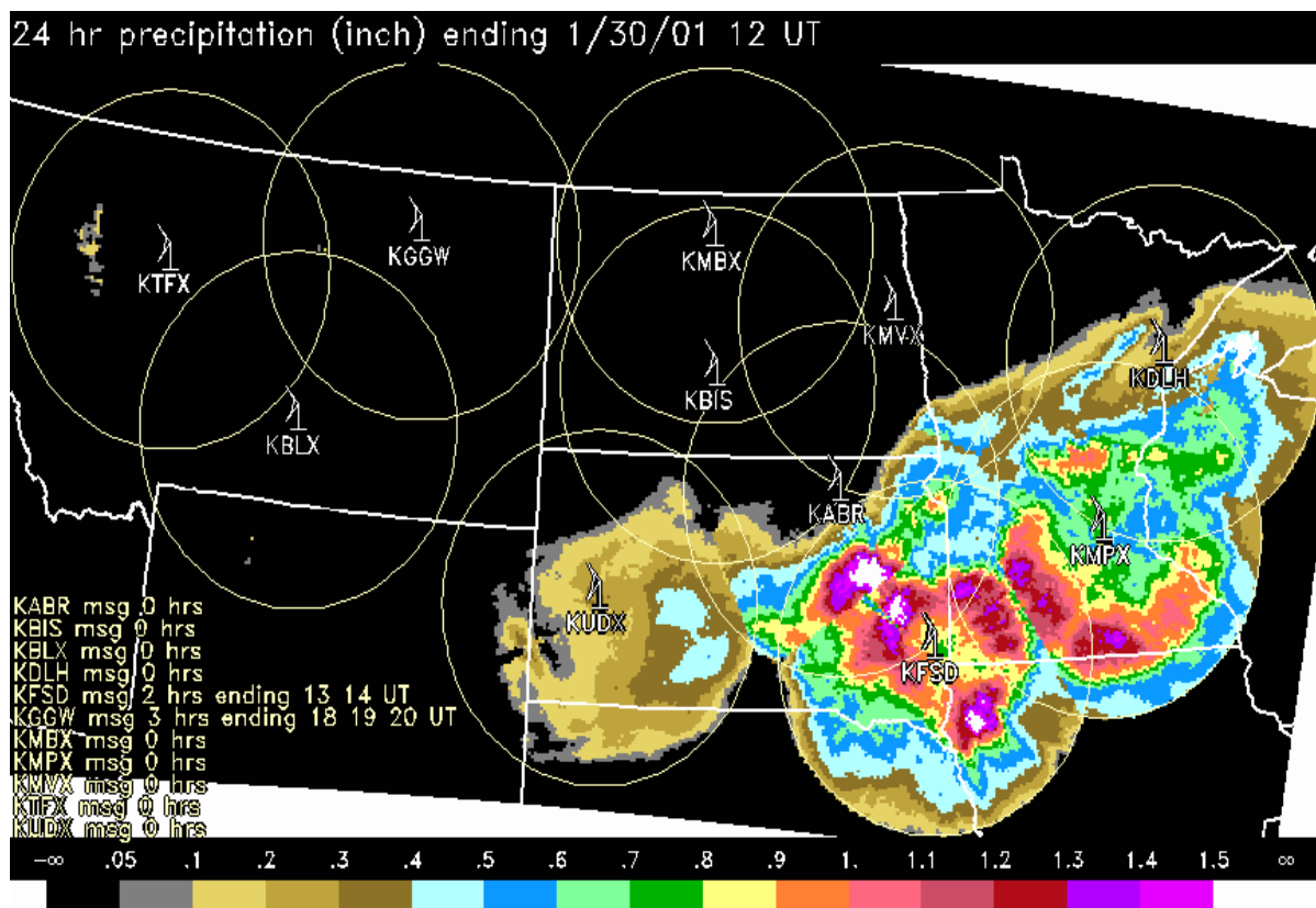
Figure 29.—SAA mosaic for ending time 1200 UTC 30 January 2001.
