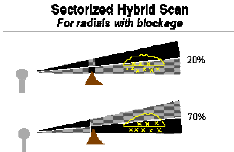
Figure 3.—Examples of hybrid scan and its possible effect on S . Top shows small amount (20%) of blockage of lowest beam so that data is still gathered beyond the blockage (checkerboard beam). Bottom shows large amount (70%) of blockage of the lowest beam so that data are no longer collected from that beam (black beam) but rather the next beam above. Yellow outline and Xs connote shallow cloud and snow particles, respectively.
