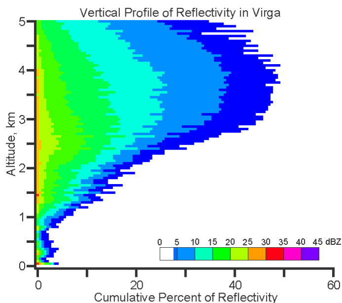
Figure 11.—Diagram of cumulative percentage of range bins exceeding a dBz value specified by color bar versus altitude above radar, for a typical virga situation.
