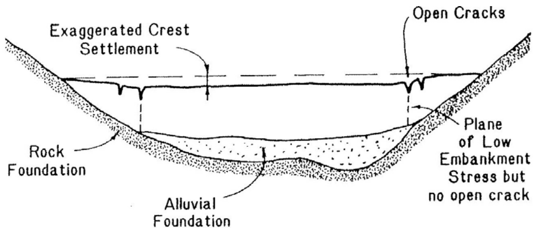
Figure 6. – Example of Dam Cracking from Differential Settlement (Sherard).
