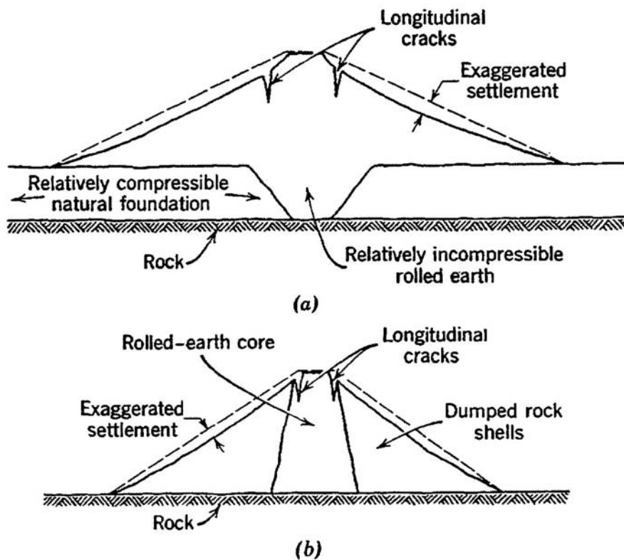
Figure 1B. – Longitudinal cracks. (a) Cracking caused by differential foundation settlement. (b) Cracking caused by differential settlement between embankment sections of dumped rock and rolled earth.
