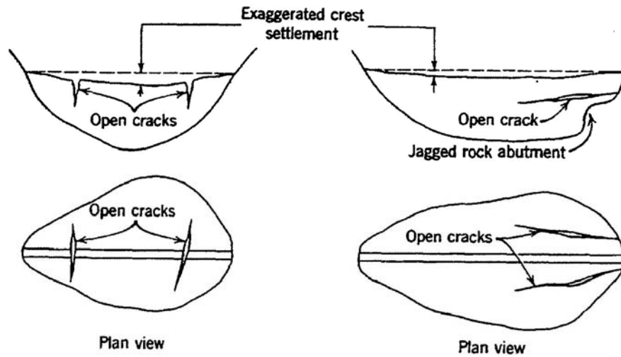
Figure 1A. – Typical transverse differential settlement cracks
