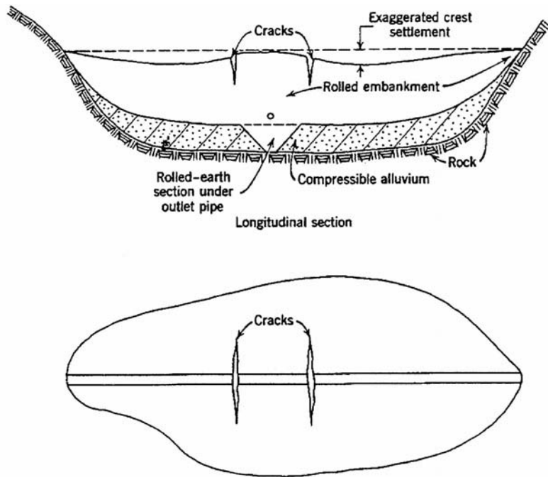
Figure 2A. – Cracking due to differential settlement between natural foundation soil and rolled-earth support under outlet pipe (or other discontinuity in the foundation).
