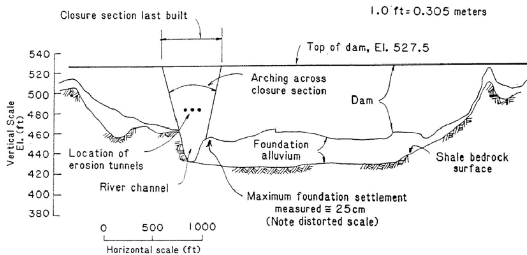
Figure 4. – Examples of Cracking Along a River Channel (Sherard).
