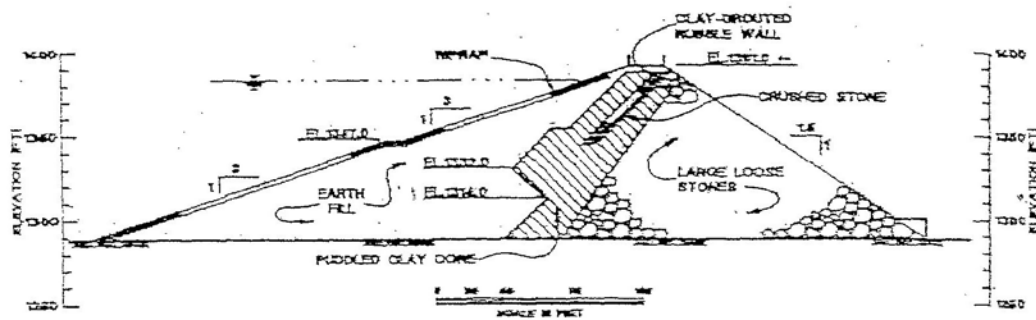
Archives Cross Section of Elmer Thomas Dam
