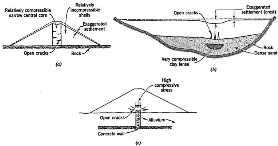
Figure 2B. – Internal embankment cracking.
