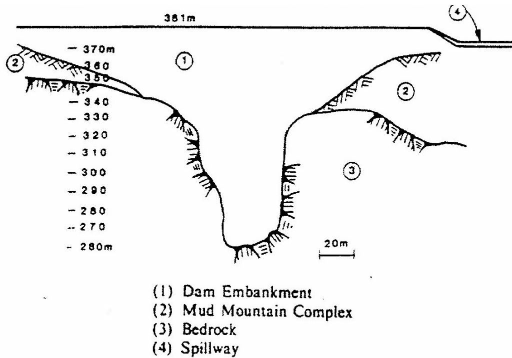
Mud Mountain Dam – Valley cross section (Graybeal 1988).
