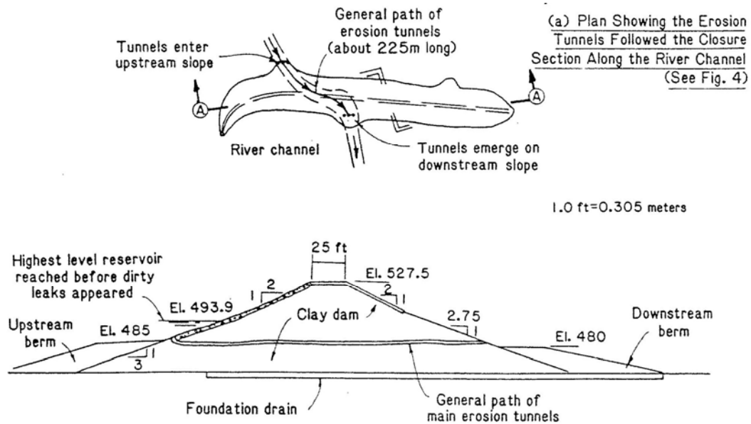
Figure 5. – Example of Dam Cracking Along a River Channel - (Sherard).
