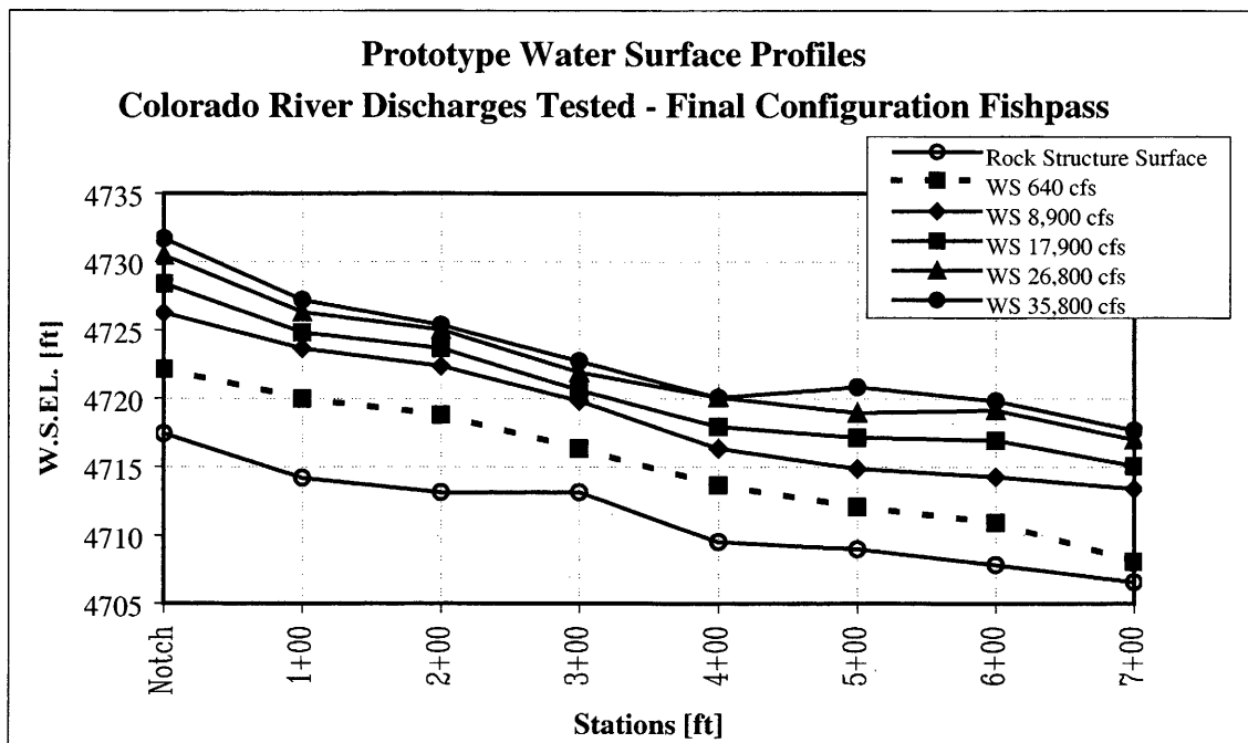
Figure 9. - Prototype water surface profiles for configuration 3 as obtained from physical model.
