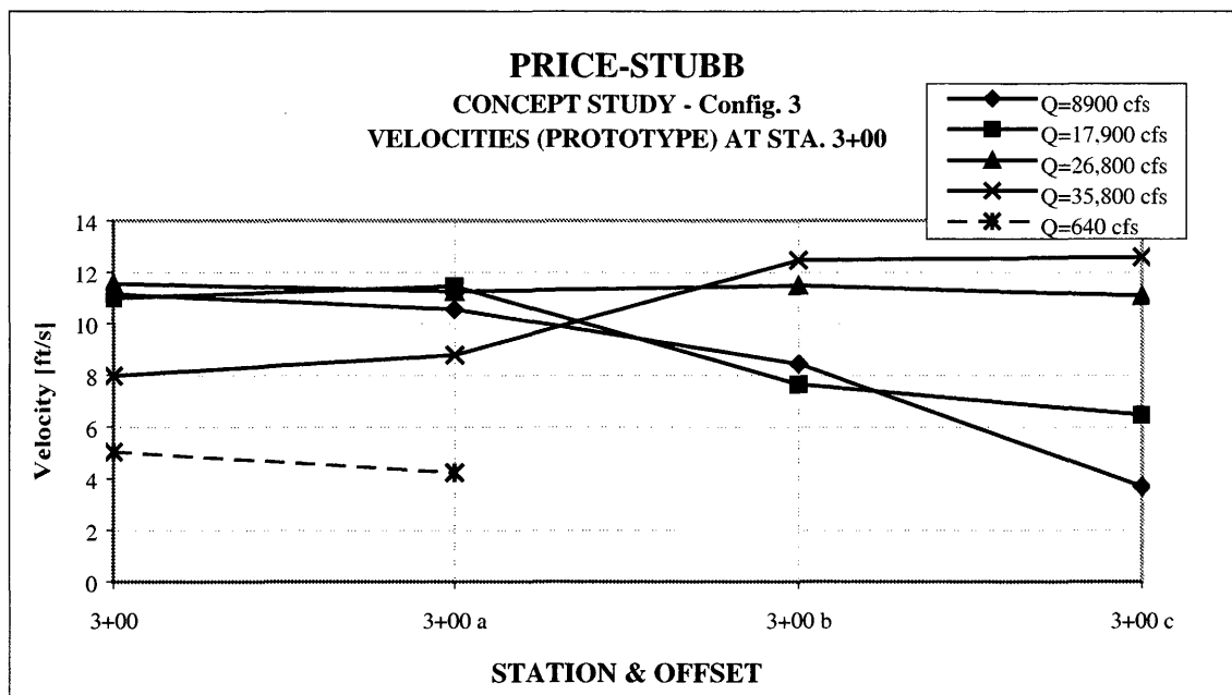
Figure 13. - Mid-depth lateral velocity distributions (looking upstream) at STA 3+00 for Colorado River discharges tested.
