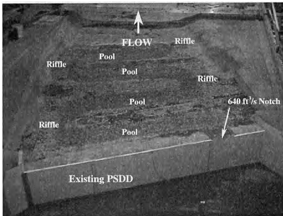
Figure 5. - Configuration 2: 400-foot rock-ramp structure with low-flow notch in diversion dam and riffle-pool substructure.
