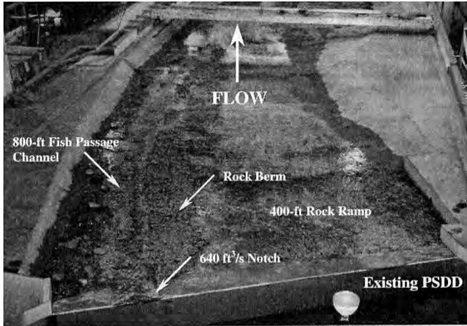
Figure 6. - Configuration 3: 800-foot (1.5 percent slope) fish passage channel along the left bank and a low-flow notch and 400-foot (3.0 percent slope) lateral rock-ramp structure.
