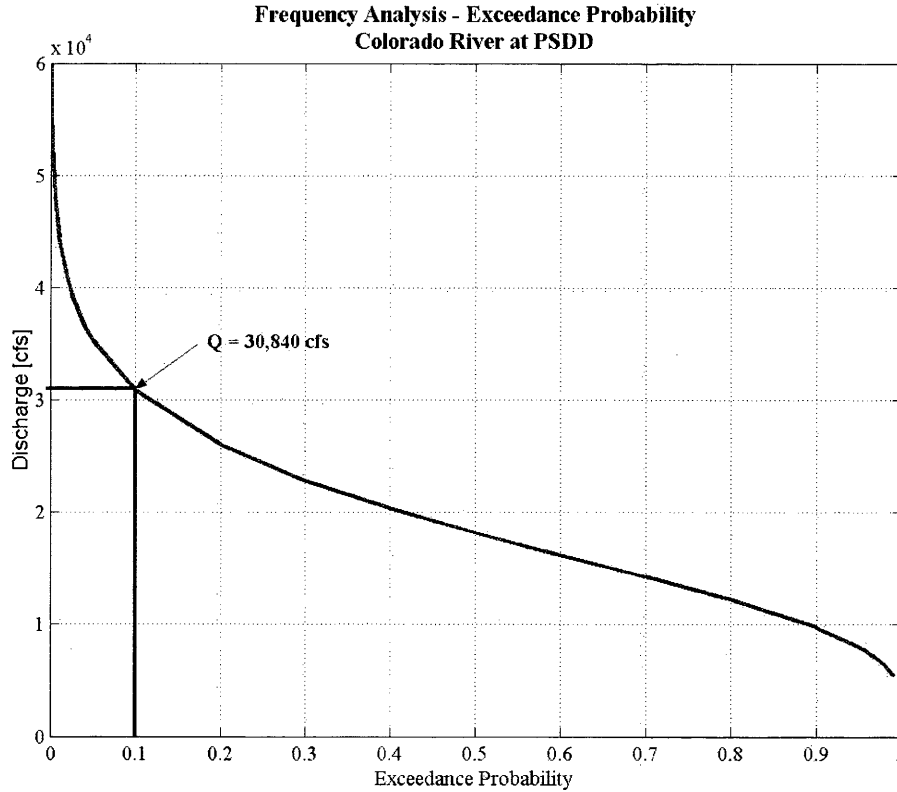
Figure 2. - Frequency analysis for the Colorado River at PSDD showing 10 percent exceedence limit discharge of approximately 30,800 ft 3 /s.
