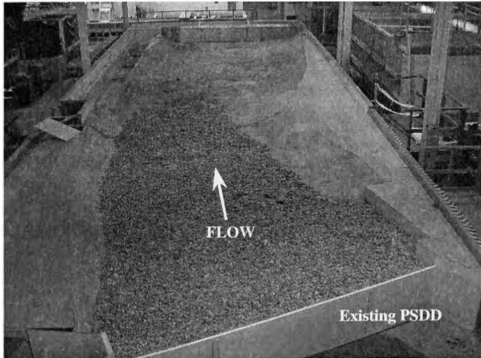
Figure 4. - Configuration 1: 800-foot rock-ramp structure constructed on a 2.0 percent slope.
