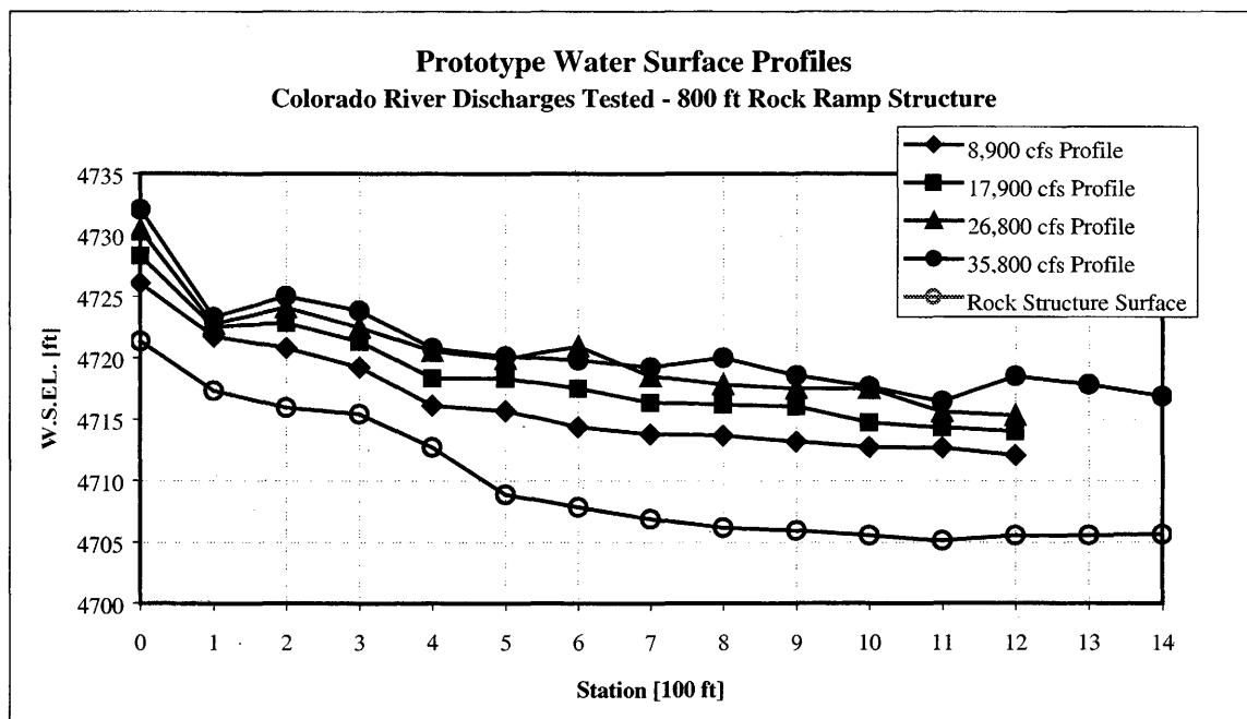
Figure 7. - Prototype water surface profiles for the 800-foot rock-ramp structure (configuration 1) obtained from the physical model study.
