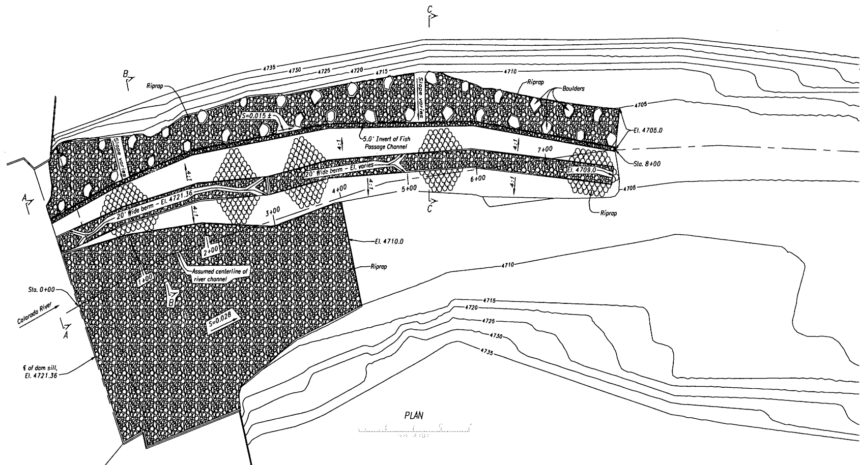
Figure 19. - Recommended configuration (configuration 3) plan view conceptual layout.
