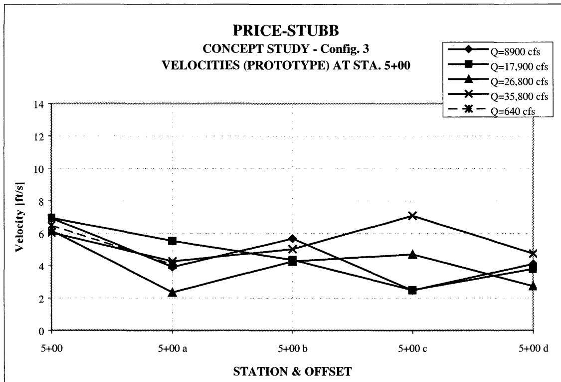
Figure 15. - Mid-depth lateral velocity distributions (looking upstream) at STA 5+00 for Colorado River discharges tested.
