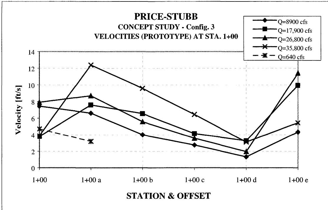
Figure 11. - Mid-depth lateral velocity distributions (looking upstream) at STA 1+00 for Colorado River discharges tested.
