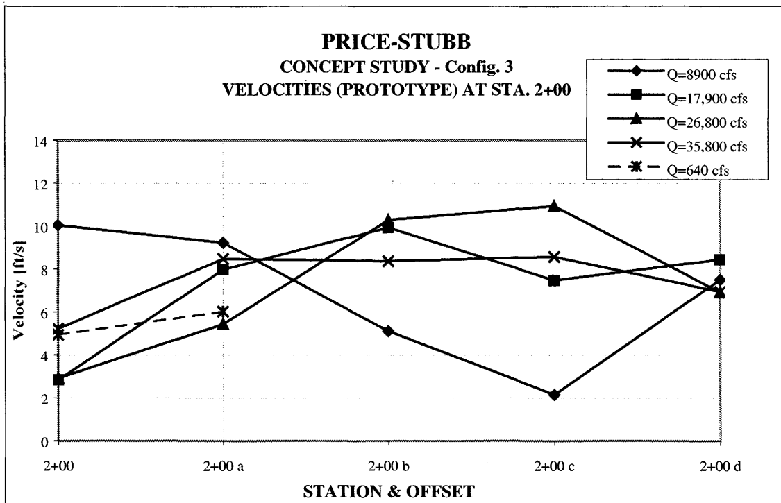
Figure 12. - Mid-depth lateral velocity distributions (looking upstream) at STA 2+00 for Colorado River discharges tested.
