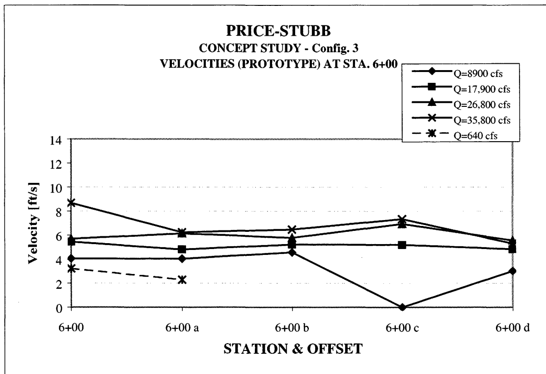
Figure 16. - Mid-depth lateral velocity distributions (looking upstream) at STA 6+00 for Colorado River discharges tested.
