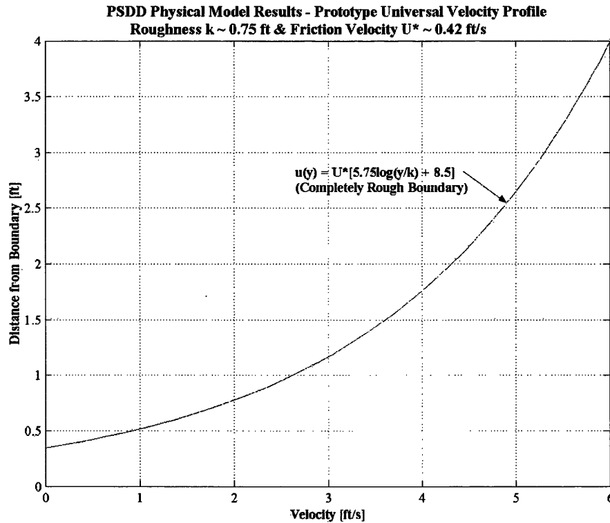
Figure 18. - Universal velocity profile (completely rough boundary). Friction velocity, U^* , was obtained from model data and roughness taken for proposed rock size ( D_{50} = 16 in).
