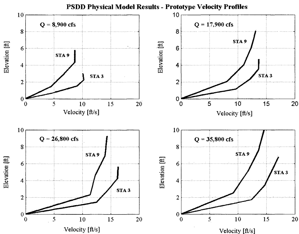
Figure 8. - Prototype velocity profiles (velocity versus distance above bed elevation) for the 800-foot rock-ramp structure for various Colorado River discharges tested.
