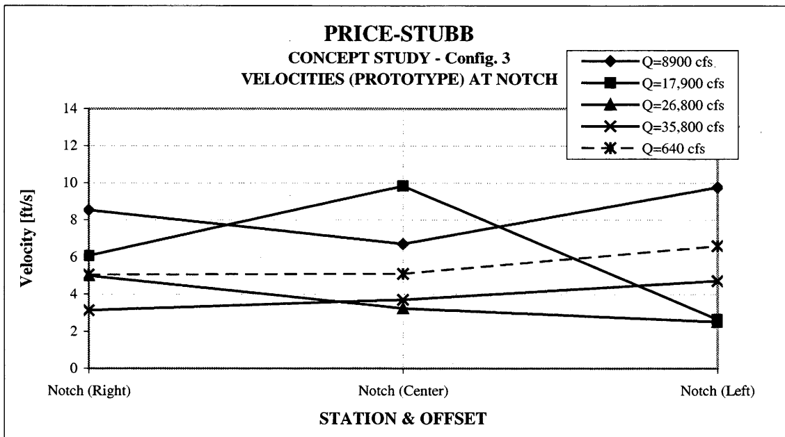
Figure 10. - Mid-depth lateral velocity distributions (looking upstream) at notch (fish passage channel exit) for Colorado River discharges tested.
