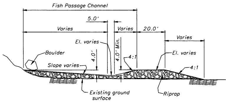
Figure 20. - Recommended configuration sections along fish passage structure reach downstream from PSDD.
