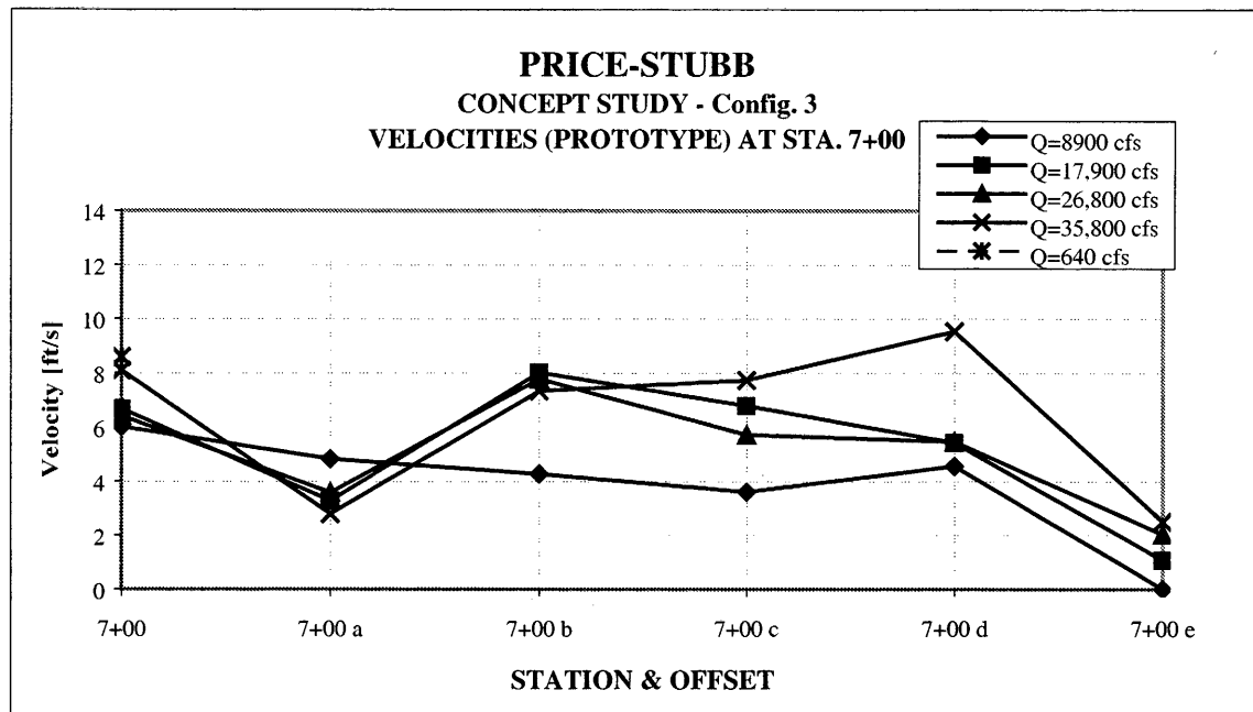
Figure 17. - Mid-depth lateral velocity distributions (looking upstream) at STA 7+00 for Colorado River discharges tested.
