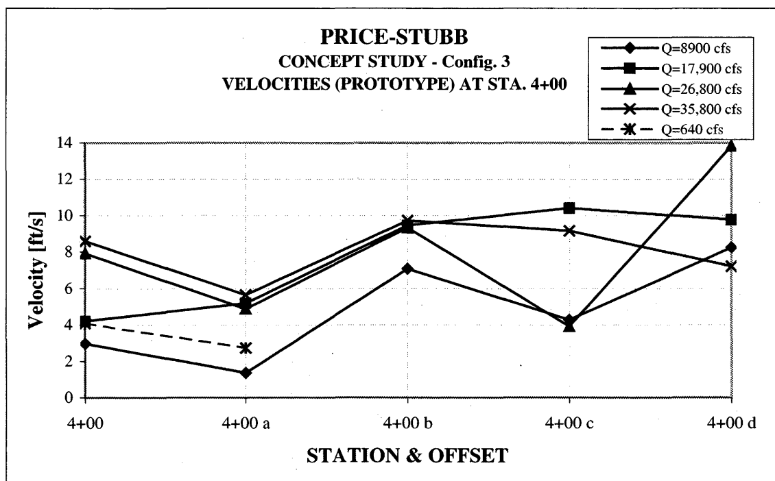
Figure 14. - Mid-depth lateral velocity distributions (looking upstream) at STA 4+00 for Colorado River discharges tested.
