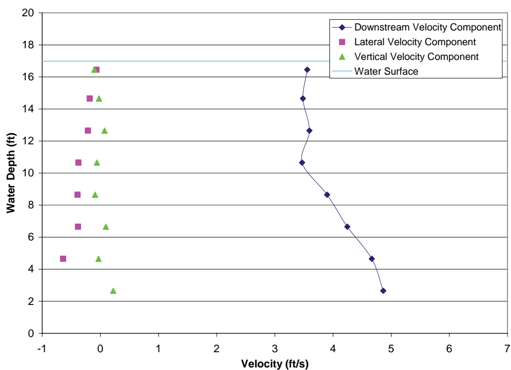
FIGURE A2-9.—Test 3-1, bypass 1 intake profile with all bypasses open, measured bypass ratio = 0.98, bypass ratio with facility instruments = 1.27, outgoing tide, water depth = 16.98 ft, trashrack differential = 0.94 ft, louvers differential = 0.45 ft.
