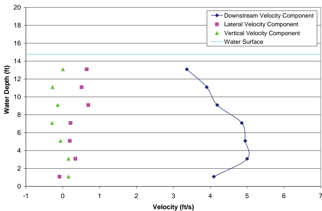
FIGURE A1-1.—Test 1A, bypass 1 intake profile with all bypasses open, measured bypass ratio = N/A, bypass ratio with facility instruments = N/A, incoming tide, water depth = 14.75 ft, recently cleaned trashrack and louvers.
