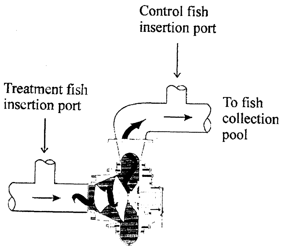
Figure 4. Cross section view of the Hidrostal pump and fish injection ports (fish protective impeller shroud is not shown in this drawing).
