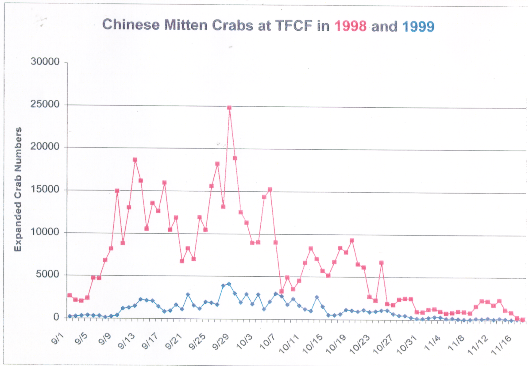
Figure 5. Daily comparison of 1998 and 1999 estimated mitten crab entrainment at the Tracy Fish Collection Facility, California (Siegfried, personal communication).
