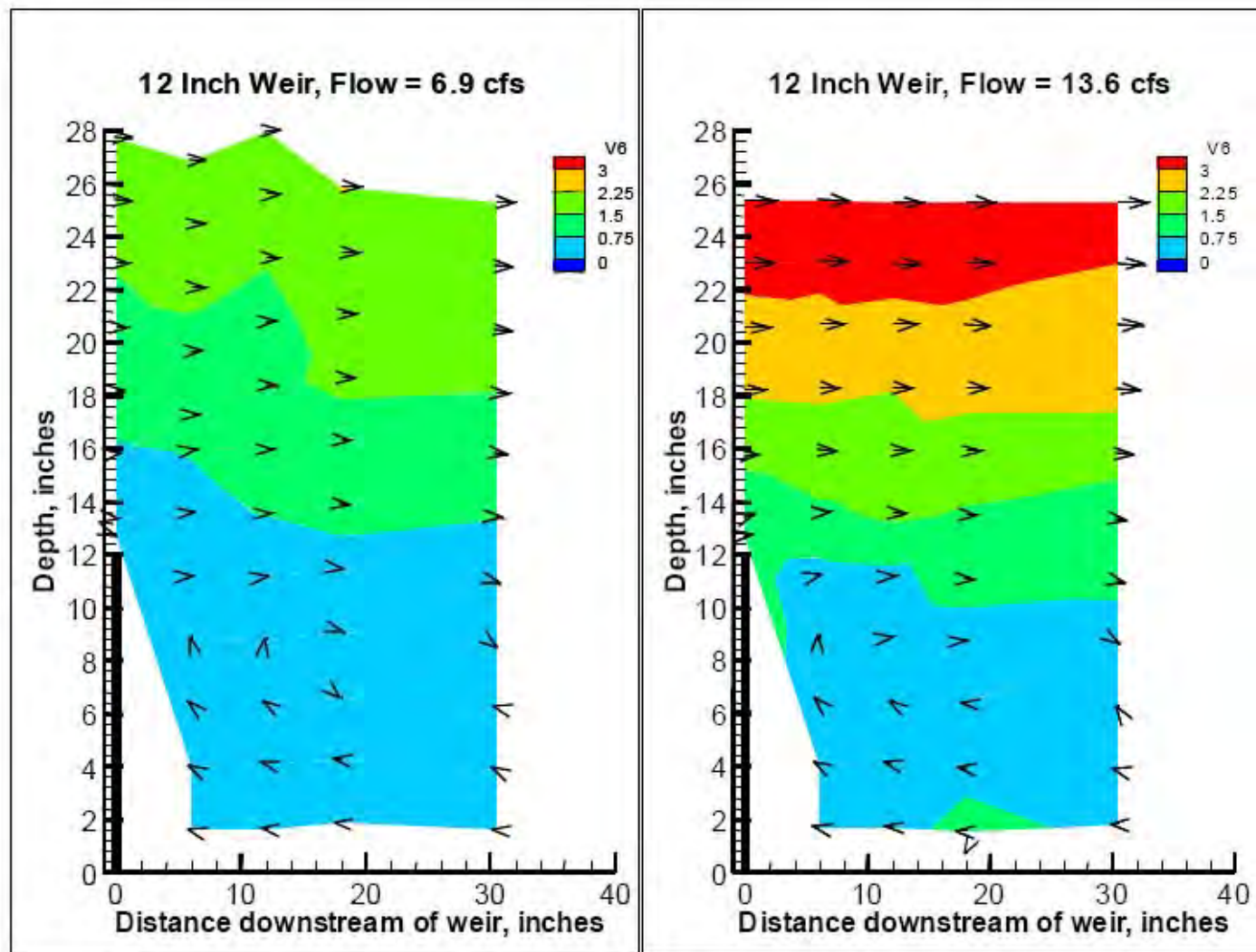
Figure 23 - Elevation view of measured velocity vector field downstream of 12 inch high weir baffles.
