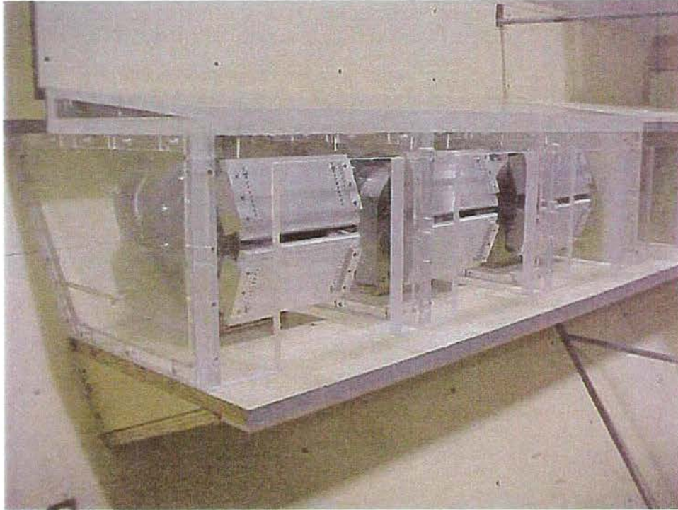
Figure 1. - Photograph of the three 48-in clamshell gates and gate-house structure modeled at a 1:10.667 scale.
