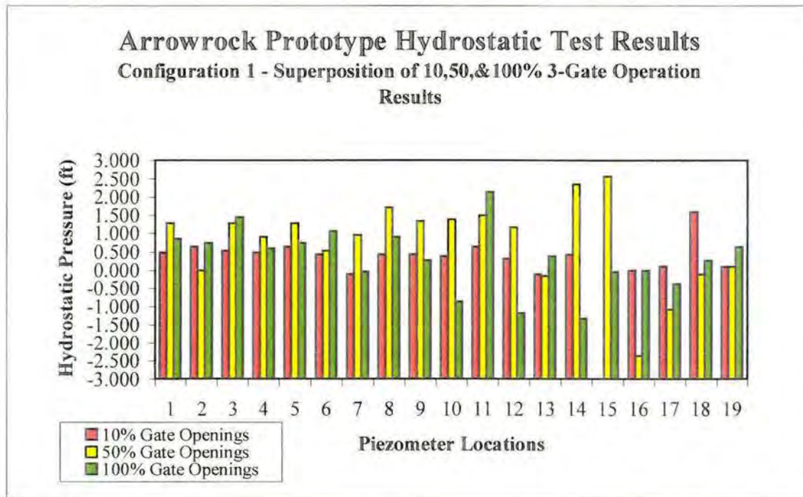
Figure 11. - Combined results plot for configuration 1, 3-gate simultaneous operation at 10, 50, and 100% gate openings.
