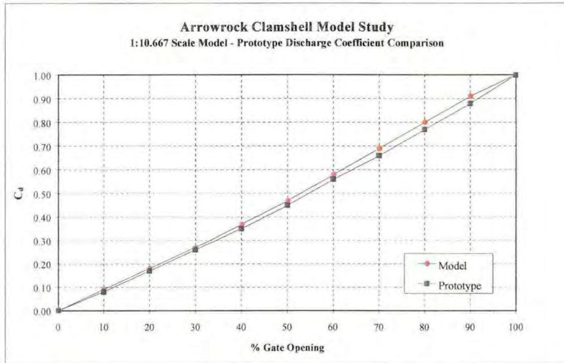
Figure 3. - Comparison between the model slide-gate and prototype clamshell-gate discharge coefficients.
