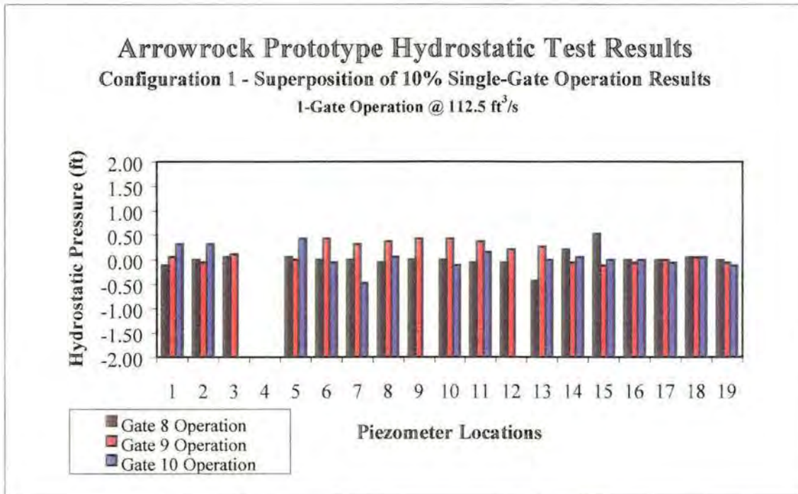
Figure 7. - Superposition of 10% single-gate operation results for configuration 1 demonstrating the local influence of gate operation on hydrostatic pressure differentials.
