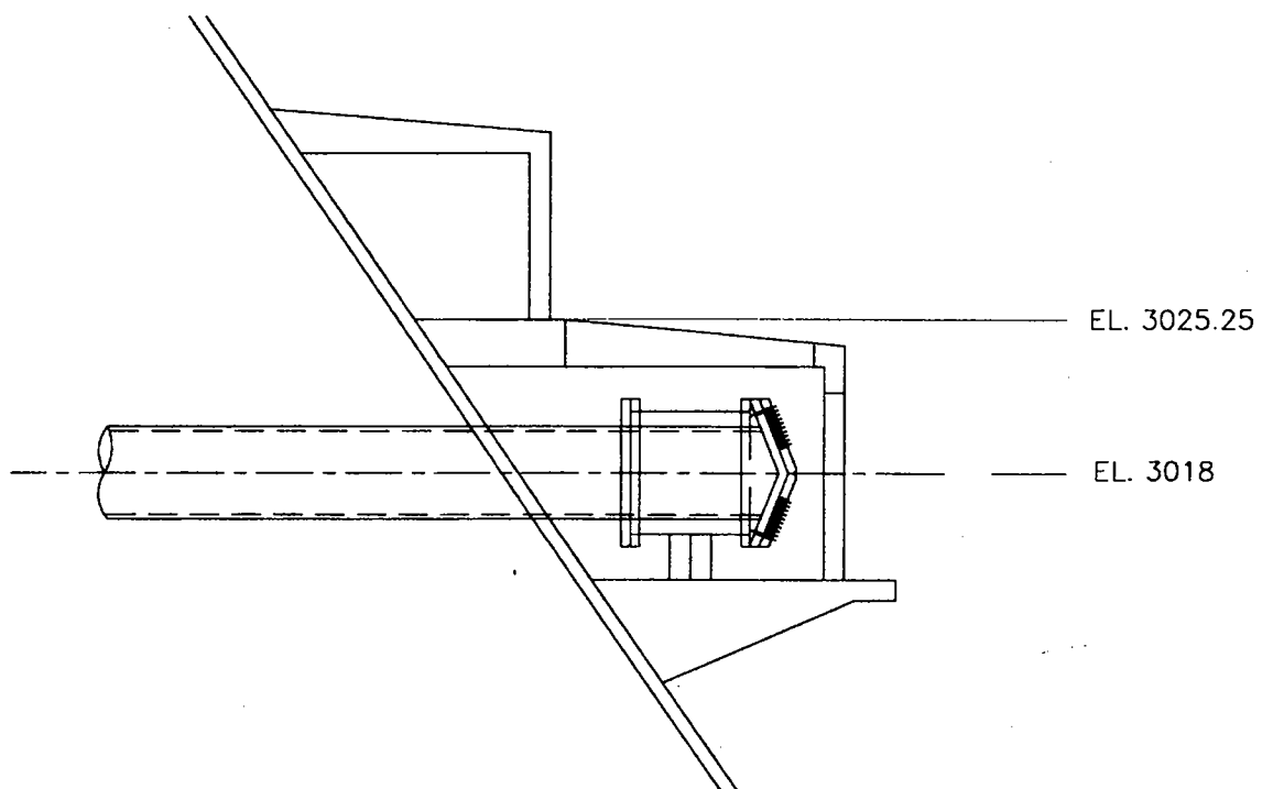
Figure 5. - Configuration 1, gates located back from end of gate-house structure such that gate lips are inside the structure.
