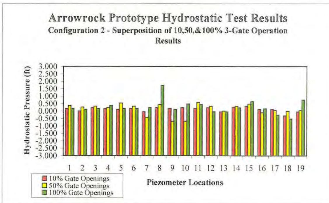
Figure 12. - Combined results plot for configuration 2, 3-gate simultaneous operation at 10, 50, and 100% gate openings.
