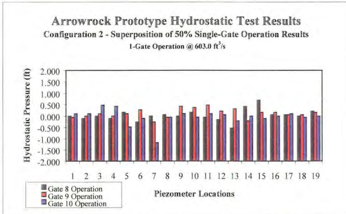
Figure 9. - Superposition of 50% single-gate operation results for configuration 2 illustrating lower overall pressure differentials in comparison with configuration 1, but similar local increased pressure differentials due to gate operation.
