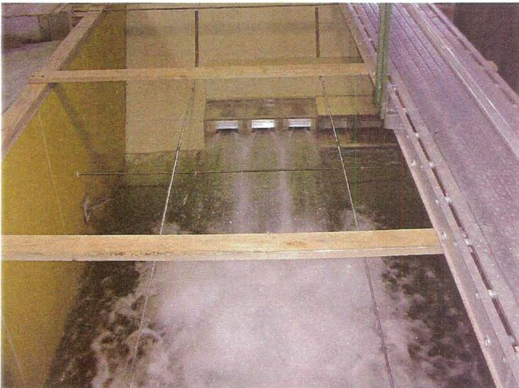
3 gates operated at 50% open in free-discharge mode.
