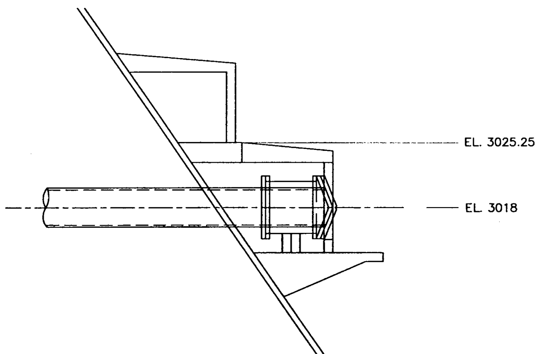
Figure 13. - Configuration 3 (to be evaluated), gates located forward in gate-house (i.e. gate-house structure shortened) such that gate lips are located outside of gate-house structure.
