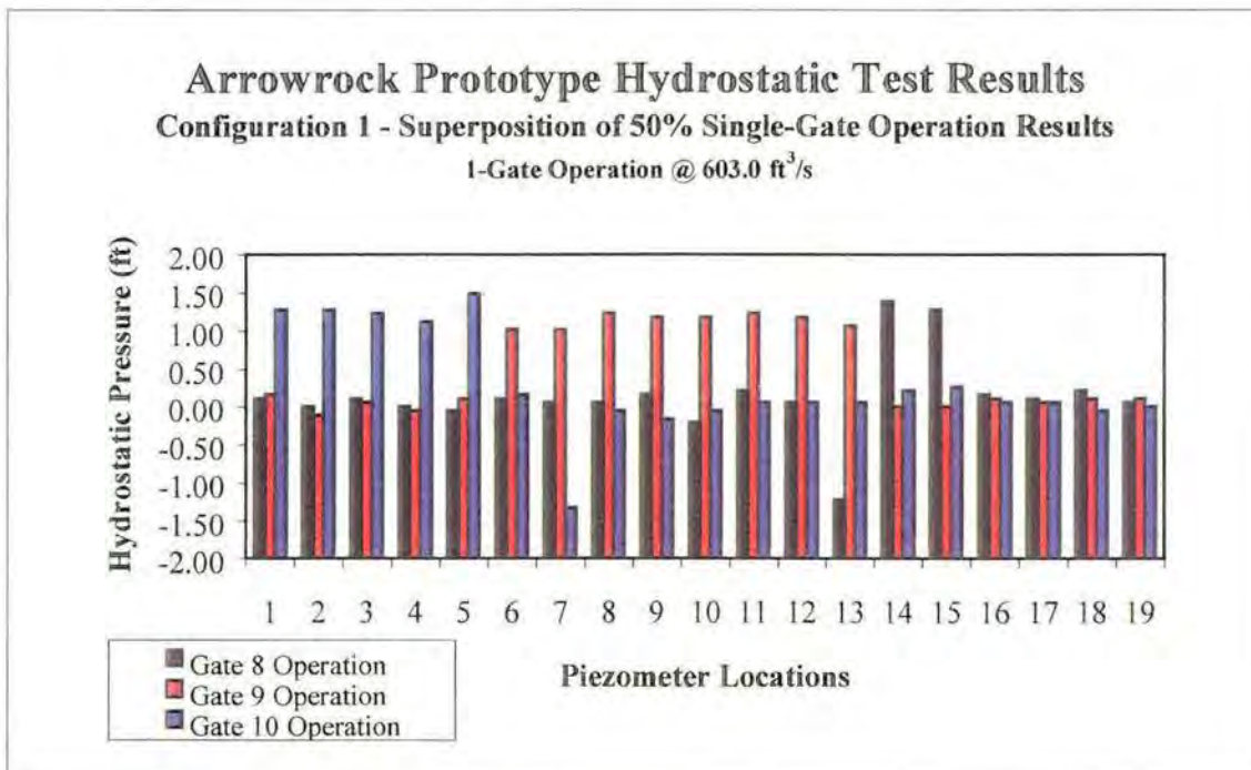
Figure 8. - Superposition of 50% single-gate operation results for configuration 1 also showing local influence of gate operation on hydrostatic pressure differentials.
