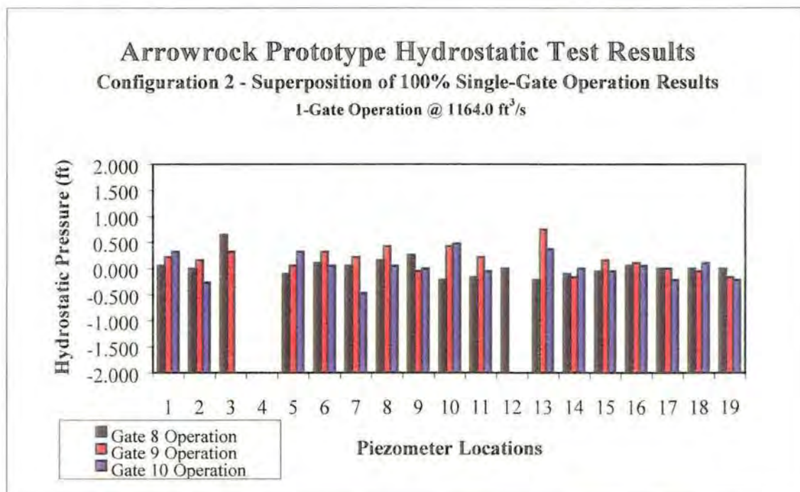
Figure 10. - Superposition of 100% single-gate operation results for configuration 2 showing diminished local pressure increase effect.
