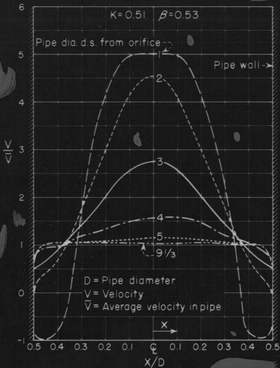
VELOCITY REDISTRIBUTION IN PIPE DOWNSTREAM FROM ORIFICE
