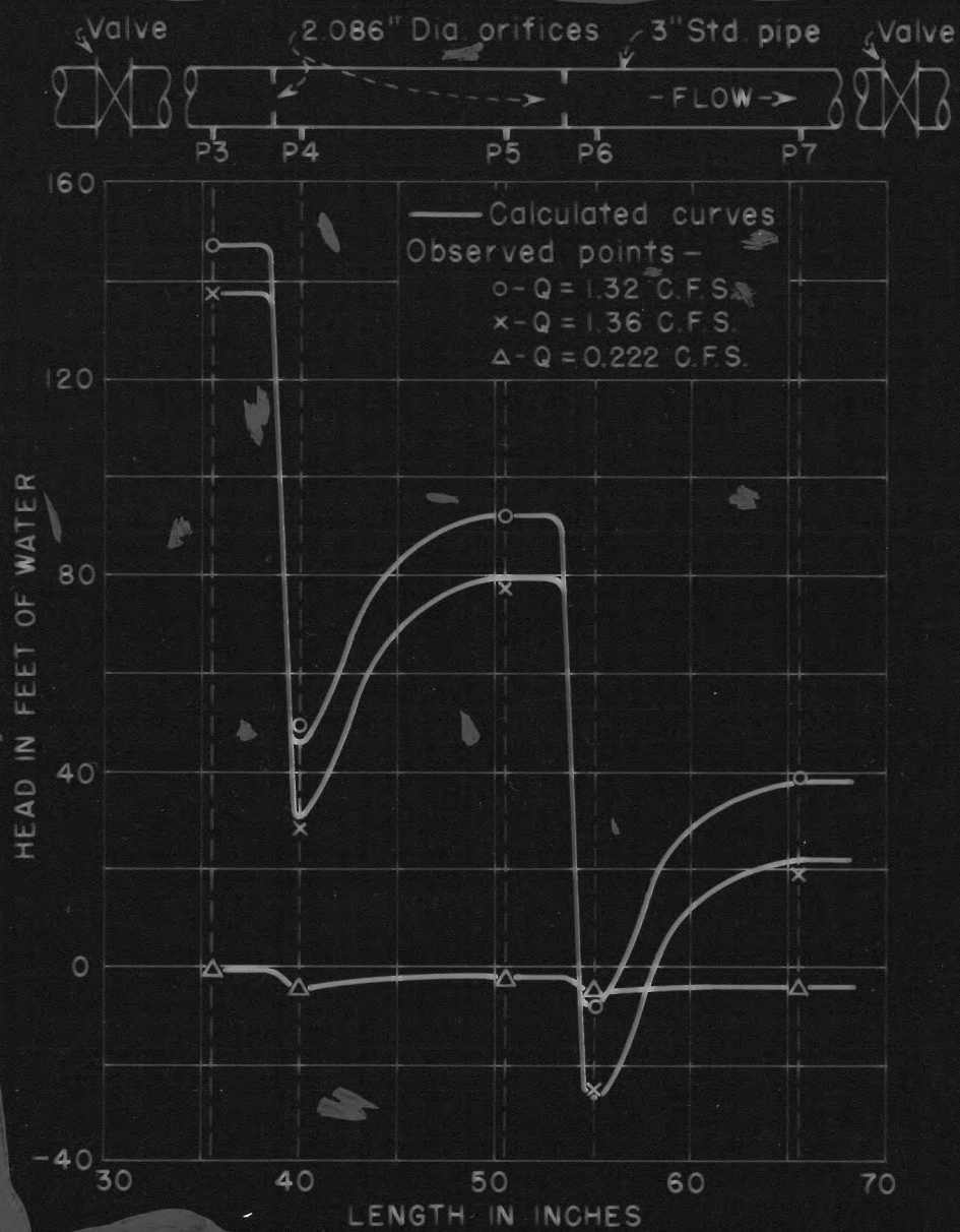
HYDRAULIC GRADIENT FOR ORIFICES IN TANDEM IN PIPELINES
