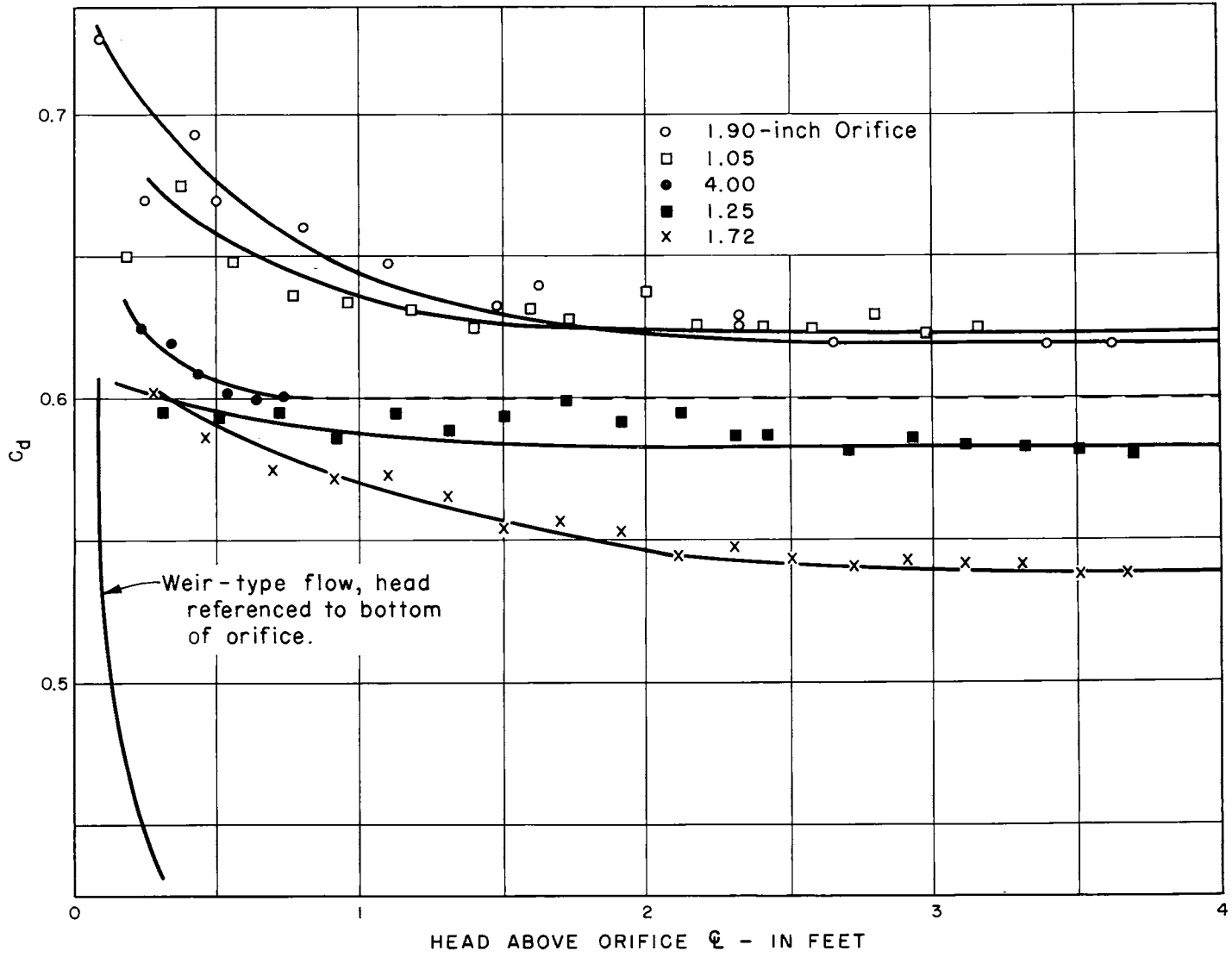
ORIFICES FOR AUTOMATIC SPILLWAY GATE CONTROLS Discharge Coefficients for Orifices in Wall of 10-inch Diameter Pipe
