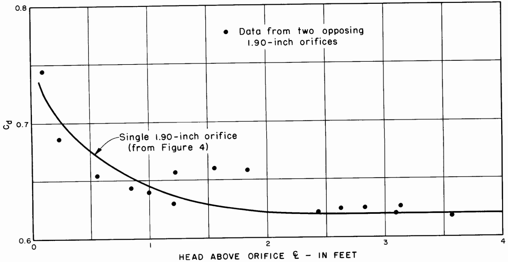
ORIFICES FOR AUTOMATIC SPILLWAY GATE CONTROLS Effect of Opposing Orifices
