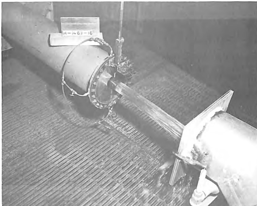
A. Test rig for 3-inch orifice placed concentrically in 10-inch-diameter, 4-foot-long pipe. Photo PX-D-64863
