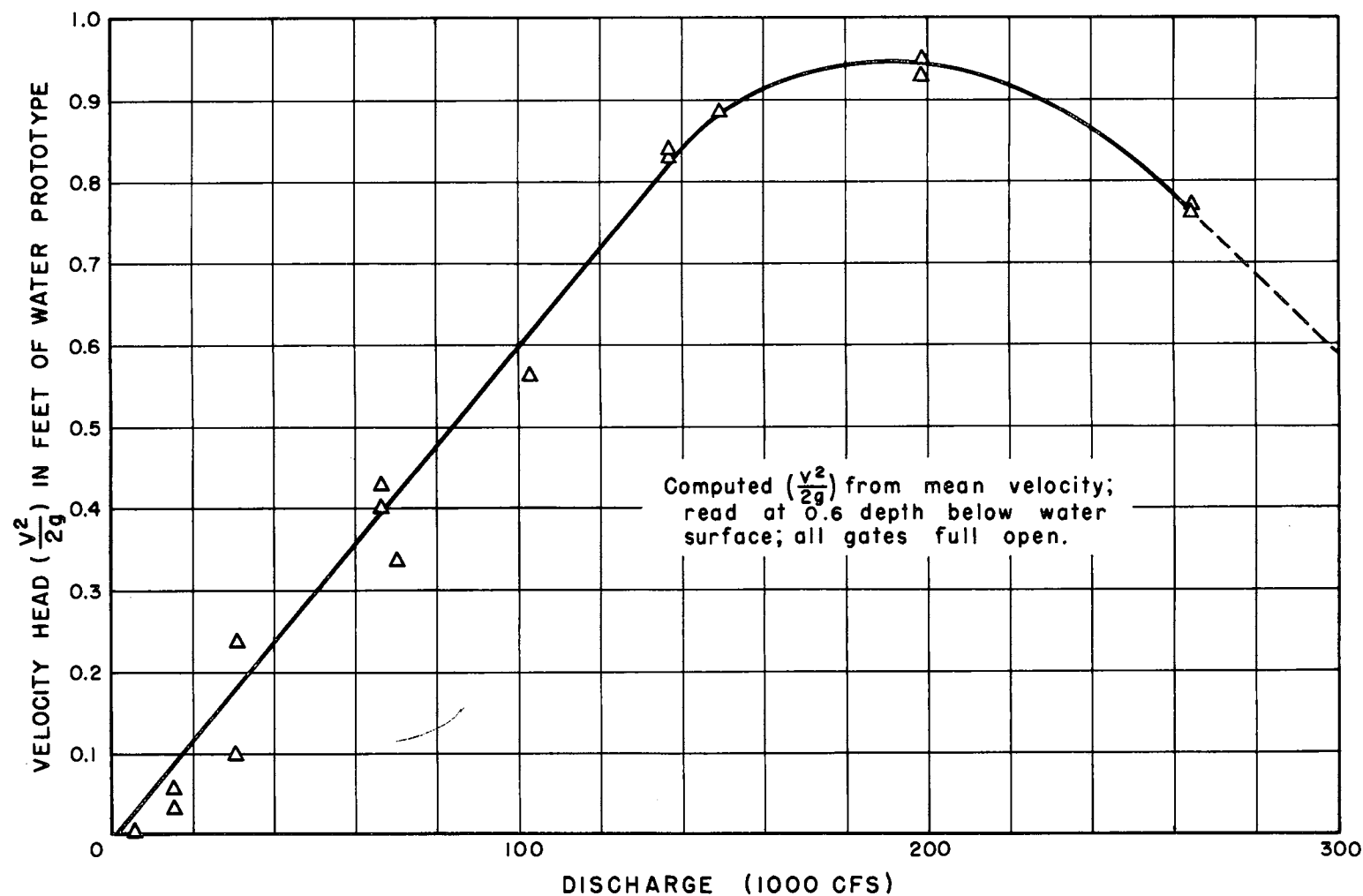
GLEN ELDER DAM SPILLWAY VELOCITY HEAD OVER MODEL STILLING WELL INTAKE FOR FULL OPEN GATES
