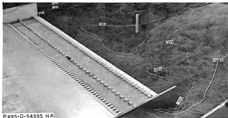
B. After 8 hours (prototype) operation at 264,500 cfs tailwater El. 1431. Erosion pattern similar to preliminary basin
