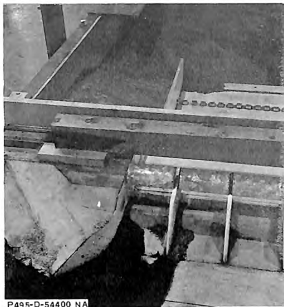
A. Material eroded from the left approach channel side slope and deposited in the low-velocity areas of the two adjacent end bays and at the stilling basin end sill after 264,500 cfs discharge for 4 hours (prototype)
