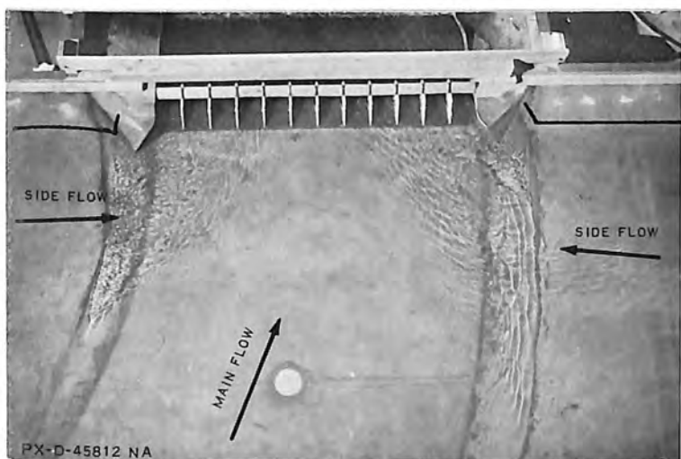
Discharge 264,500 cfs (Maximum) Gates fully opened, Res. W.S. El. 1492.2
