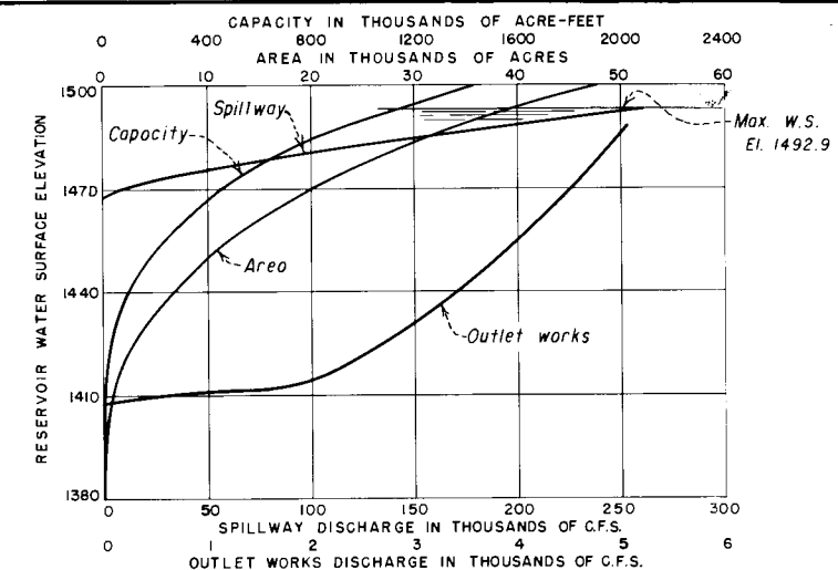
AREA-CAPACITY-DISCHARGE CURVES
