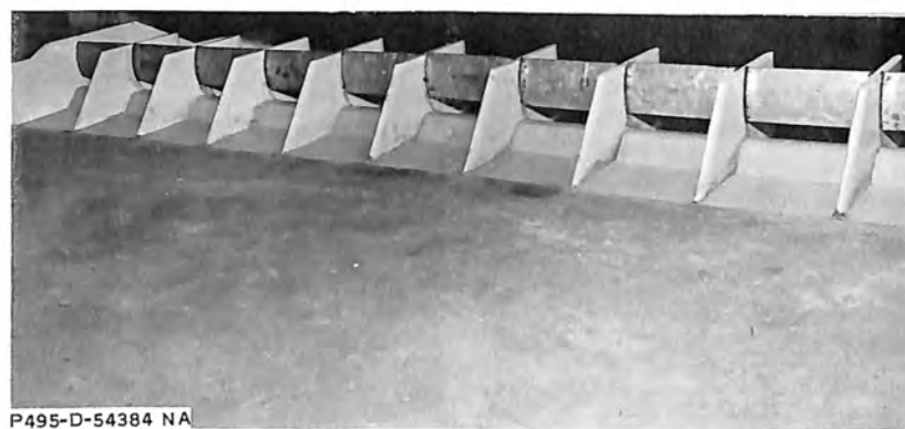
The approach channel showing 10 of the 12 spillway bays
