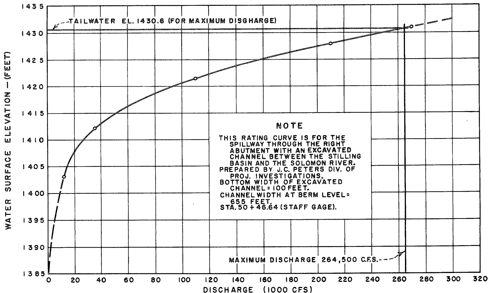
GLEN ELDER DAM SPILLWAY TAILWATER RATING CURVE (AT UPSTREAM END OF EXCAVATED CHANNEL)
