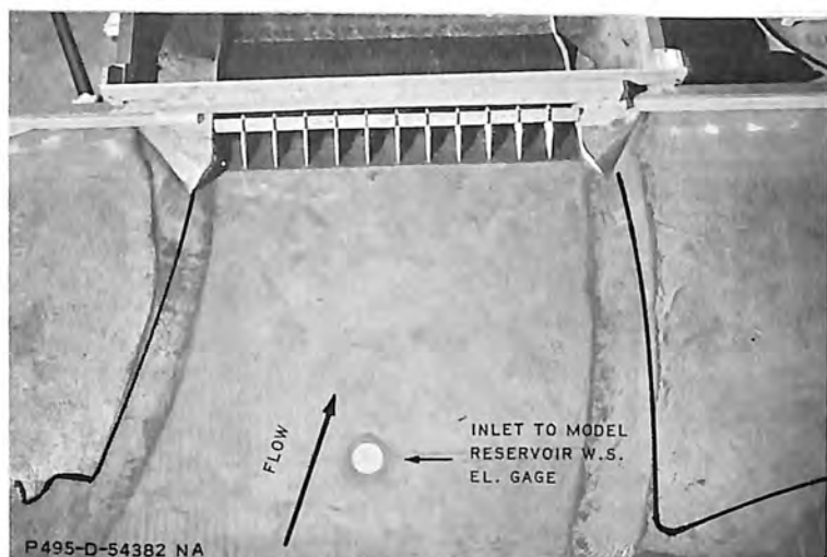
Discharge 66,125 cfs (25% of maximum) Gates fully opened, Res. W.S. El. 1477.3
