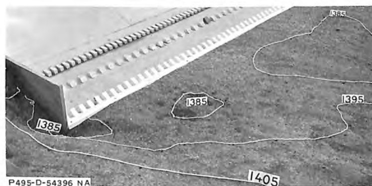
C. Closeup of erosion at the end of the basin training wall
