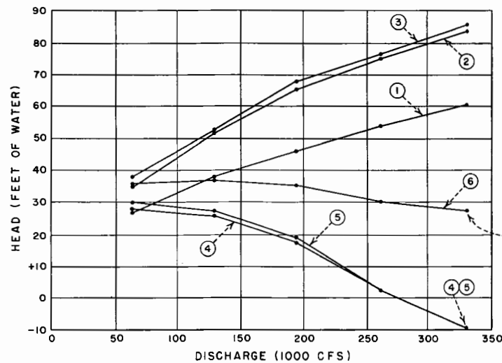
A. Average pressures read from water manometers
