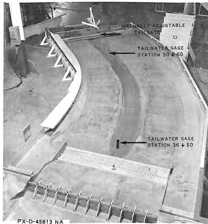
View facing downstream
