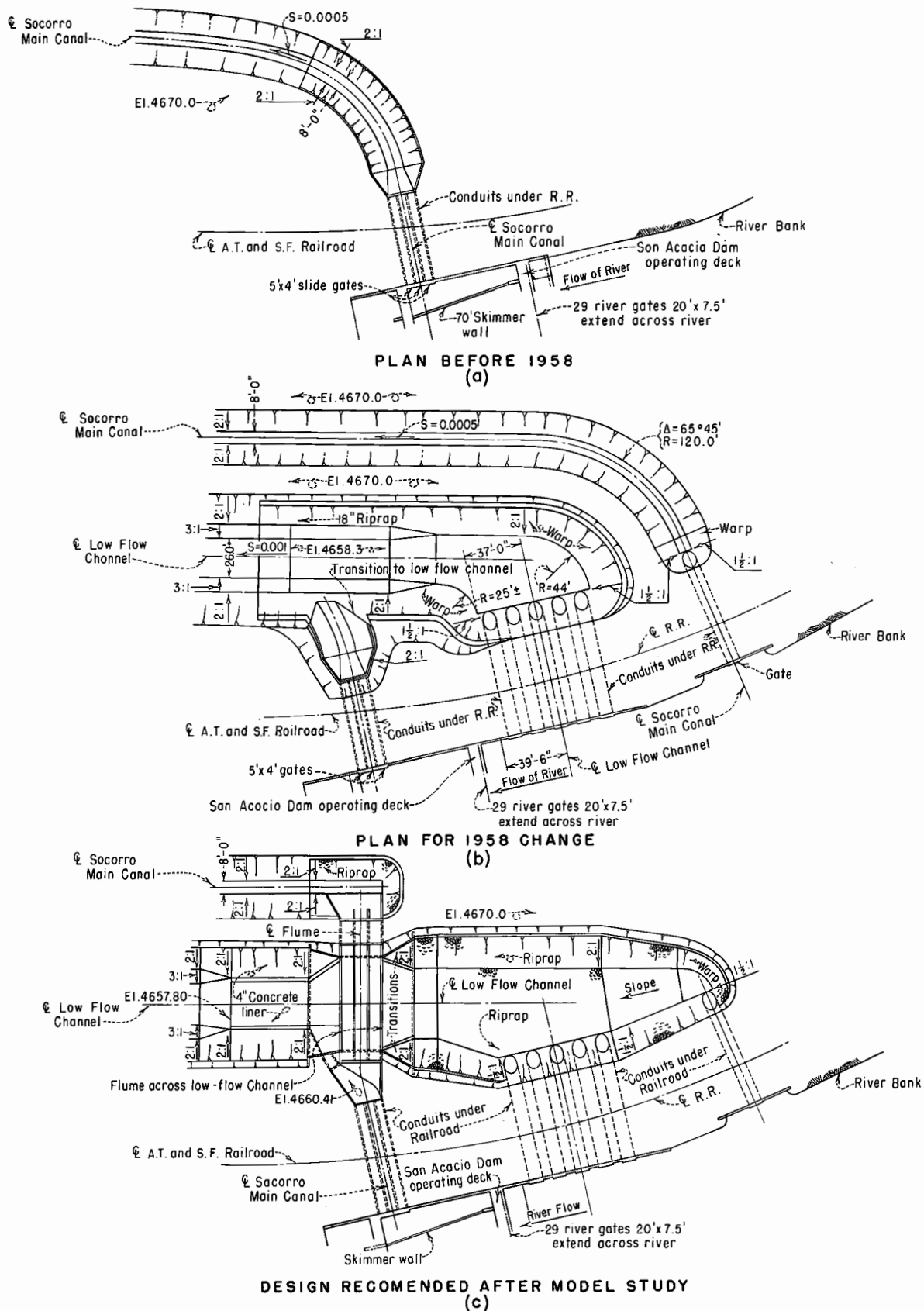
MIDDLE RIO GRANDE PROJECT NEW MEXICO SAN ACACIA DIVERSION DAM PLANS OF HEADWORKS AT DIVERSION DAM 1:20 HYDRAULIC MODEL STUDY
