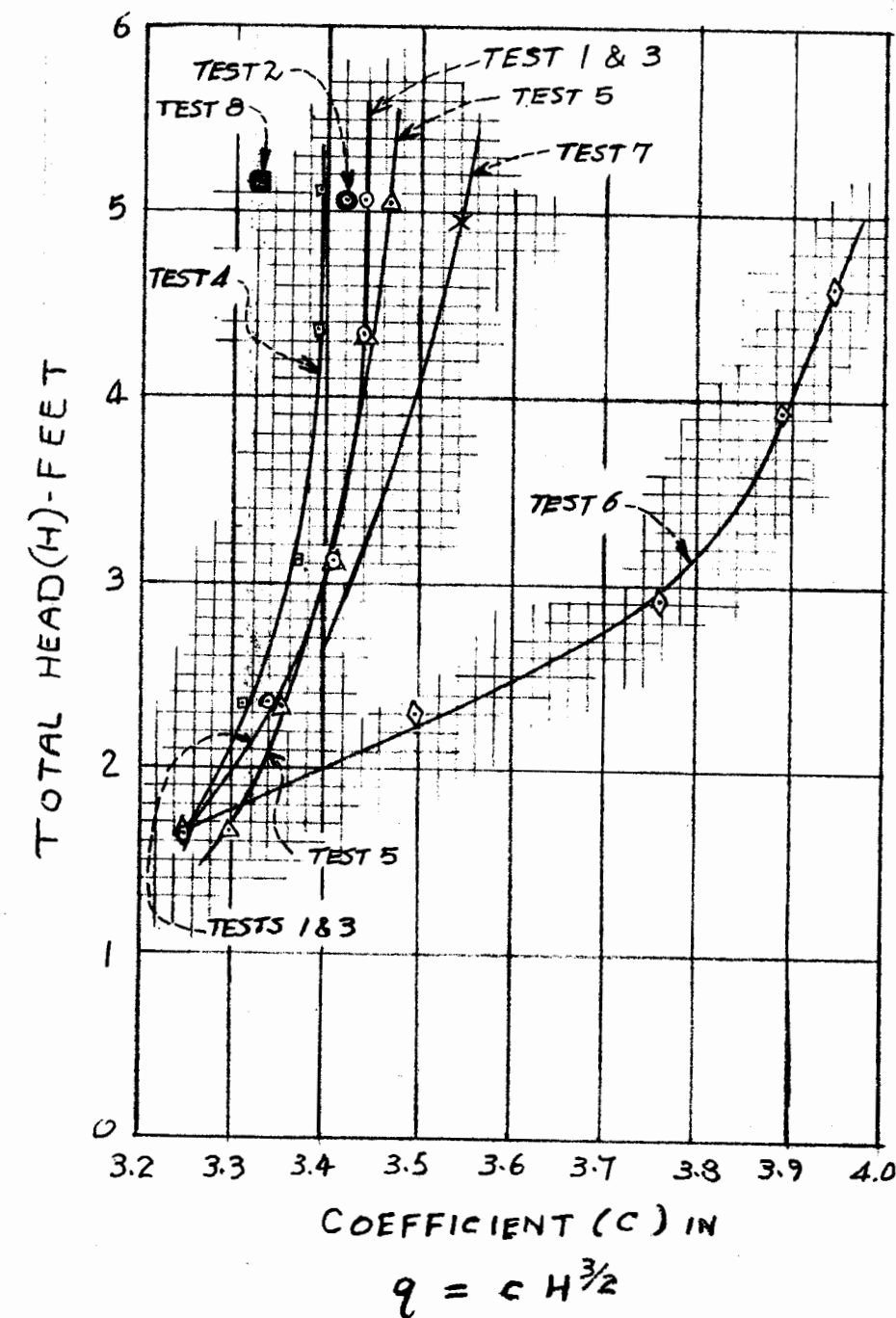
ROBLES DIVERSION DAM DISCHARGE AND DISCHARGE COEFFICIENT CURVES
