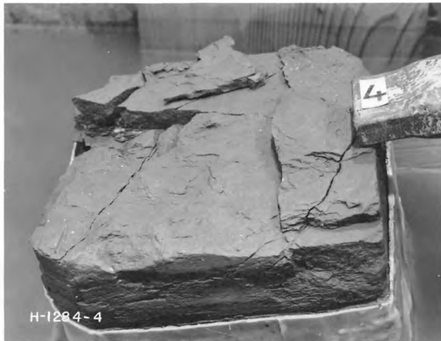
Sample after 1 hour test with flow velocity of 8 feet per second
