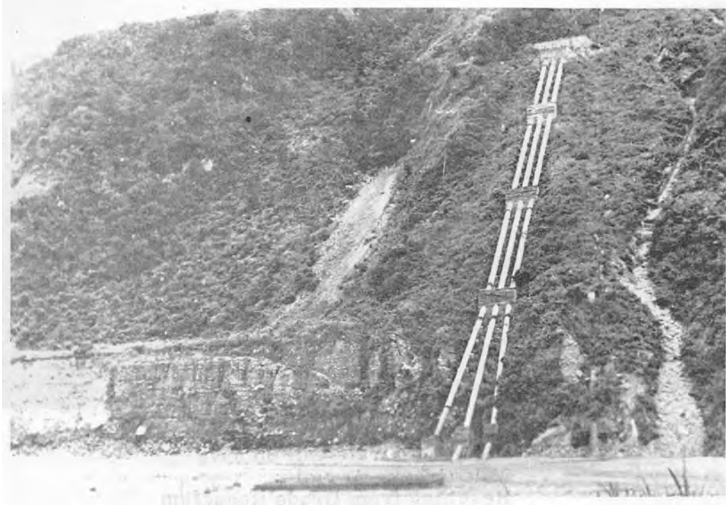
Figure 2. Roof of Powerplant Buried by Rise of Bed of the Mu Kwa River in Formosa
