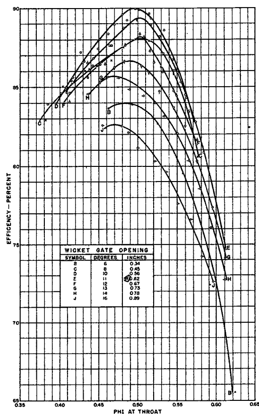
C-EFFICIENCY CURVES-MODIFIED SF-4 RUNNER
