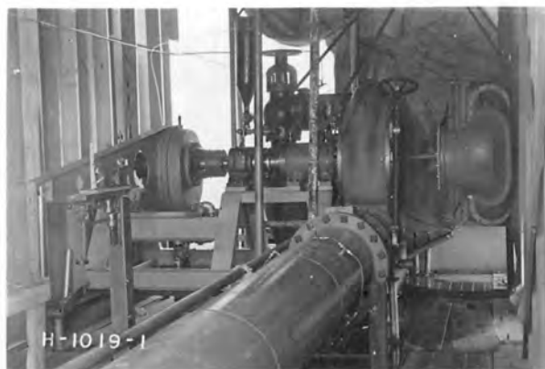
A. Turbine test arrangement. Water Brake dynamometer at left rear, penstock in foreground, and draft tube at right. Spool from turbine to draft tube not installed.
