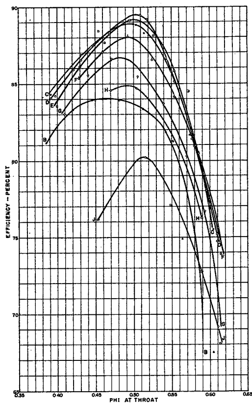
A-EFFICIENCY CURVES-ORIGINAL SF-4 RUNNER
