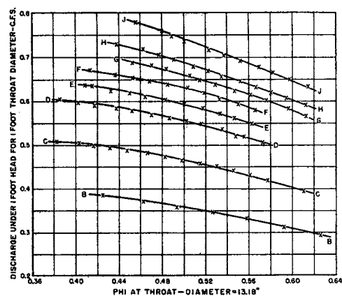
D— \Phi AT THROAT VS UNIT DISCHARGE
