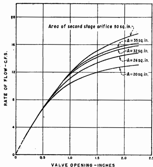
D - DISCHARGE THROUGH ABSORBER FOR 500 FOOT TOTAL HEAD
