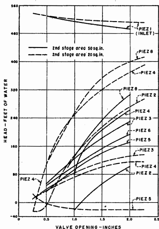
A - PRESSURES AT INLET AND WITHIN ENERGY ABSORBER
