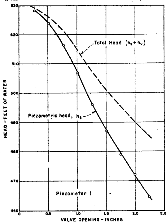
A - HEAD AT INLET TO BY-PASS VALVE
