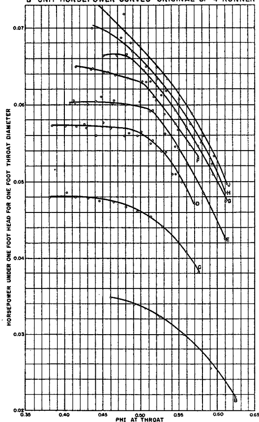
D-UNIT HORSEPOWER CURVES-MODIFIED SF-4 RUNNER
