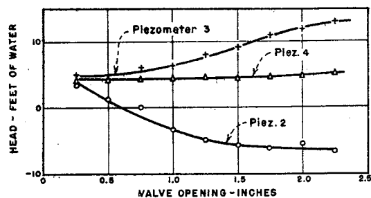
B - PRESSURES IN ENERGY ABSORBER
