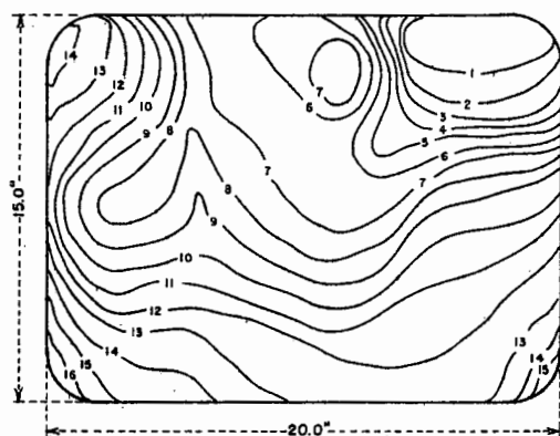
C - VELOCITY DISTRIBUTION AT OUTLET OF DRAFT TUBE. VIEW LOOKING DOWNSTREAM ( Q=12.68 cfs, valve opening 1\frac{1}{4} inches. No air admitted at third stage.)
