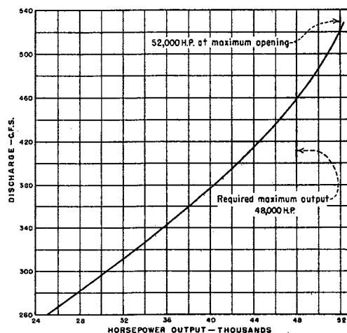
E—TOTAL HORSEPOWER VS TOTAL DISCHARGE
