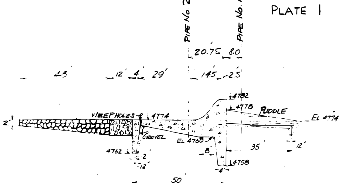
SECTIONAL VIEW SCALE HOR. 1"=30' VERT. 1"=20'
