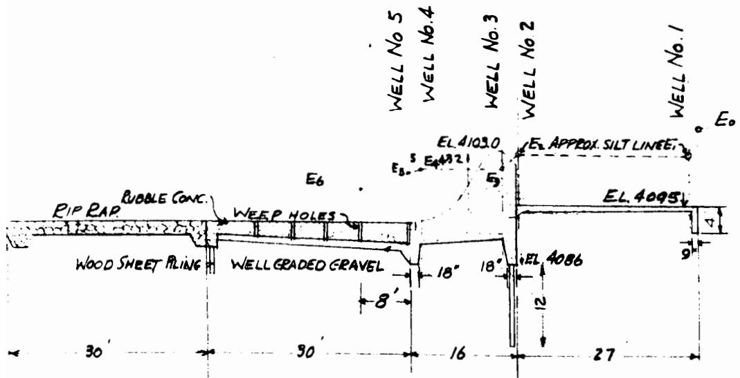
SECTION THRU SPILLWAY
