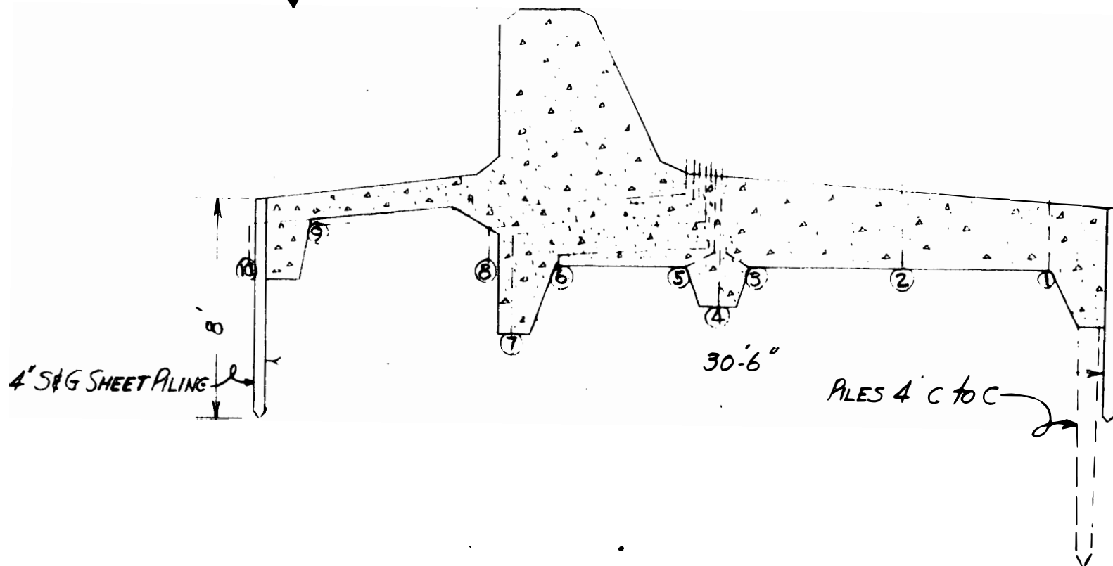
ISLAND PARK DAM SCALE: 1" = 5'
