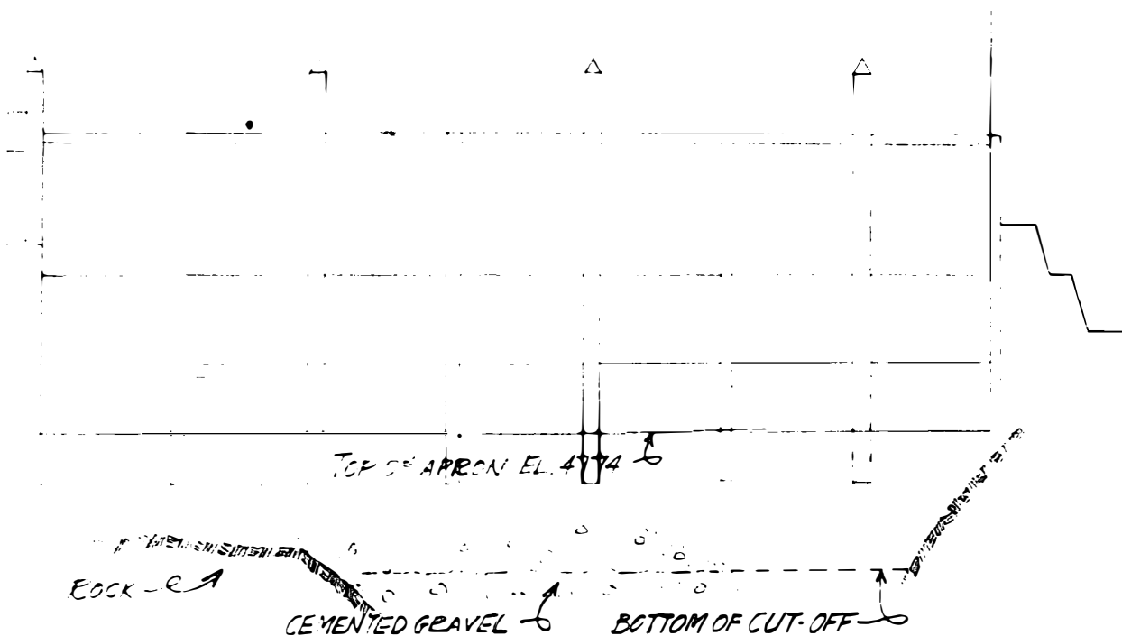
RIVER SECTION LOOKING UPSTREAM SCALE HOR 1"=10', VERT 1"=20'
