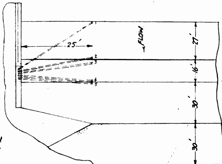
PARTIAL PLAN
