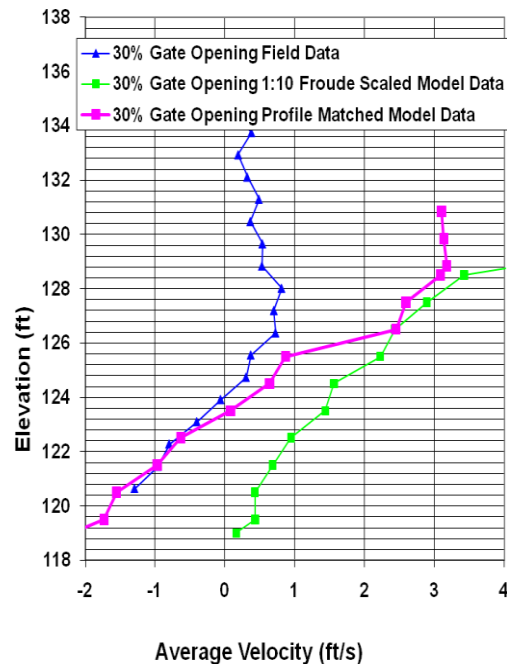
Figure 9. Vertical profiles of basin exit velocities compared at 30% gate opening for 1:10 scale model, profile matched model, and prototype.
