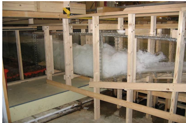
Figure 2. Choke Canyon stilling basin 1:10 scale model operating at 50% gate opening.
