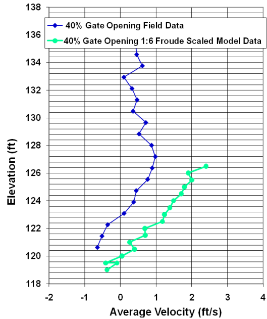
Figure 15. Vertical profiles of basin exit velocities compared at 40% gate opening for 1:6 scale model and prototype.
