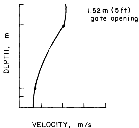
Figure 22.—Velocity profiles of existing and modified configurations. Yellowtail Afterbay Dam.
