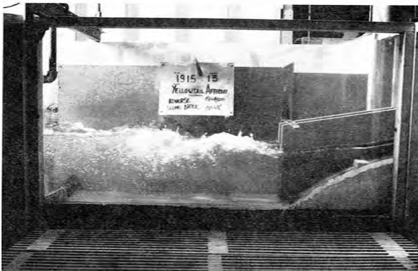
Figure 14.—Model operating with flow deflector configuration. Gate opening = 2.44 m and Q = 127 \text{ m}^3/\text{s} . (8 ft & 4500 \text{ft}^3/\text{s} ). Yellowtail Afterbay Dam.
