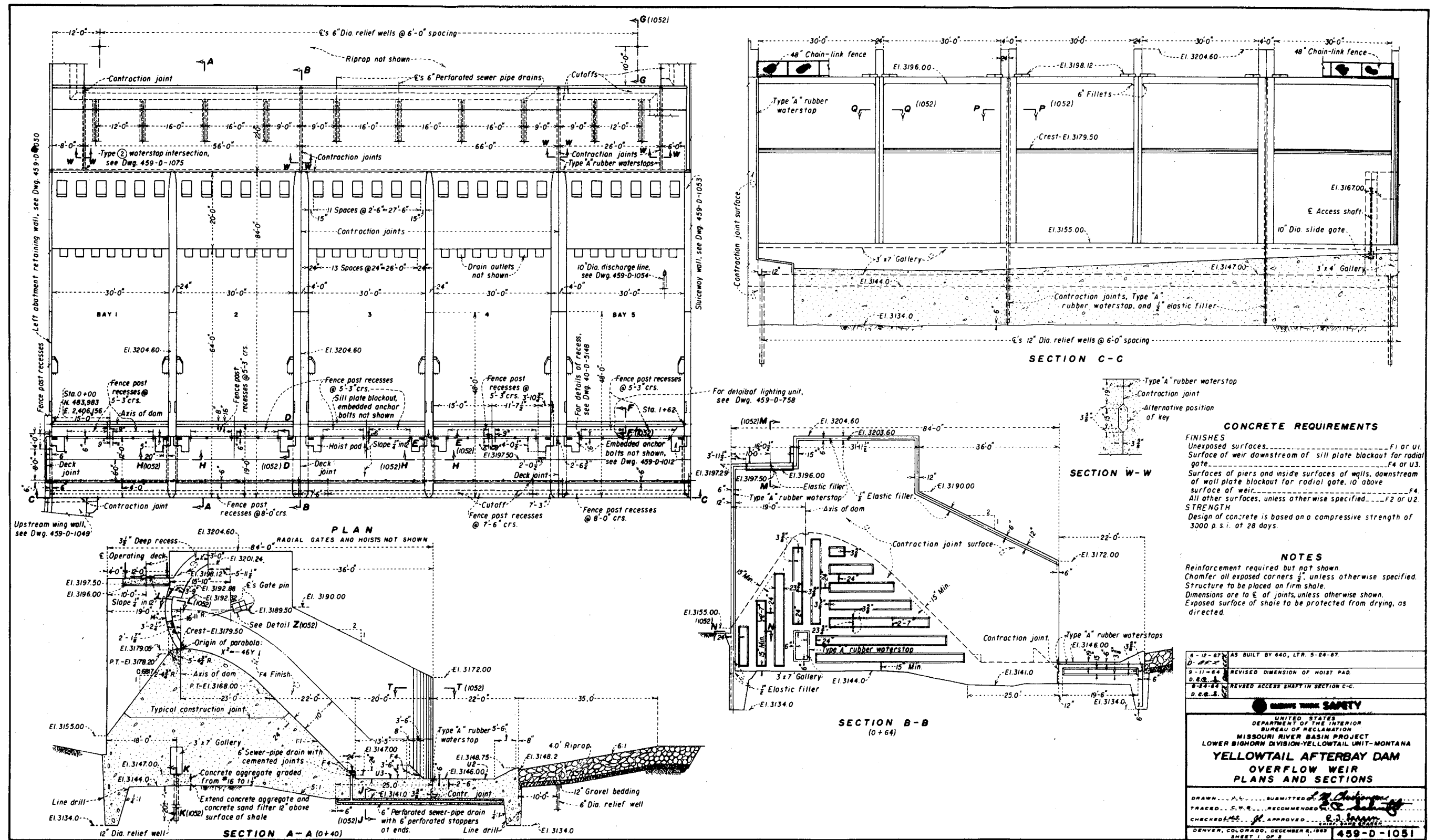
Figure 2.—Spillway overflow weir plan and sections.
