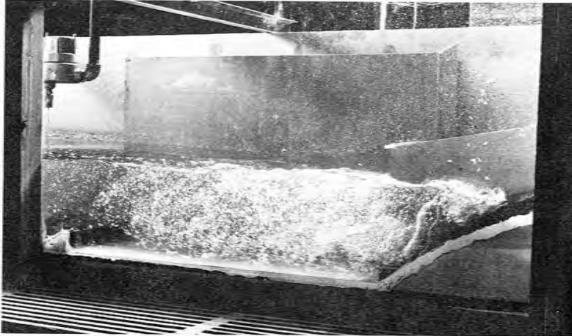
a. Existing configuration. P801-D-79773
