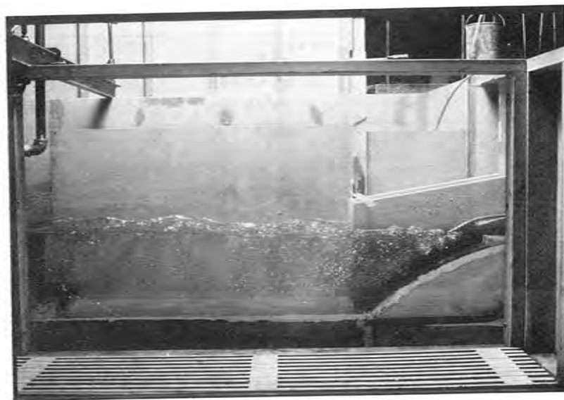
Figure 11.—Second modification—deflectors EL 962.25 m (3157.0 ft). Gate opening = 2.44 m and Q = 106 \text{ m}^3/\text{s} (8 ft & 3750 \text{ft}^3/\text{s} ). Yellowtail Afterbay Dam. P801-D-79766
