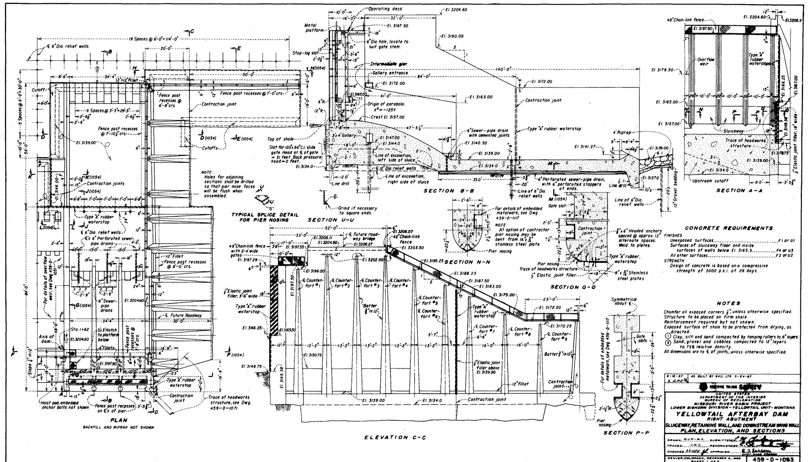
Figure 3.—Sluiceway plan and sections.
