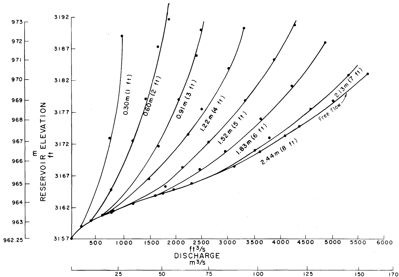
Figure 8.—Sluiceway discharge curve. Yellowtail Afterbay Dam.
