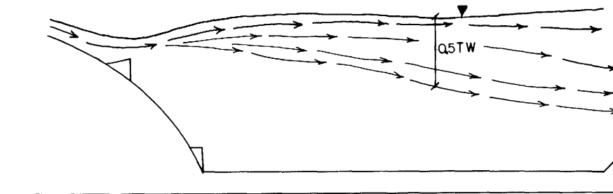
Figure 17.—Sluiceway jet profile, existing configuration. Yellowtail Afterbay Dam.
