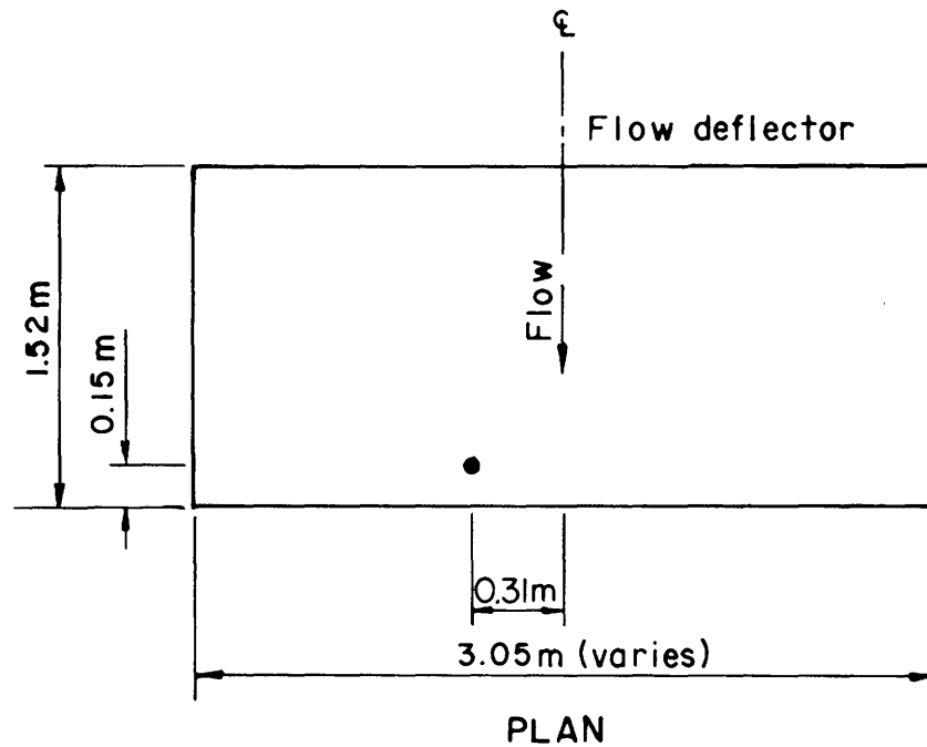
Figure 20.—Piezometer location on flow deflector. Yellowtail Afterbay Dam.
