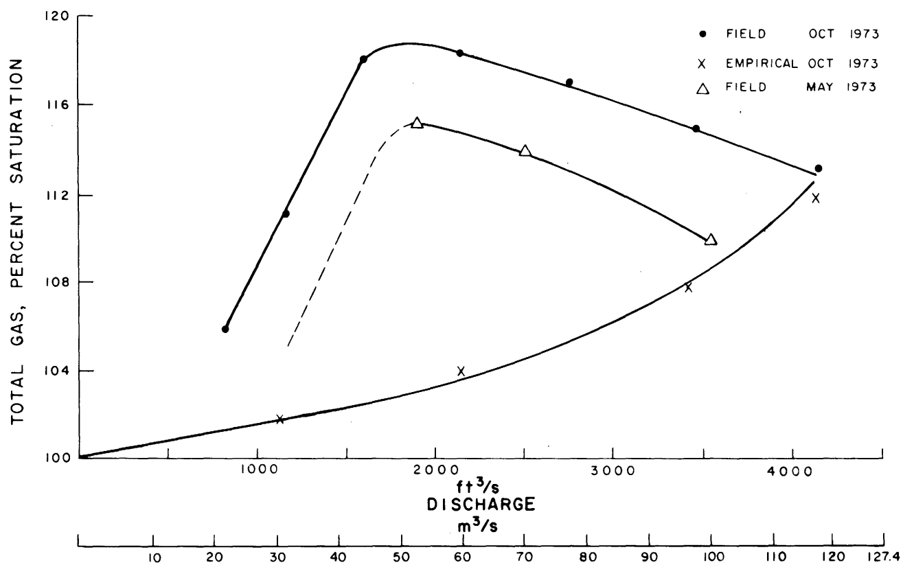
Figure 9.—Total gas saturation versus sluiceway discharge. Yellowtail Afterbay Dam.
