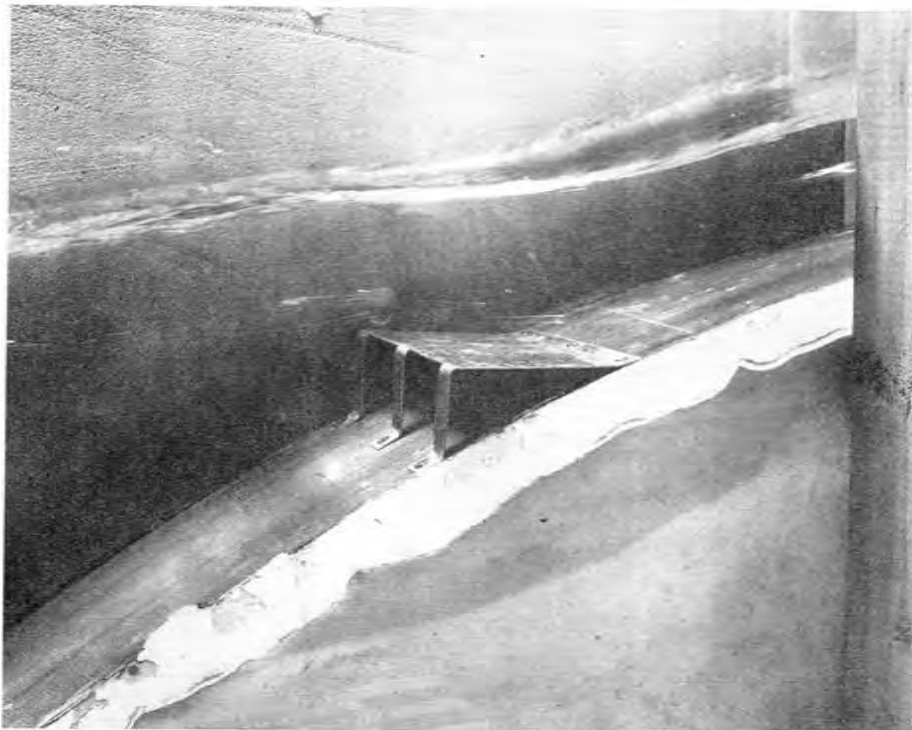
Figure 21.—Structural steel flow deflector installed in hydraulic model. Yellowtail Afterbay Dam. P801-D-79777
