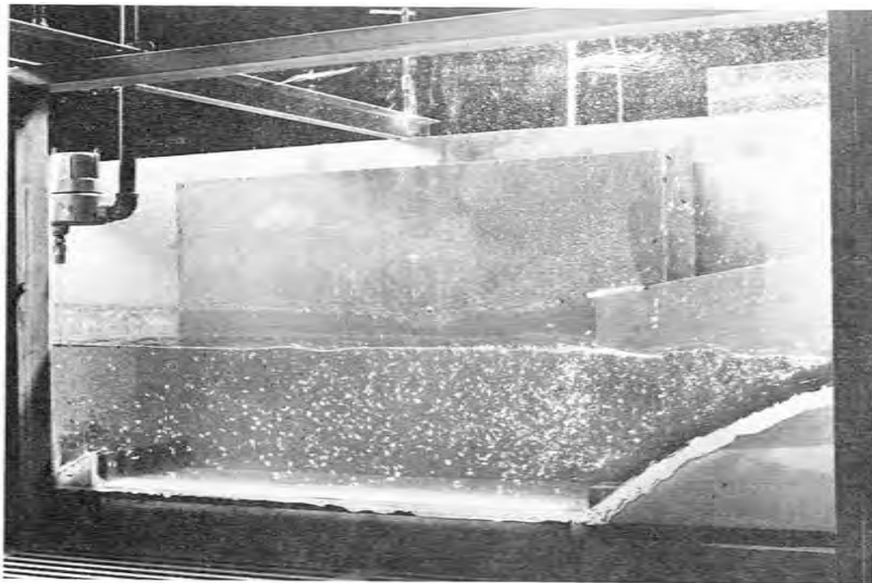
a. Existing configuration. P801-D-79767
