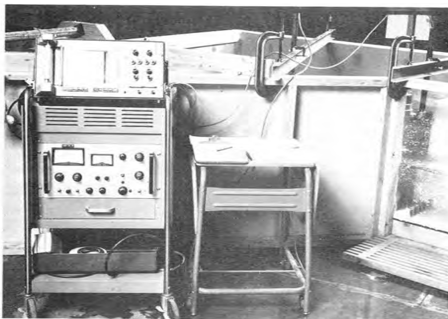
Figure 24.—Recorder for wave measurements. P801-D-79779
