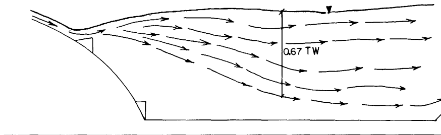
Figure 18.—Modified sluiceway jet profile, Q = 57 \text{ m}^3/\text{s} (2000 \text{ft}^3/\text{s} ). Flow deflector recommended design. Yellowtail Afterbay Dam.
