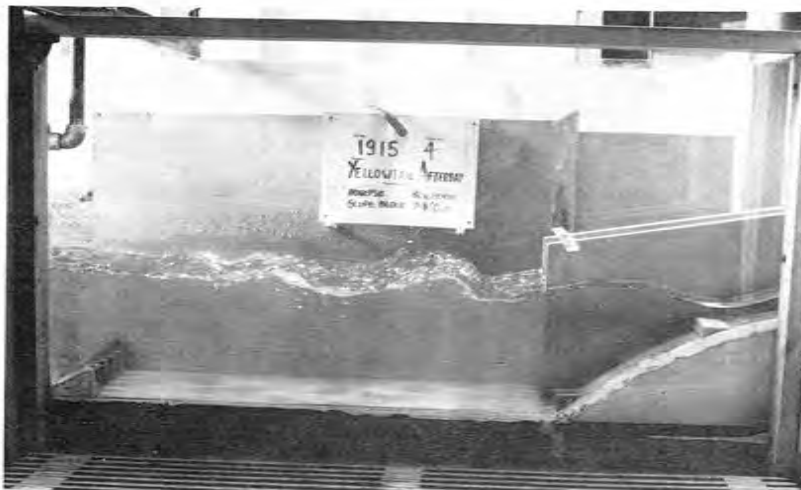
Figure 12.—Model operating with flow deflector configuration. Gate opening = 2.44 m and Q = 57 \text{ m}^3/\text{s} . (8 ft & 2000 \text{ft}^3/\text{s} ). Yellowtail Afterbay Dam.
