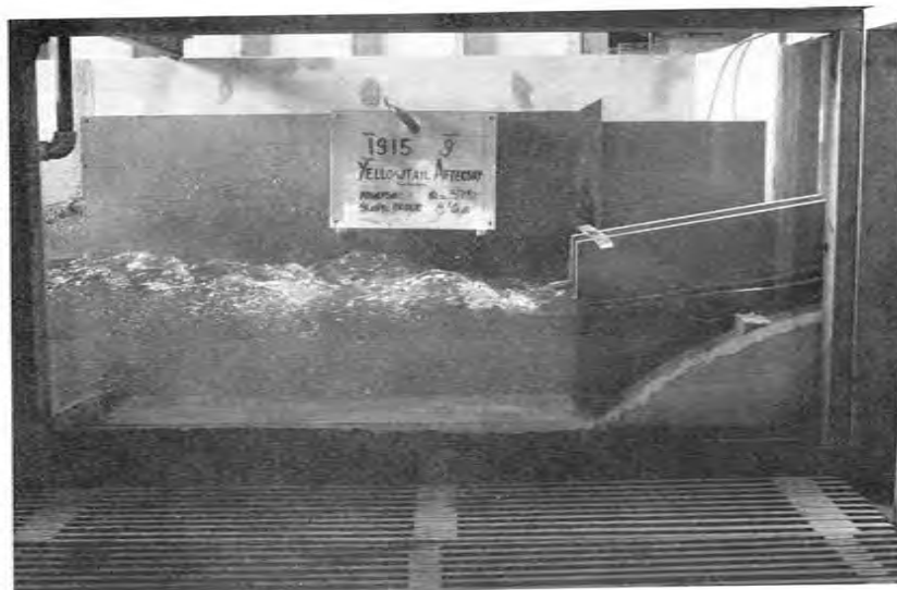
Figure 13.—Model operating with flow deflector configuration. Gate opening = 2.44 m and Q = 106 \text{ m}^3/\text{s} . (8 ft & 3750 \text{ft}^3/\text{s} ). Yellowtail Afterbay Dam.
