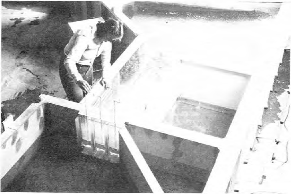
Figure 4.—Yellow Afterbay Dam sluiceway model in operation. Scale 1:24. P801-D-79761
