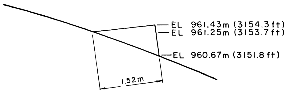
DETAIL A
