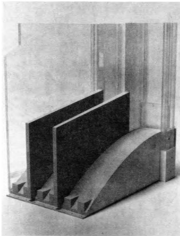
Figure 7.—Model sluiceway crest, gates, and piers. Yellowtail Afterbay Dam. P801-D-79764
