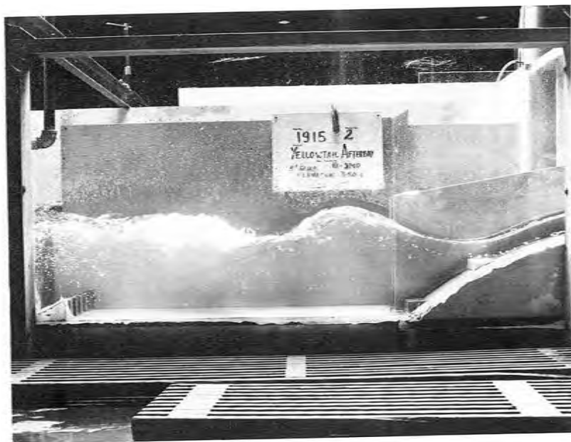
Figure 10.—First modification—deflectors EL 960.30 m (3150.6 ft). Gate opening = 2.44 m and Q = 106 \text{ m}^3/\text{s} (8 ft & 3750 \text{ft}^3/\text{s} ). Yellowtail Afterbay Dam. P801-D-79765
