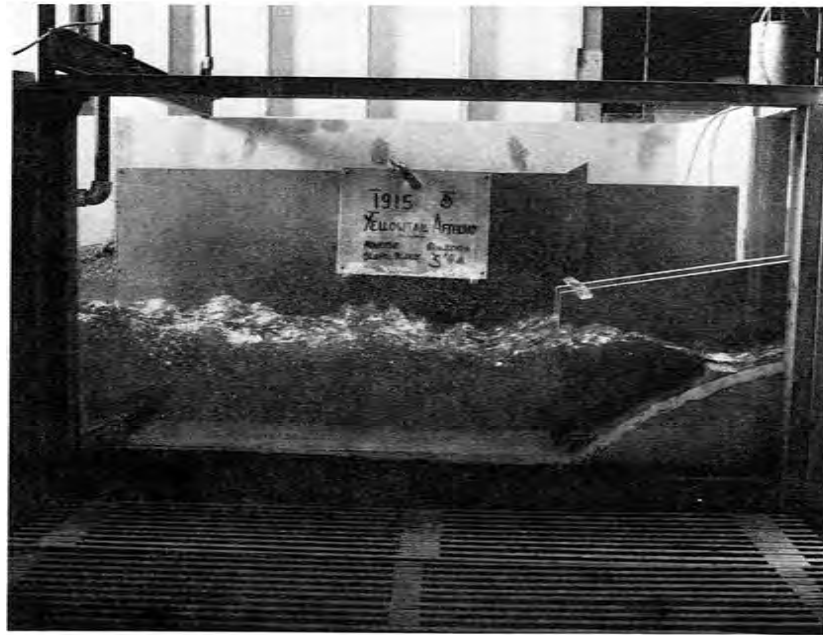
Figure 16.—Most frequent operating condition with flow deflectors installed. Gate opening = 0.91 m and Q = 57 \text{ m}^3/\text{s} (3 ft and 2000 \text{ft}^3/\text{s} ). Yellowtail Afterbay Dam. P801-D-79976
