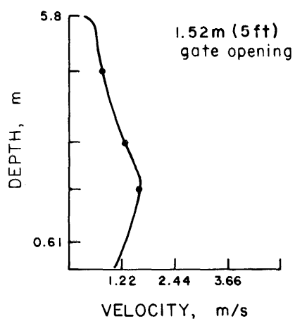
Figure 22.—Velocity profiles of existing and modified configurations. Yellowtail Afterbay Dam.
