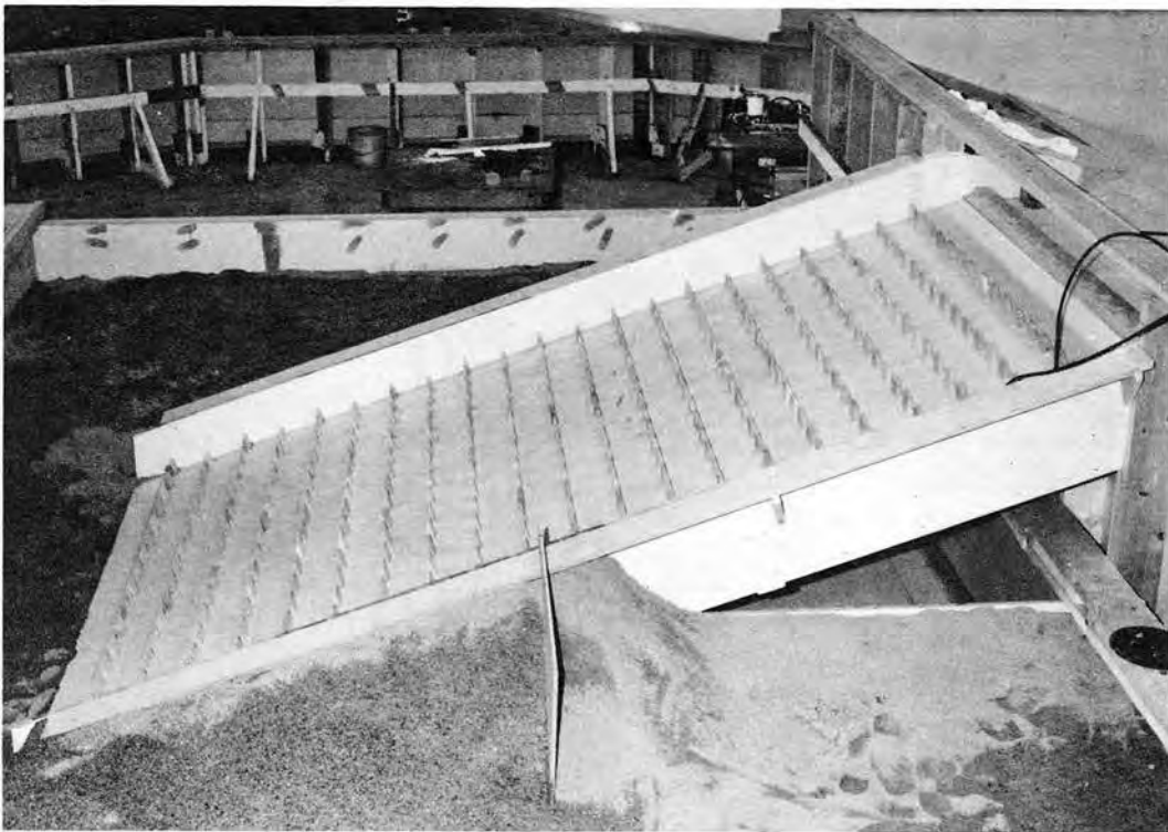
Figure 3.—Model during construction. Photo P801-D-79010
