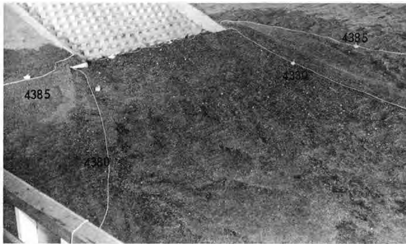
a) Discharge 5000 ft 3 /s. Photo P801-D-79015
