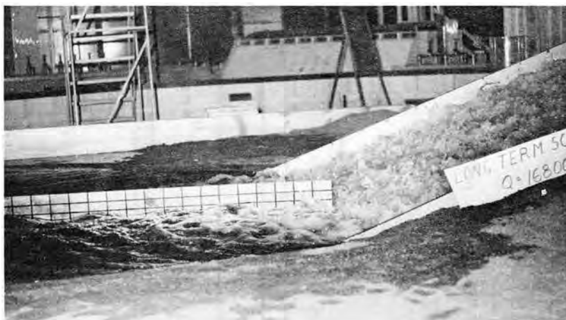
b) Discharge 16 800 ft 3 /s, top of plate at El. 4395. Photo P801-D-79025
