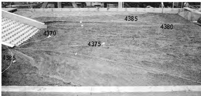
b) Discharge 16 800 ft 3 /s. Photo P801-D-79016
