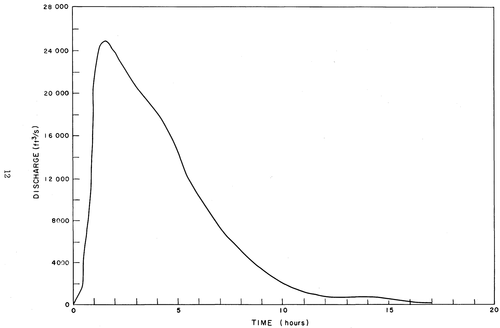
Figure 1.—Outflow hydrograph.
