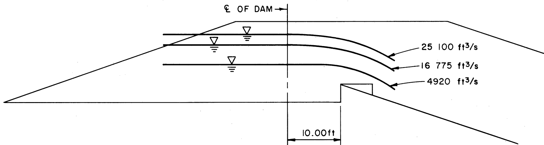
Figure 15.—Water surface profiles along centerline of the spillway.
