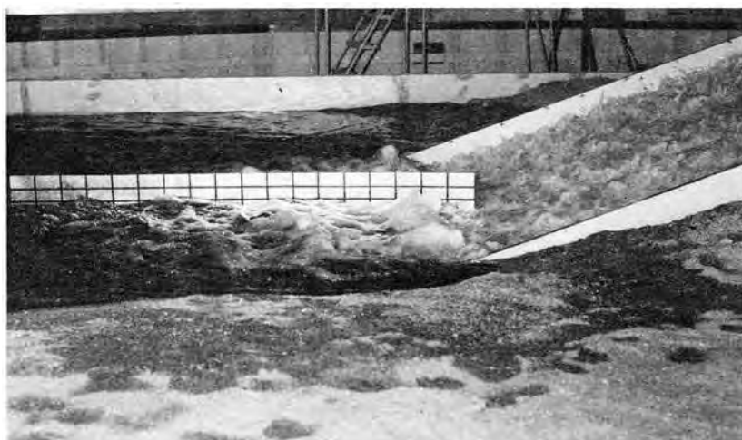
Figure 13.—Stilling basin water surface.
