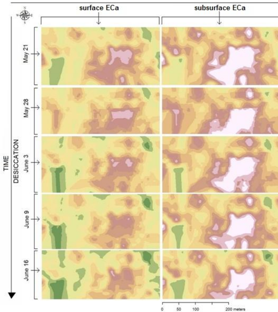
Figure 6.8 Temporal Study at MS 3b in 2008 demonstrating the effects of soil dessication on EM-38 signal response. Weekly Surveys conducted from May 21, 2008 thru June 16, 2008 following exact transects for each survey. Surface ECa (left column) represent the EM-38 Horizontal signal, subsurface ECa (right column) represents the EM-38 Vertical signal.
