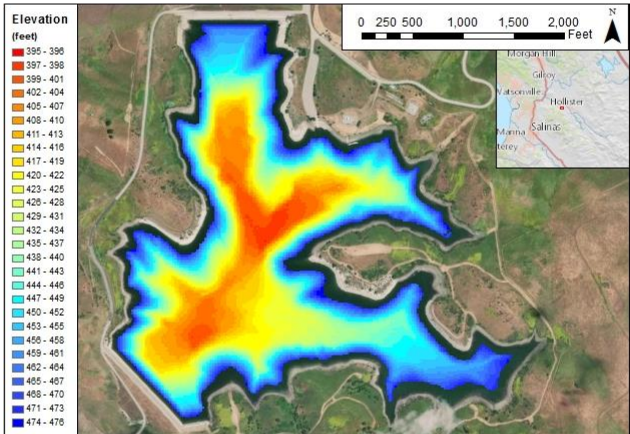
Figure 3. San Justo Reservoir bathymetric chart from 2017 survey.
