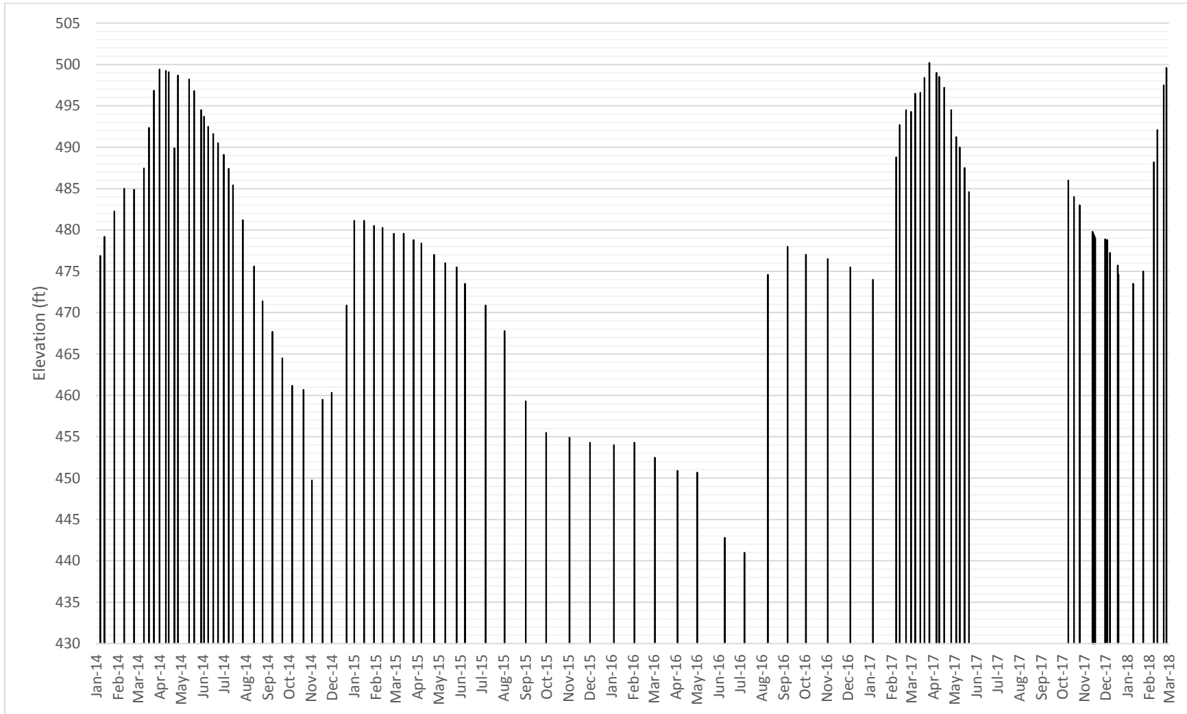
Figure B 1. San Justo Reservoir, available historic elevation data (Jan. 2014 - Mar. 2018).
