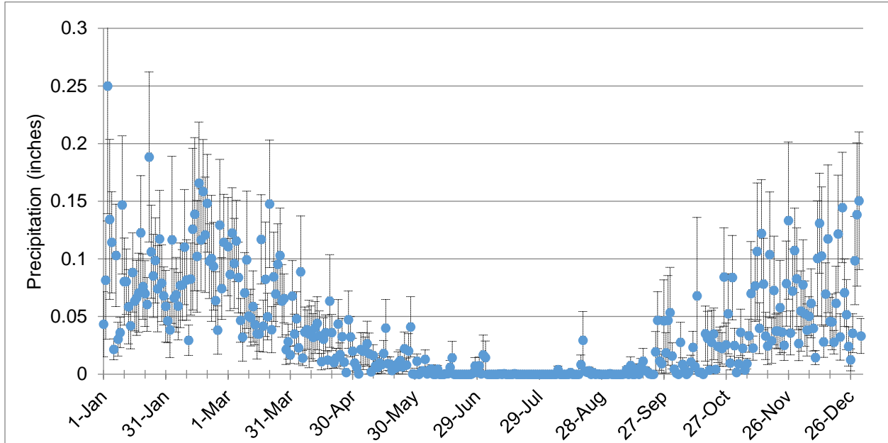
Figure C 1. 35 year daily precipitation means and standard deviations, Hollister weather station.
