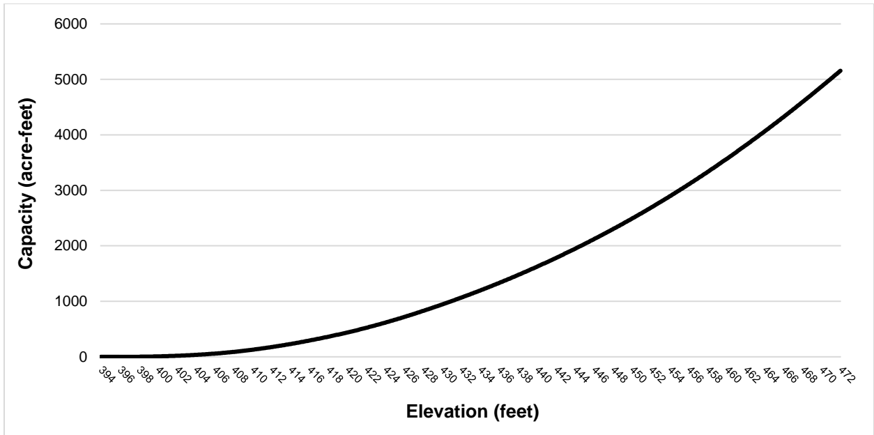
Figure 2. San Justo Reservoir capacity by elevation from 2017 bathymetry.
