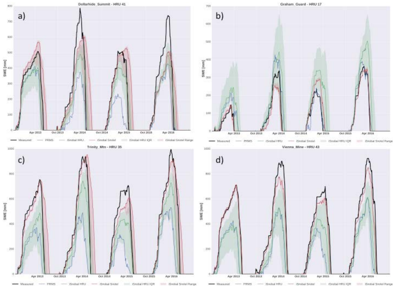
Figure 4. SWE comparison for Dollarhide Summit, Graham Guard Station, Trinity Mountain, and Vienna Mine. Black line is SNOTEL measurement, blue is PRMS, red is 10 iSnoPal pixels around the measurement, and green is iSnoPal median and IQR within the HRU.
