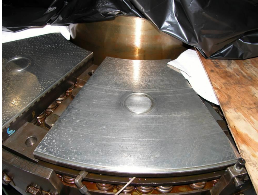
Photo 9.—Spring loaded thrust shoe bearing.
