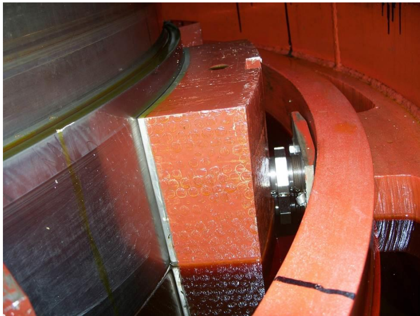
Photo 13.—Adjustable segmented shoe bearing.
