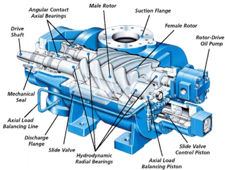
Figure 11. Cutaway view of a twin-screw reciprocating compressor.
