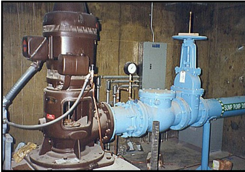
Photograph 2. Sump pumping unit discharge assembly.
