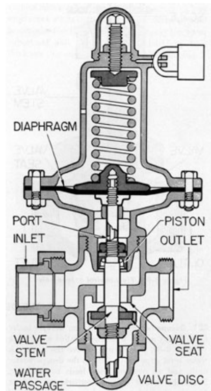
Figure 8. Pressure reducing valve components.
