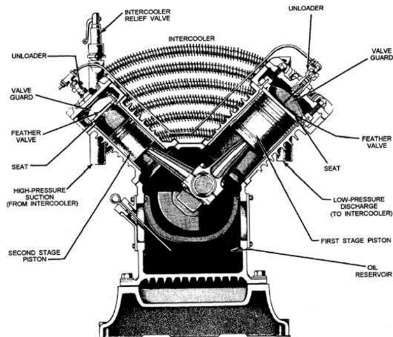
Figure 10. Two-stage reciprocating compressor.
