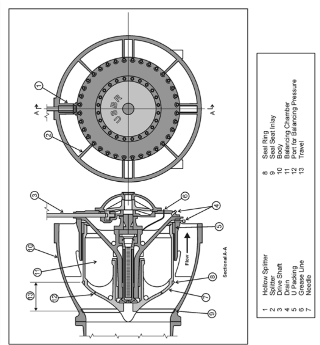
Figure 29. Hollow jet valve (mechanically operated)
