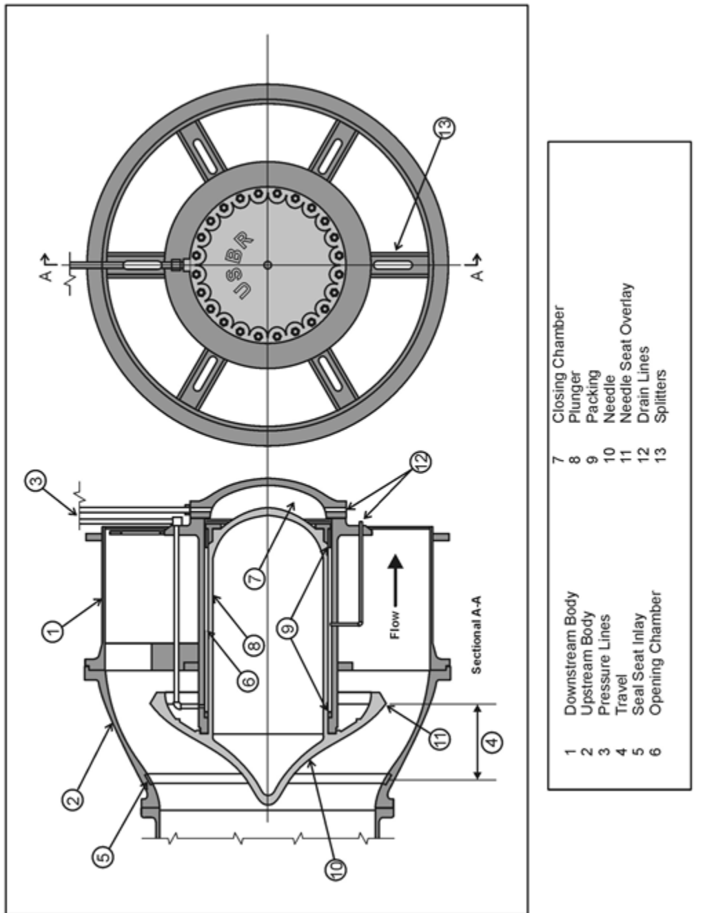
Figure 30. Hollow jet valve (hydraulically operated)
