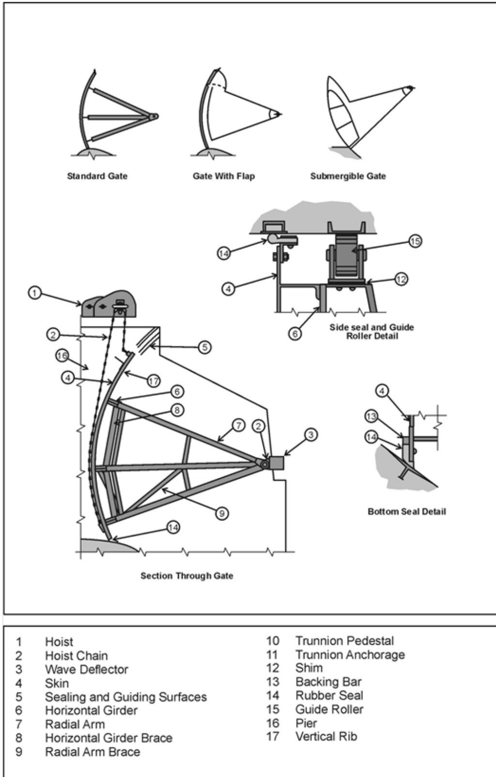
Figure 18. Radial Gates
