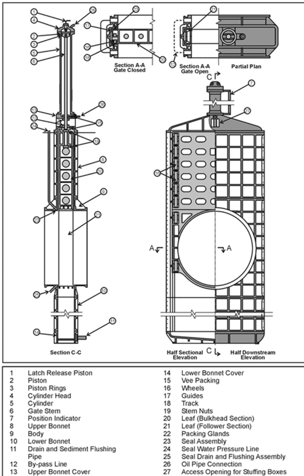
Figure 24. Ring seal gate (mechanically operated)
