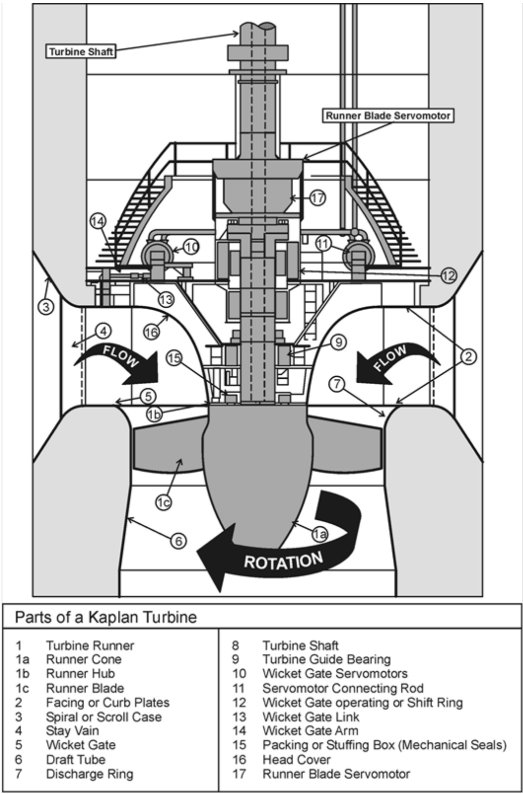
Figure 2. Kaplan turbine
