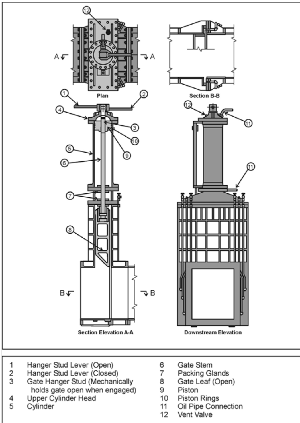
Figure 19. Slide gate
