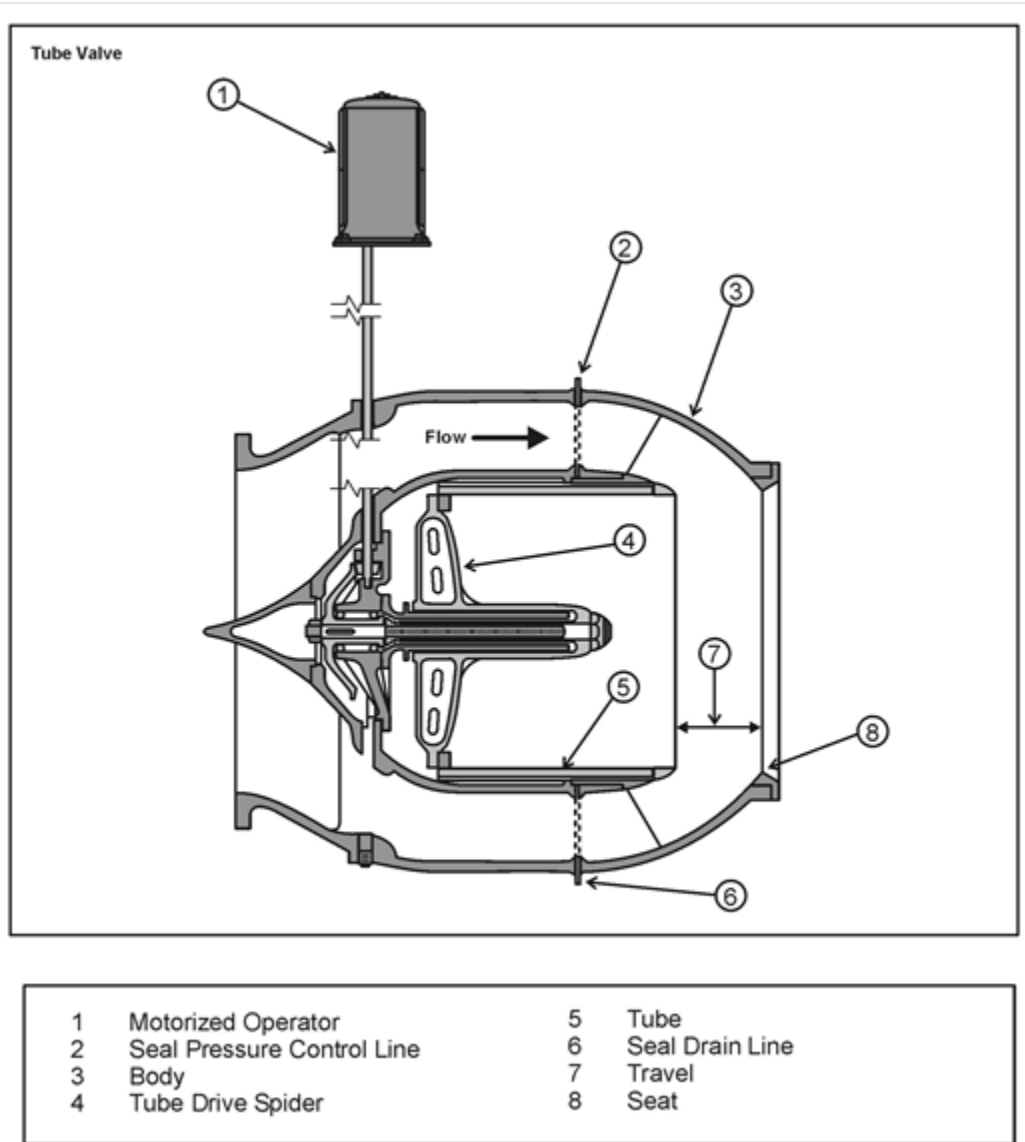
Figure 28. Tube Valve
