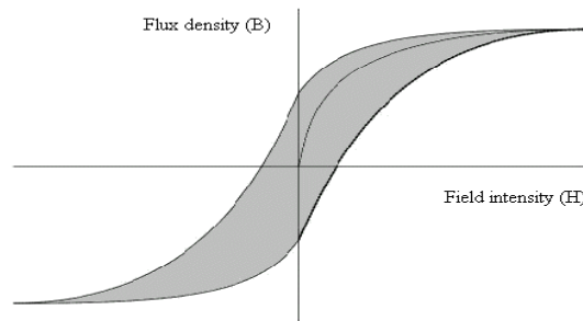
Figure E-1. Curves plotted showing magnetic flux density as a function of magnetizing force.
