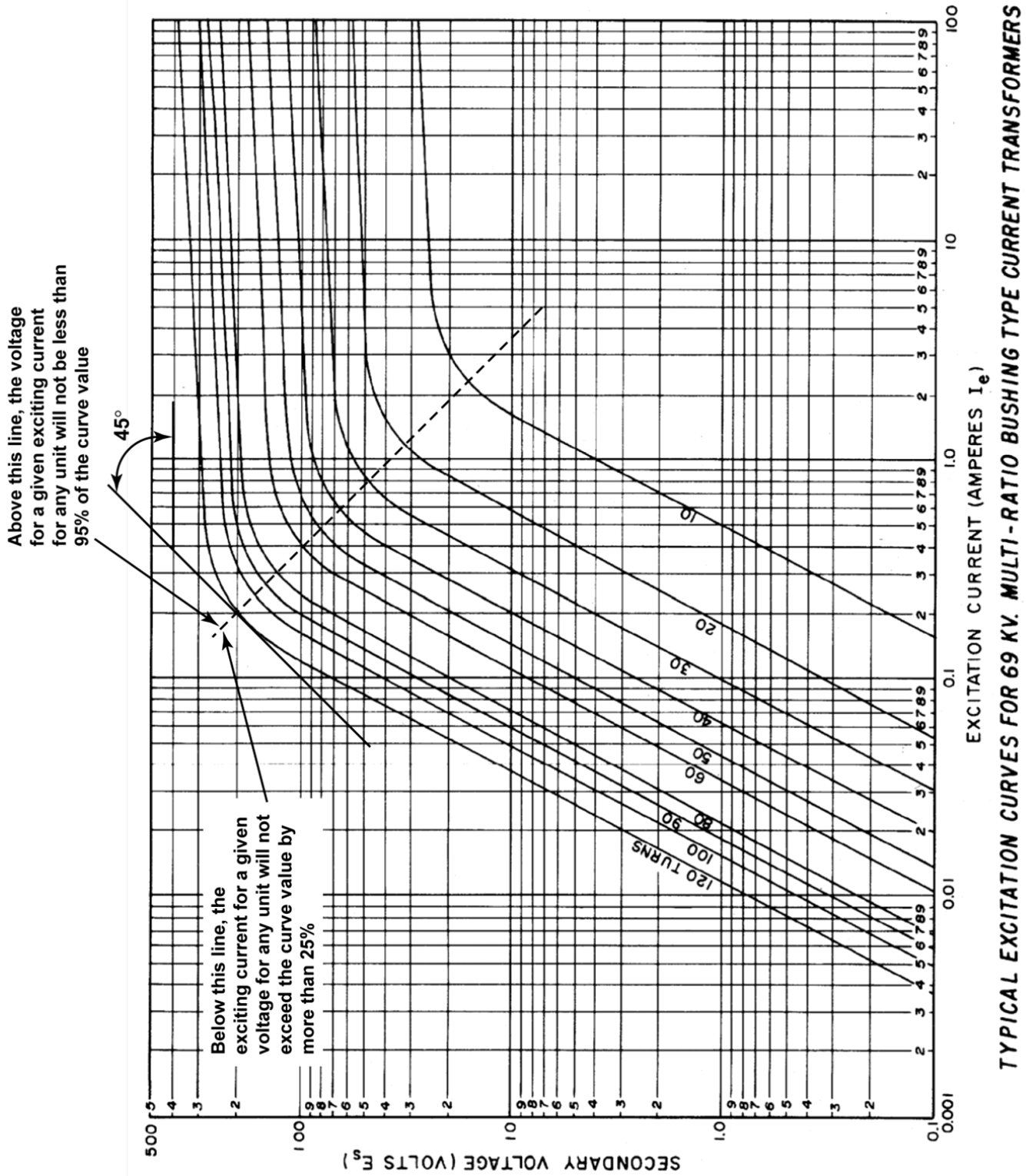
Figure E-3. Typical excitation curve – C200 CT.
