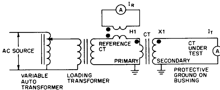
Figure E-7. Offline current method for manually testing CTs.
