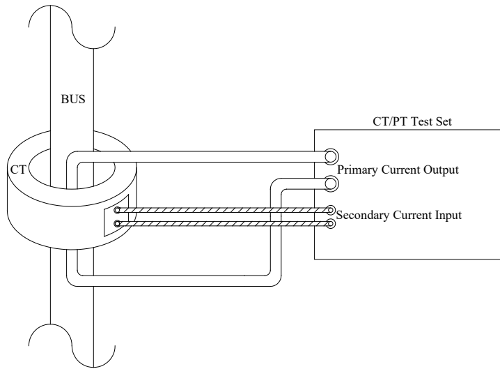
Figure E-6. Offline current method for testing CTs with test set.
