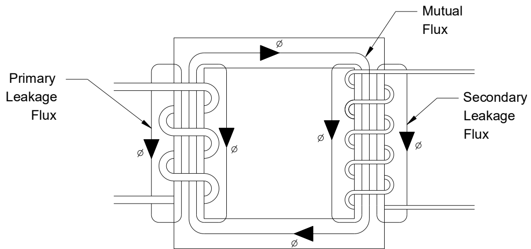
Figure C-2. Leakage flux.
