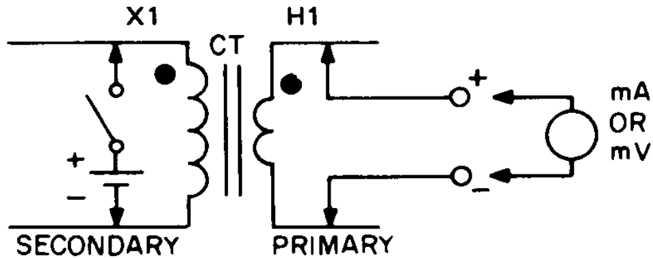
Figure E-8. DC voltage polarity test for CTs.
