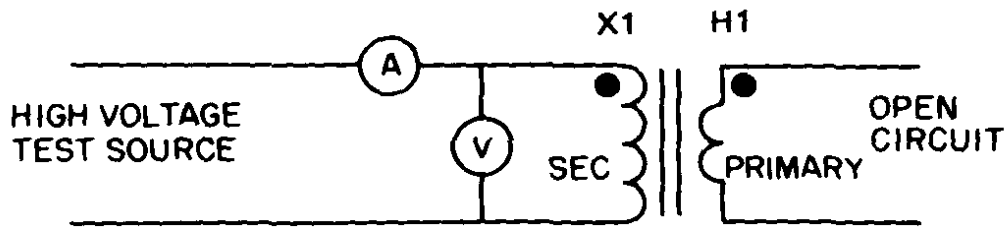
Figure E-4. CT excitation, voltage method to measure ratio, and demagnetizing test setup.
