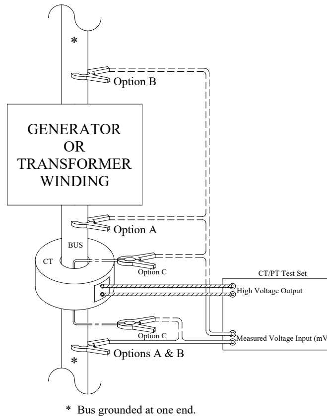
Figure E-5. Offline voltage method.
