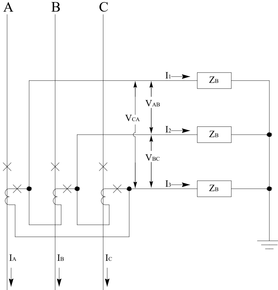
Figure D-2. Delta connected CTs.
