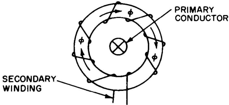
Figure C-1. Uniformly distributed secondary winding.
