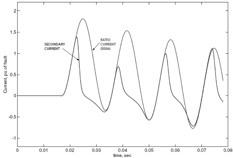
Figure E-2. Example of a 50:5 CT under fault current of 500 amperes (amps) (fully offset).
