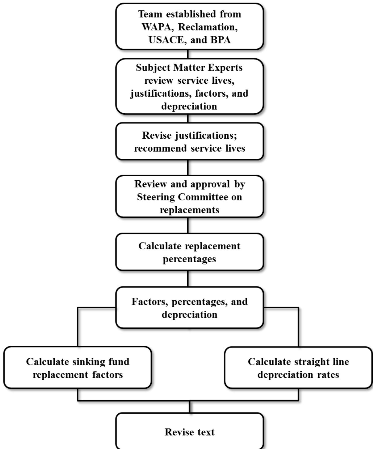
Figure 1. Study Methodology
